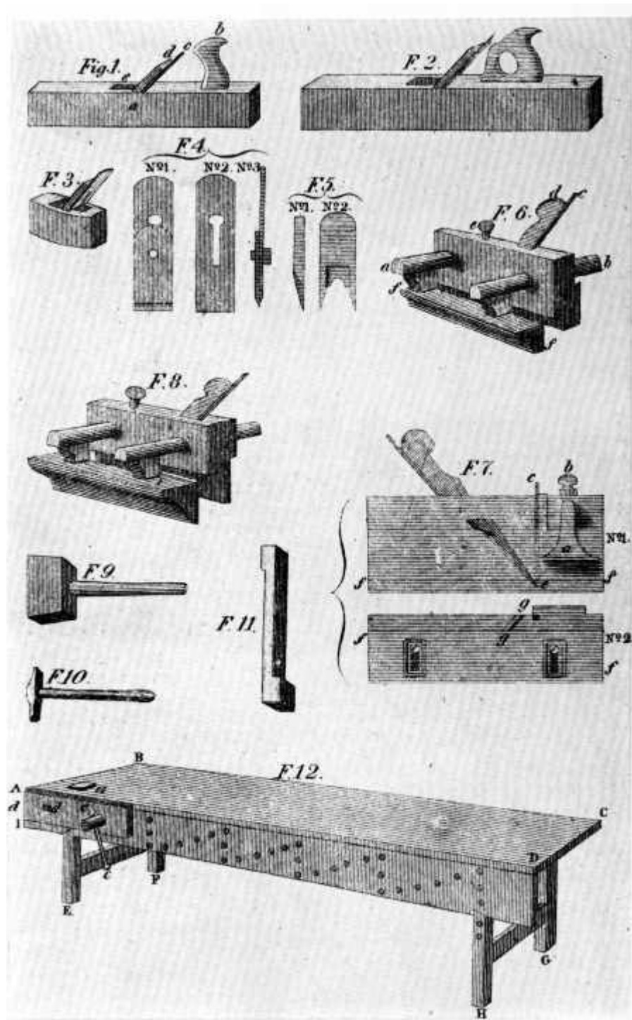
Figure 9.—1832: THE WORKBENCH DELINEATED BY NICHOLSON was little improved over Moxon's, although the planes—jack (1), trying plane (2), smoothing plane (3), sash fillister (7), and plow (8)—followed the form seen in Martin (fig. 7). The inception of this shape occurred in the shops of Sheffield toolmakers in the last half of the 18th century, and it persisted until replaced by metallic versions patented by American innovators during the last quarter of the 19th century. (Nicholson, The Mechanic's Companion . Smithsonian photo 56631.)
