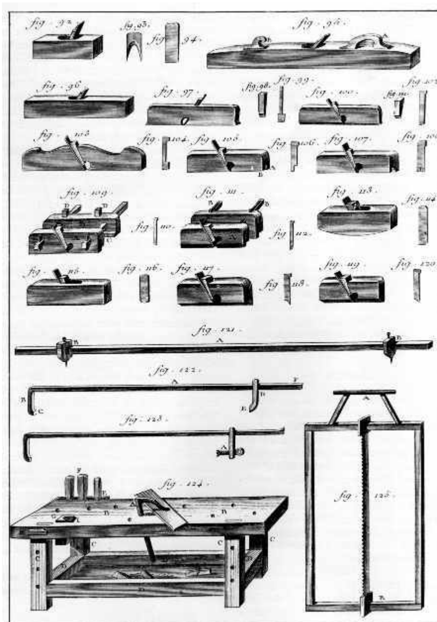
Figure 5.—1769:THE BENCH PLANES OF THE JOINER increased in number, but in appearance they remained much the same as those illustrated by Moxon. (Denis Diderot, Recueil de planches sur les science et les arts libéraux , Paris, 1769, vol. 7, "Menuiserie." Smithsonian photo 56630.)
