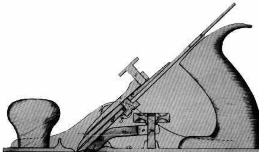
Figure 64.—1867: THE DRAWING accompanying B.A. Blandin's specification for an "Improvement in Bench Planes" retained only the familiarly shaped handle or tote of the traditional wood-bodied plane. This new shape rapidly became the standard form of the tool with later variations chiefly related to the adjustability of the plane-iron and sole. (Wash drawing from U.S. Patent Office, May 7, 1867, Record Group 241, the National Archives.)
