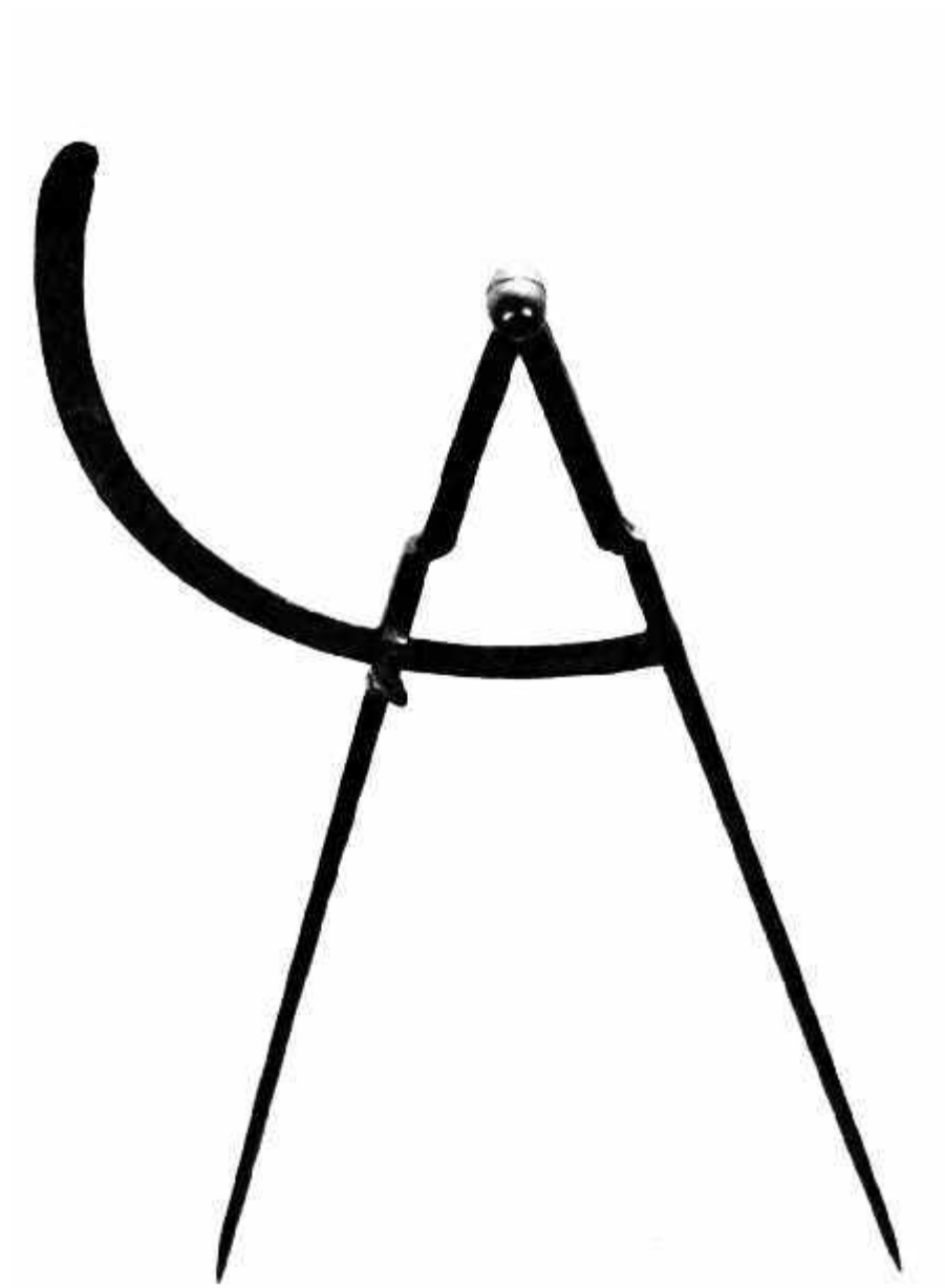
Figure 18.—18 TH CENTURY: Carpenter's dividers of English origin, undated. (Smithsonian photo 49792-B.)
