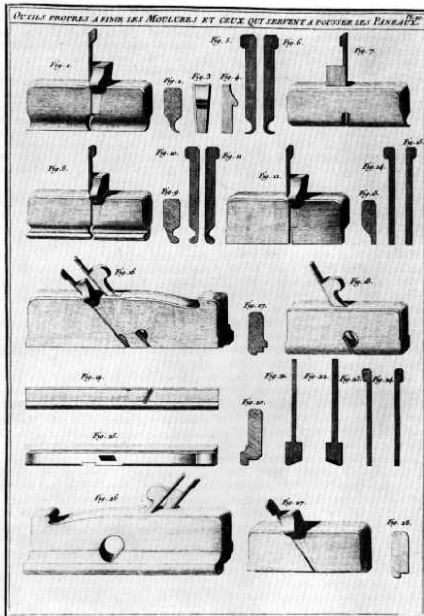
Figure 6.—1774:ANDRÉ ROUBO's L'Art du menuisier contains detailed plates and descriptions of the most specialized of woodworking planes: those used to cut panel moldings. The conformation of these tools was still distinctly in keeping with the Moxon type and suggests that, at least in Europe, no remarkable change had yet occurred in the shape of planes. (André-Jacob Roubo, L'Art du menuisier . Troisième partie, troisième section, l'art du menuisier ébéniste [Paris, 1774]. Smithsonian photo 49790-D.)
