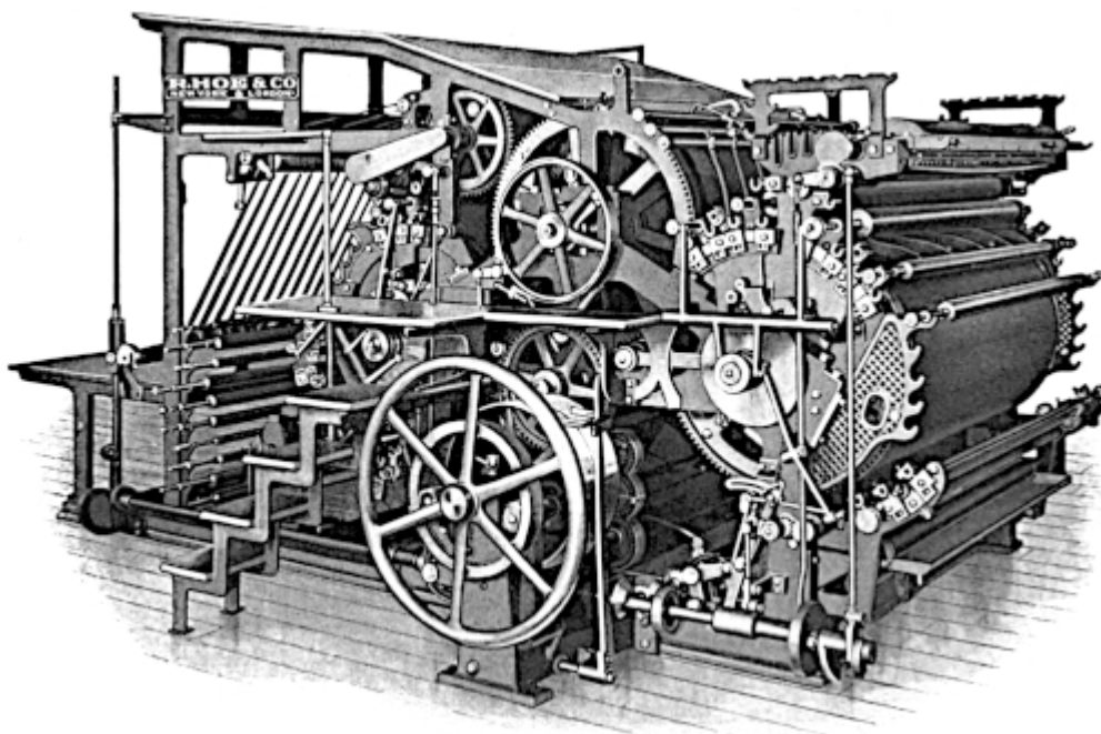
TWO-COLOR ROTARY ZINCOGRAPHIC OR ALUMINUM PRESS
