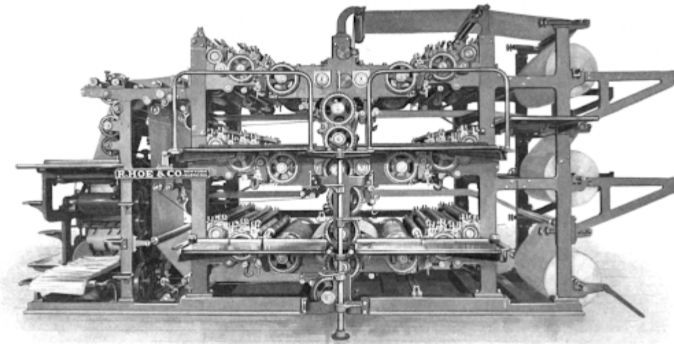
STRAIGHT-LINE PRESS
