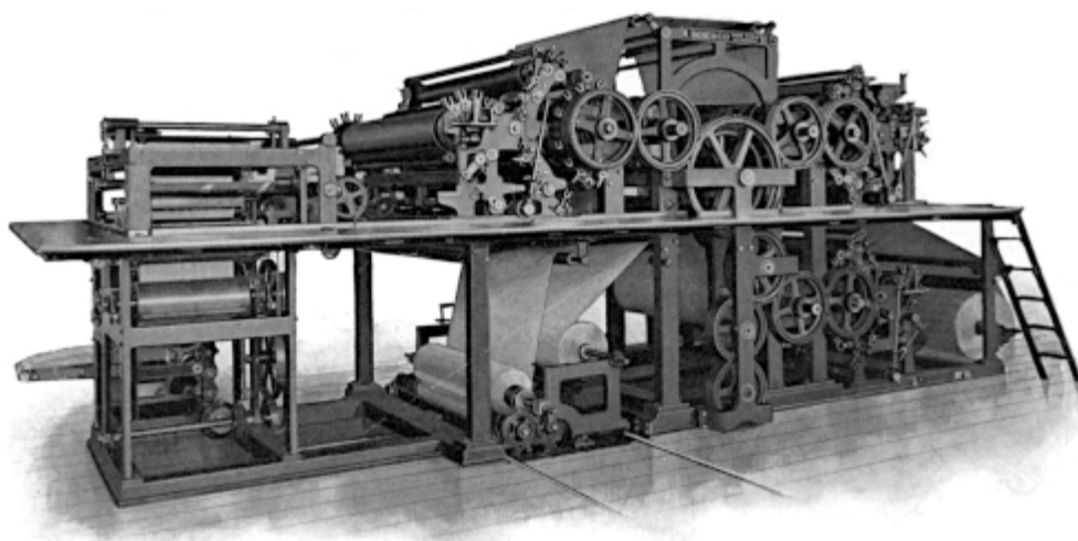
"COLLIER'S WEEKLY" PRESS
