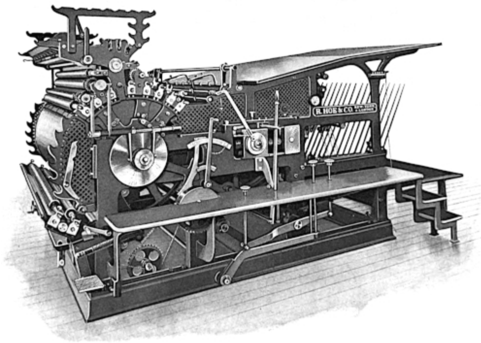
ROTARY ZINCOGRAPHIC OR ALUMINUM PRESS
