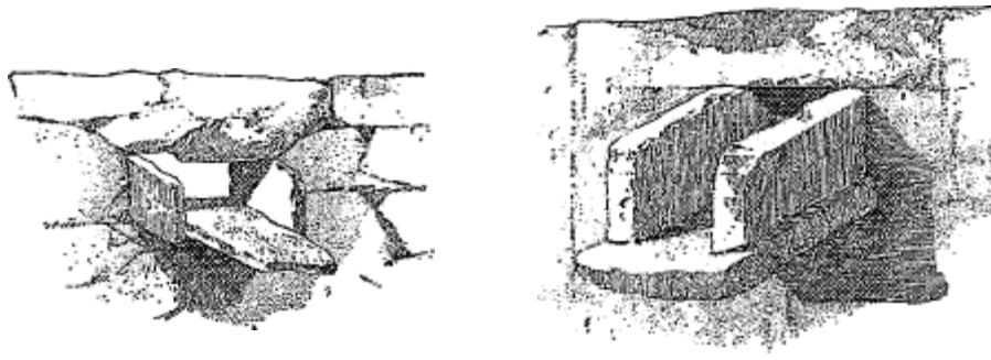
FIG. 40. Trough roof drains of stone.
