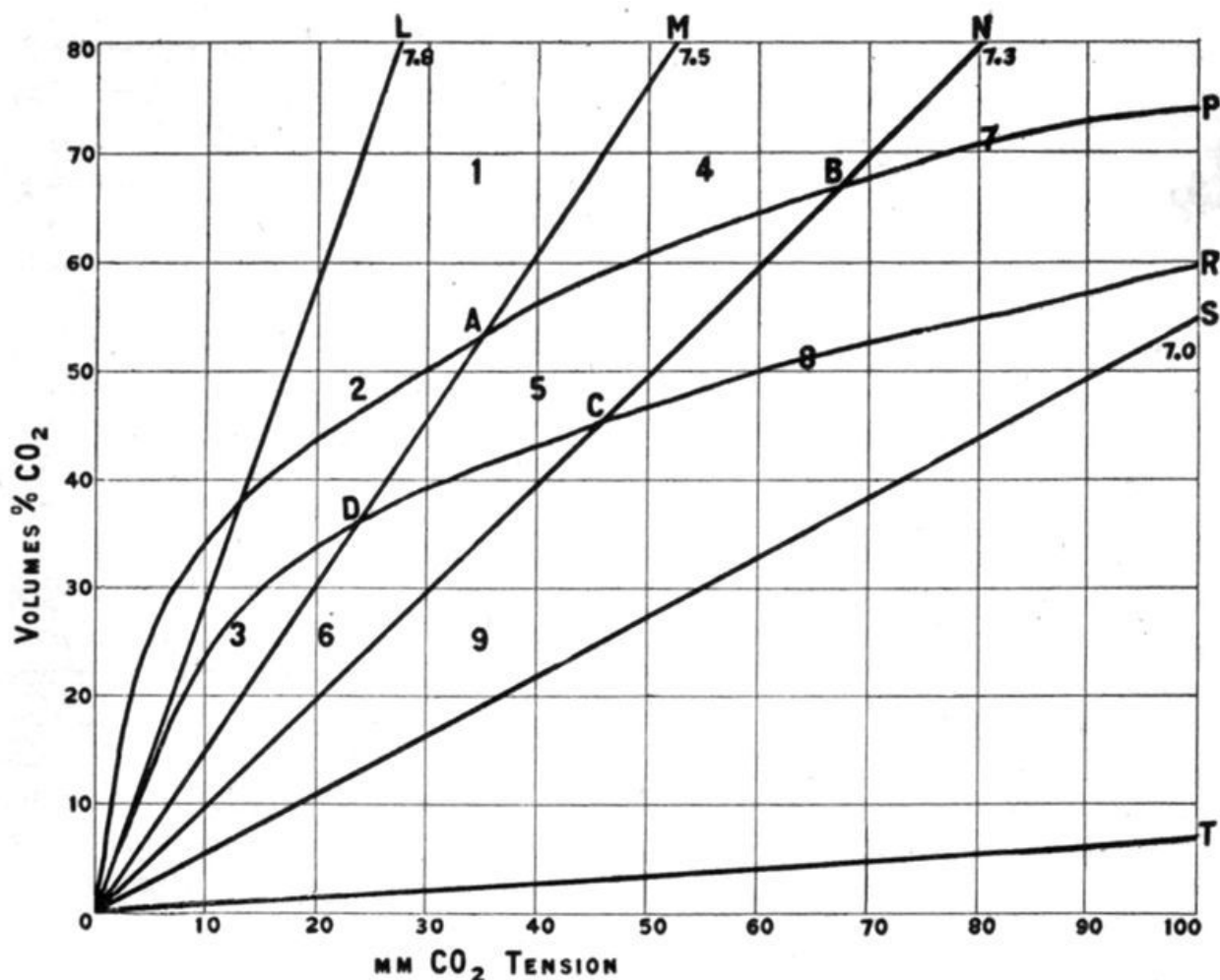
FIG. 152.—Carbon dioxide absorption curves. (Modified from Peters, Barr, and Rule, and Van Slyke).
