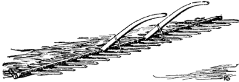
Figure 144.—Revolving Hayrake. The center piece is 4" x 6" x 12' long. The teeth are double enders \frac{3}{8} " square and 4' 6" long, which allows 24" of rake tooth clear of the center timber. Every stick in the rake is carefully selected. It is drawn by one horse. If the center teeth stick into the ground either the horse must stop instantly, or the rake must flop over, or there will be a repair job. This invention has never been improved upon for pulling Canada peas.
