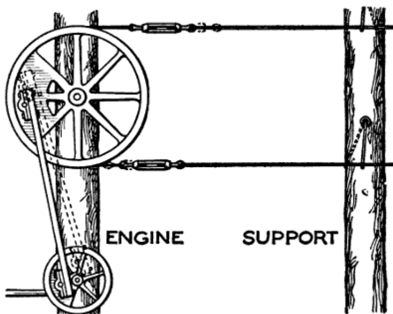
Figure 128.—Power Transmission. Circular motion is converted into reciprocating motion by the different lengths of the two pitman cranks which cause the upper wheel to oscillate. Power is carried to a distance by wires. To reduce friction the wires are supported by swinging hangers. Sometimes wooden rods are used instead of wires to lessen expansion and contraction.
