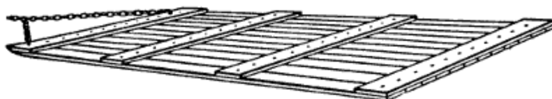
Figure 146.—Hay Skid. This hay skid is 8 feet wide and 16 feet long. It is made of \frac{5}{8} " lumber put together with 2" carriage bolts—plenty of them. The round boltheads are countersunk into the bottom of the skid and the nuts are drawn down tight on the cleats. It makes a low-down, easy-pitching, hay-hauling device.
