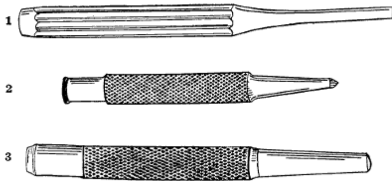
Figure 48.—(1) Tinner's Punch. Made of octagon steel in sizes to fit the rivets. The cutting end is flat and has sharp edges made by roll filing. It should be about 7" long and from \frac{3}{8} " to \frac{1}{2} " in diameter, according to the size of rivet and thickness of sheet metal to be punched. (2) Prick Punch. Usually made rather short and stocky. It may be \frac{1}{2} " or \frac{5}{8} " diameter and 4\frac{1}{2} " to 5" long. (3) Hot-iron Punch. Made in many sizes and lengths. The taper should be the same as the drawing.
