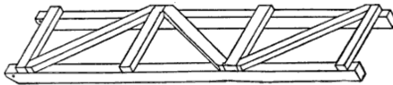
Figure 137.—Harrow Sled Long Enough to Hold a Four-Section Harrow.
