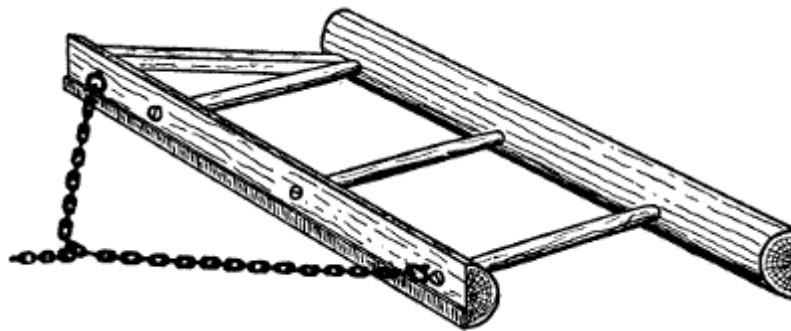
Figure 223.—Split-Log Road Drag. The front edge is shod with a steel plate to do the cutting and the round side of the rear log grinds the loosened earth fine and presses it into the wagon tracks and water holes.
