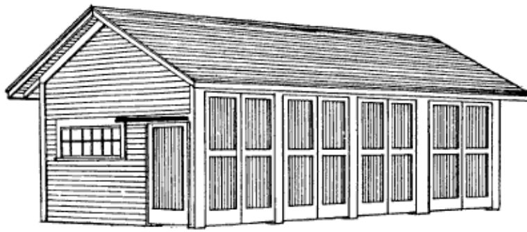
Figure 3.—Perspective View of Farm Implement Shed and Workshop.
