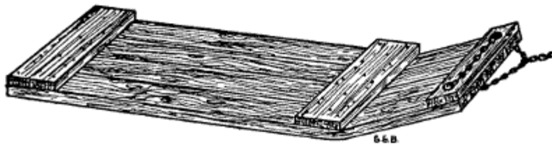
Figure 158.—Stone-Boat. Stump logs are selected for the planks. The bend of the planks is the natural curve of the large roots. The sawing is done by band saw cutting from two directions.
