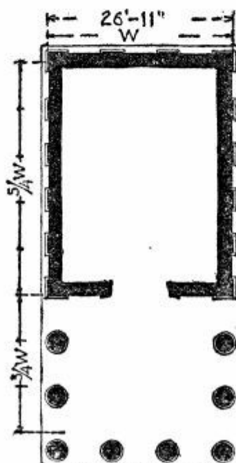
TEMPLE OF HERCULES AT CORI
