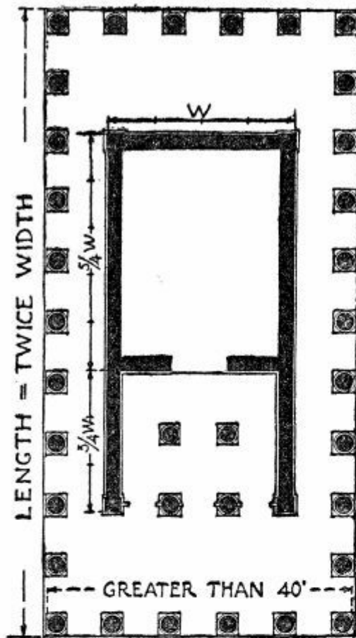
ACCORDING TO VITRUVIUS
