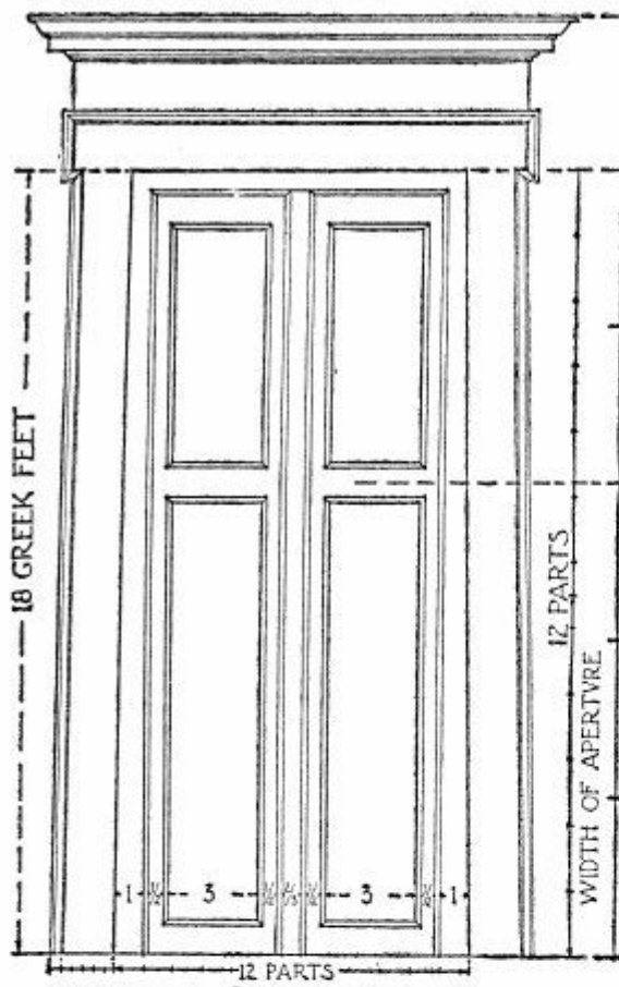
VITRUVIUS' DORIC DOORWAY
