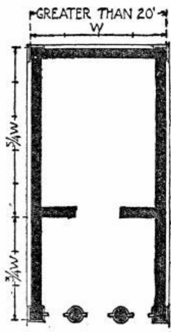
ACCORDING TO VITRUVIUS
