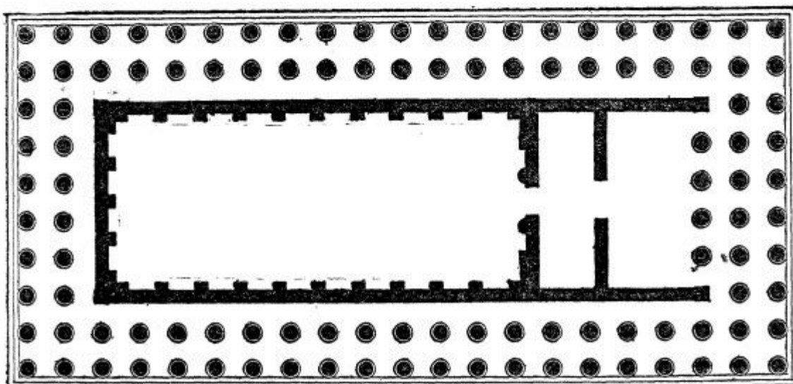
TEMPLE OF APOLLO DIDYMAEVS NEAR MILETVS
