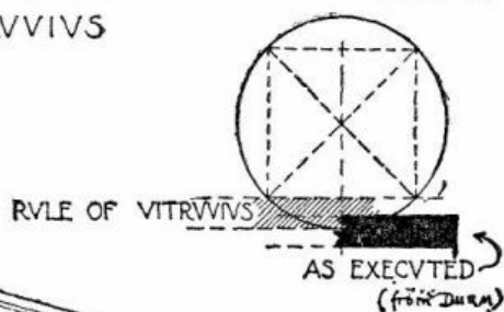
THEATRE AT OROPVS
