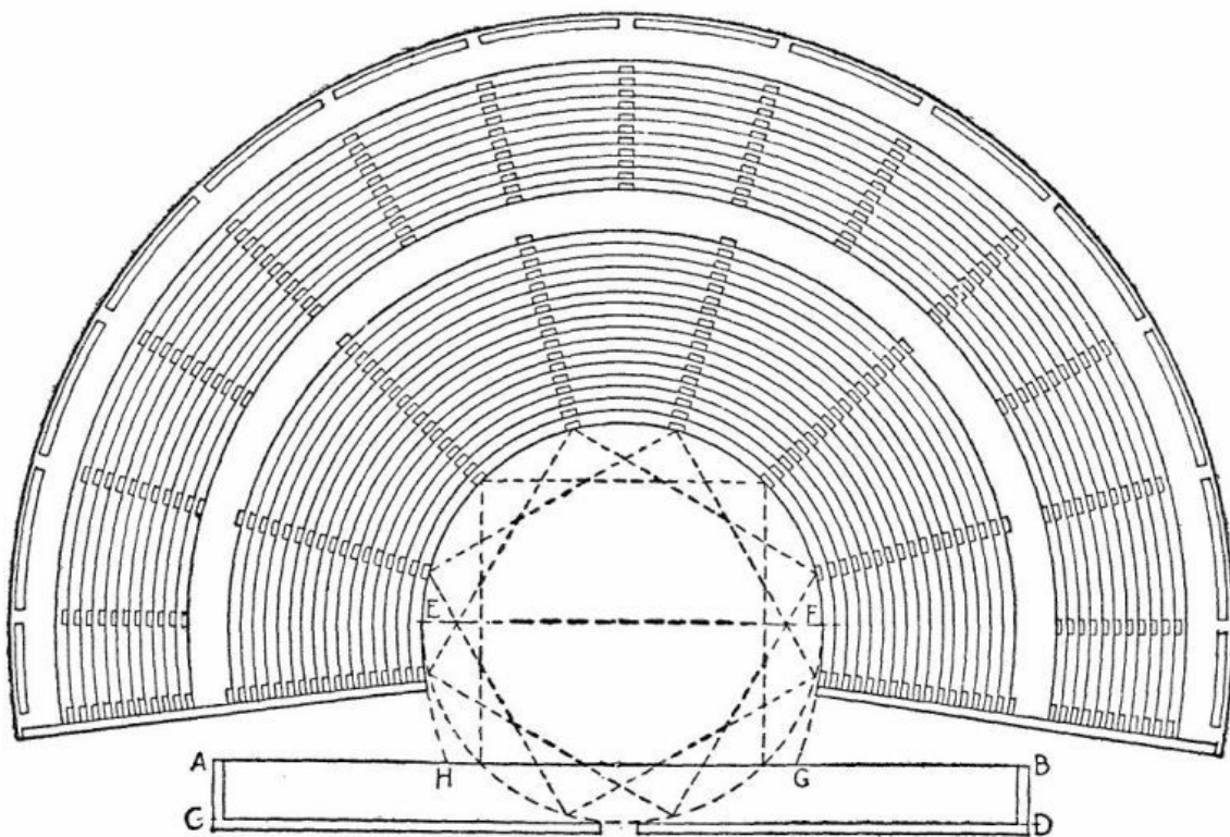
THEATRE AT EPIDAVRVS
