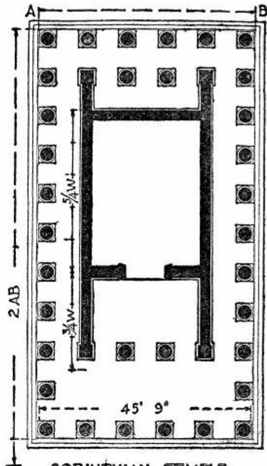
CORINTHIAN TEMPLE AT LABRANDA
