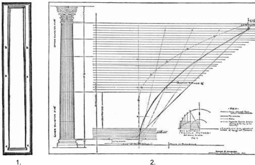
THE ENTASIS OF COLUMNS
