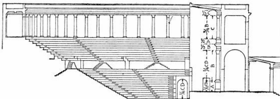
SECTION
