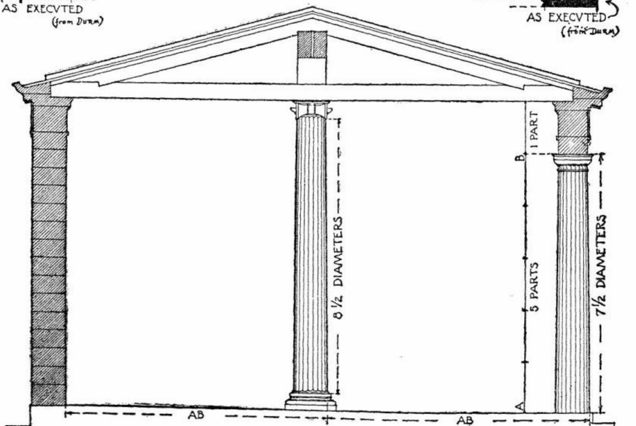
THE THEATRE PORTICO
