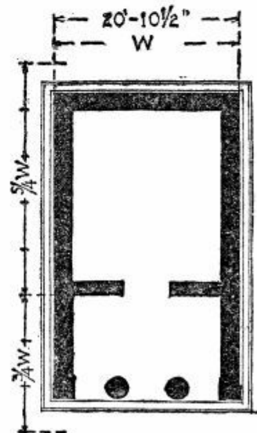
TEMPLE OF THEMIS AT RHAMNUS
