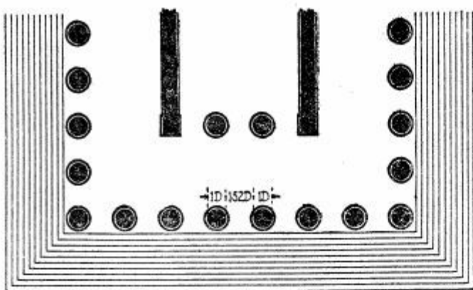
THE SMINTHEVM APPROXIMATELY A PYCNOSTYLE ARRANGEMENT
