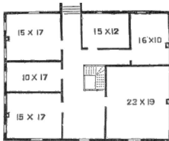
CHAMBER PLAN.
