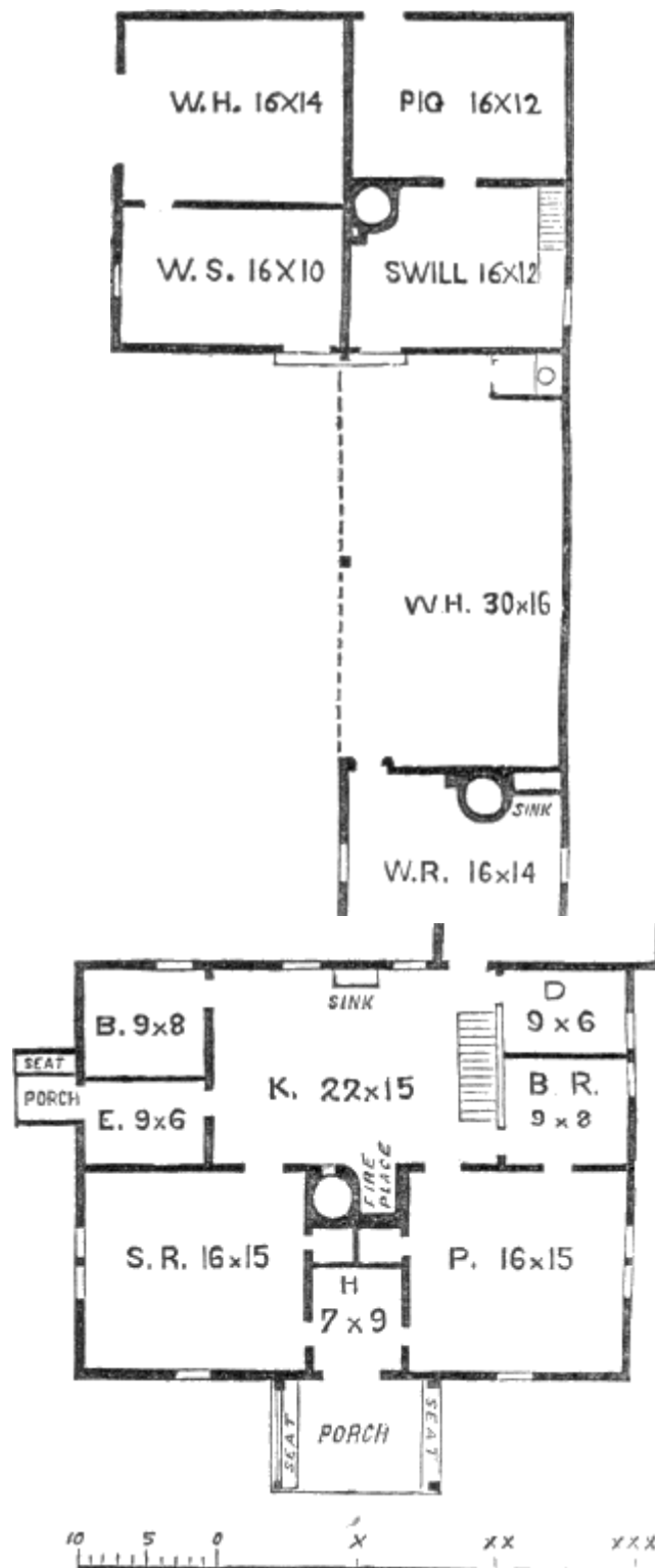
GROUND PLAN.
