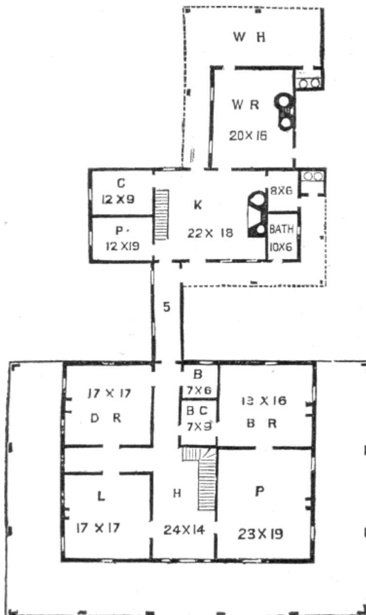
GROUND PLAN.
