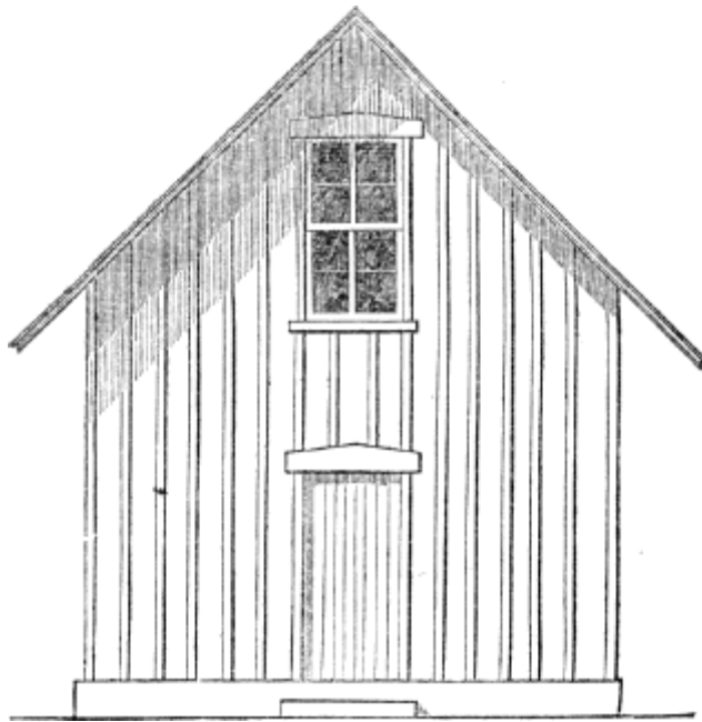
NO. I.—ELEVATION.
