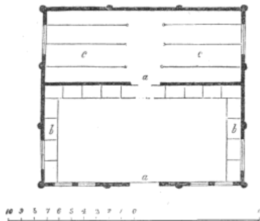
GROUND PLAN.
