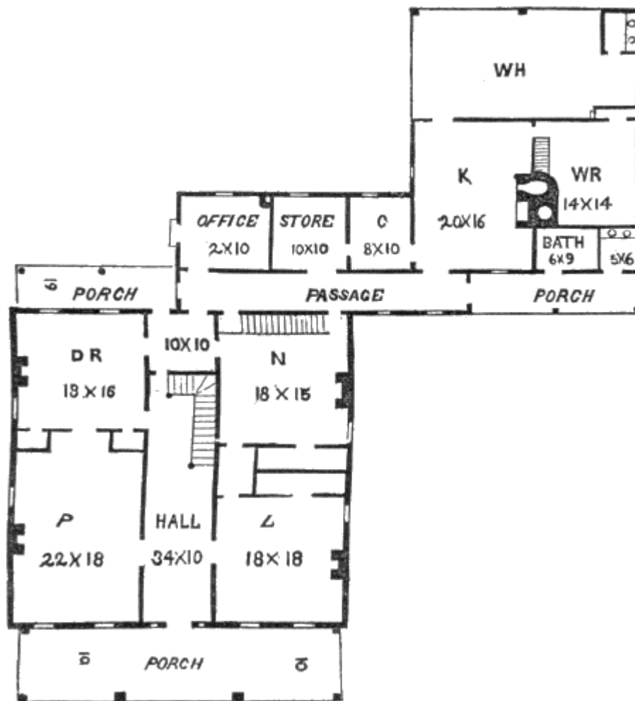
GROUND PLAN
