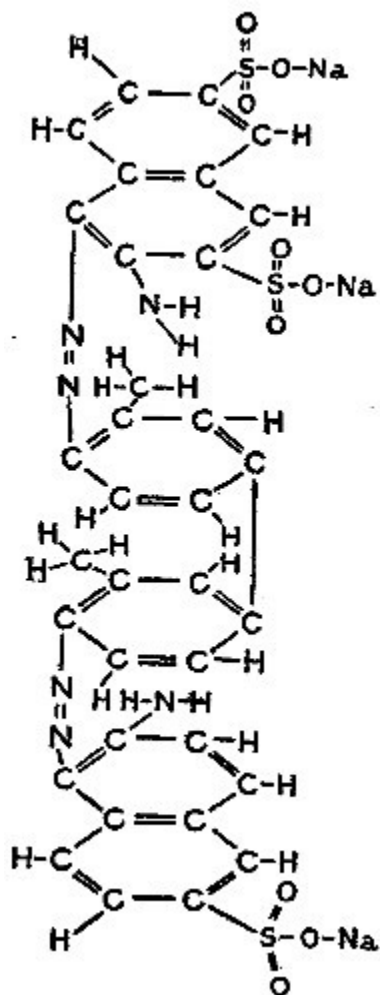
A molecule of a coal-tar dye
