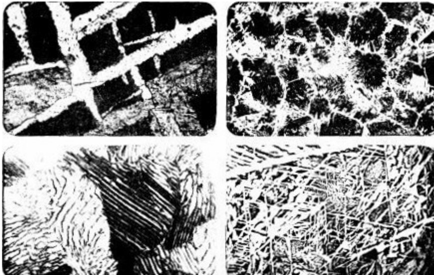
PHOTOMICROGRAPHS SHOWING THE STRUCTURE OF STEEL MADE BY PROFESSOR E.G. MARTIN OF PURDUE UNIVERSITY
