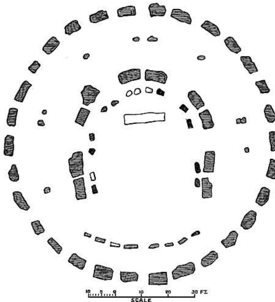
24. Plan of Stonehenge restored.
