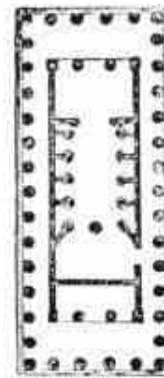
TEMPLE OF APOLLO, BASSAE
