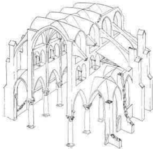
SKELETON STRUCTURE SHOWING THE METHOD OF VAULTING, BY MEANS OF THE POINTED ARCH, AND THE CONCENTRATION OF THRUSTS AND COUNTER THRUSTS. P. 273
