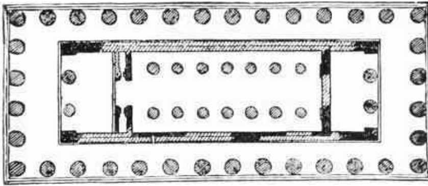
TEMPLE OF POSEIDON, PAESTUM. HEXASTYLE- PERIPTERAL
