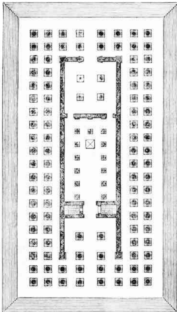
TEMPLE OF JUPITER OLYMPUS, ATHENS. OCTOSTYLE-DIPTERAL
