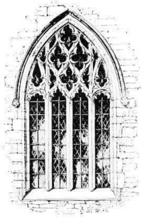
EARLY PERPENDICULAR KING'S SUTTON, NORTHAMPTONSHIRE
