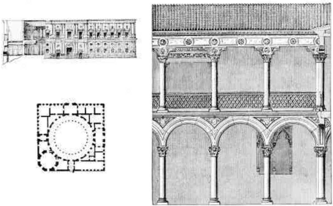
ELEVATION AND PLAN OF THE UNCOMPLETED PALACE IN CLASSICAL STYLE, OF CHARLES V IN THE ALHAMBRA GROUNDS. P. 402
