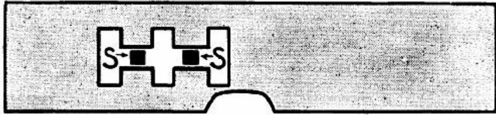
FIG. 215.—The bolt of a Barron lock.
