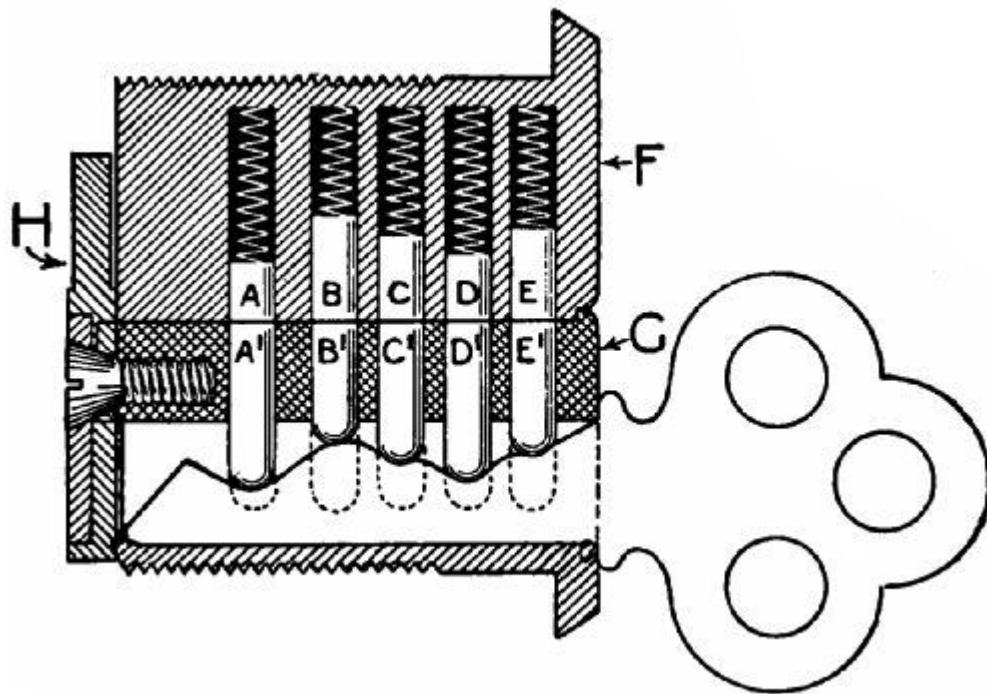
FIG. 219.—Section of a Yale lock.
