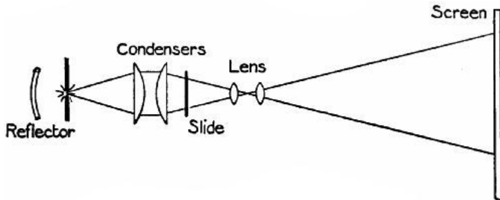
FIG. 130.—Sketch of the elements of a magic-lantern.
