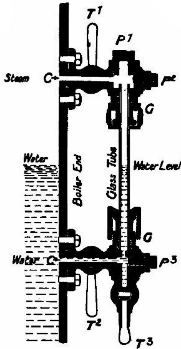
FIG. 12.—Section of a water-gauge.
