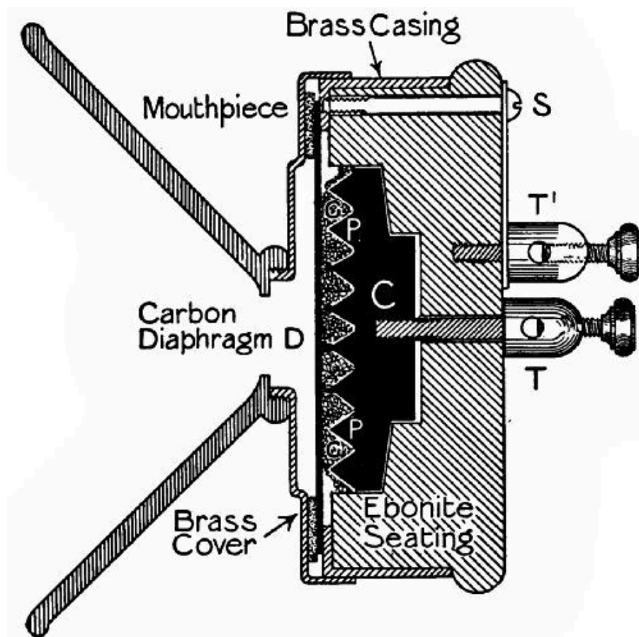
FIG. 63.—Section of a granular carbon transmitter.
