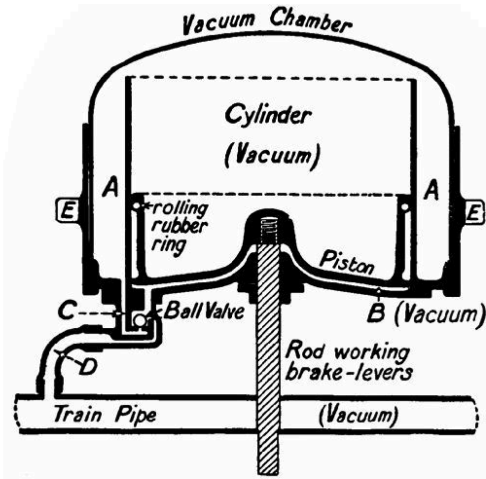
FIG. 85.—Vacuum brake "off."
