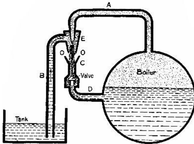
FIG. 15.—Diagram illustrating the principle of a steam-injector.
