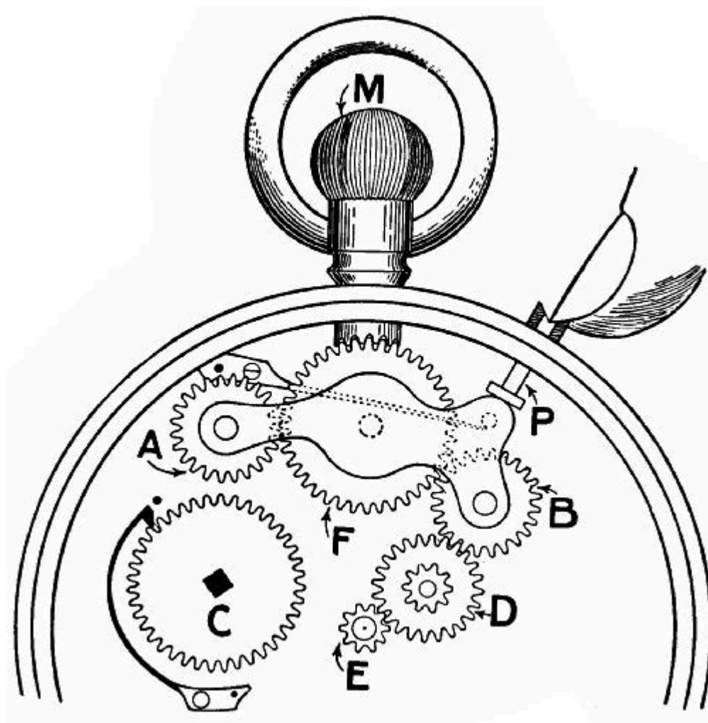
FIG. 210.—The hand-setting mechanism in action.
