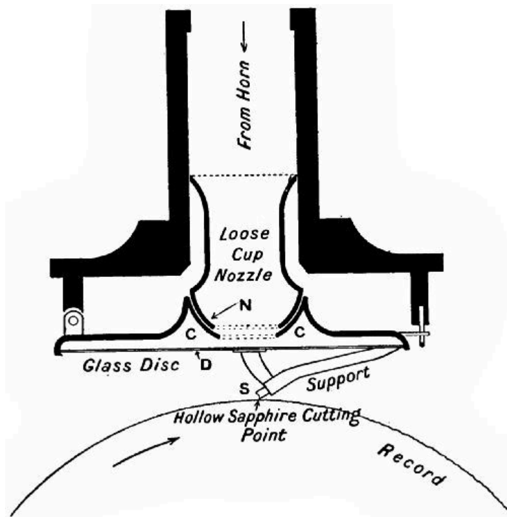
FIG. 147.—Section of an Edison Bell phonograph recorder.
