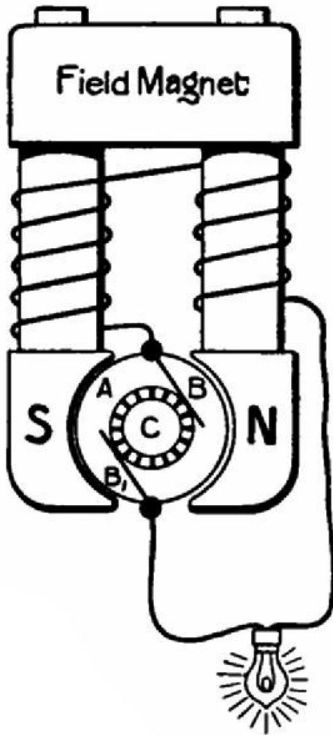
FIG. 77.—Sketch showing a "series" winding.
