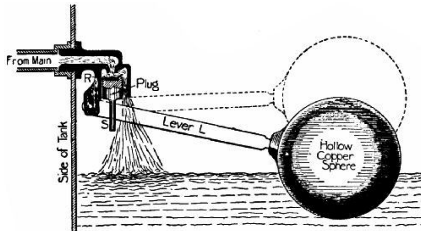
FIG. 182.—An automatic ball-valve.
