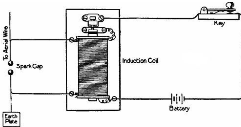
FIG. 59.—Sketch of the transmitter of a wireless telegraphy outfit.
