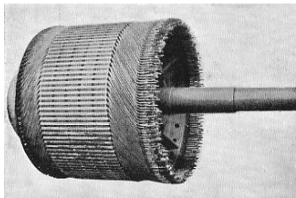
FIG. 75.—Partly finished commutator.
