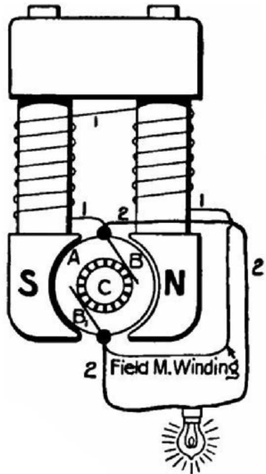
FIG. 78.—"Shunt" winding.
