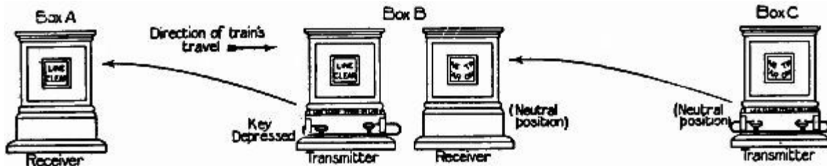
FIG. 100.—The signaling instruments in three adjacent cabins. The featherless arrows show the connection of the instruments.
