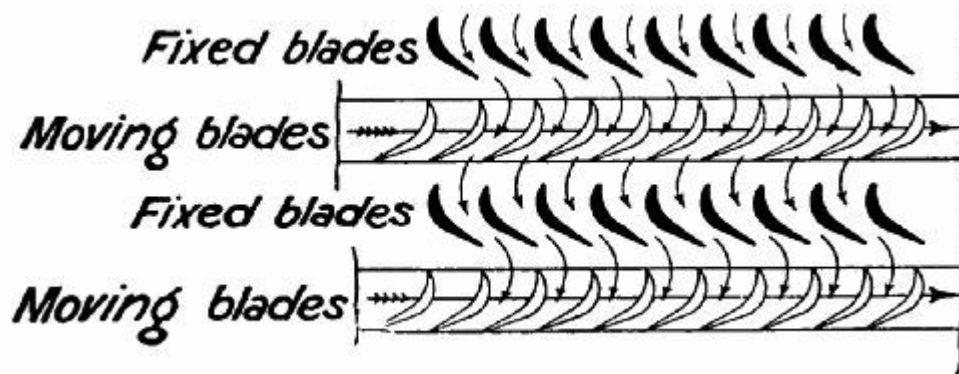
FIG. 38.—Blades or vanes of a Parsons turbine.
