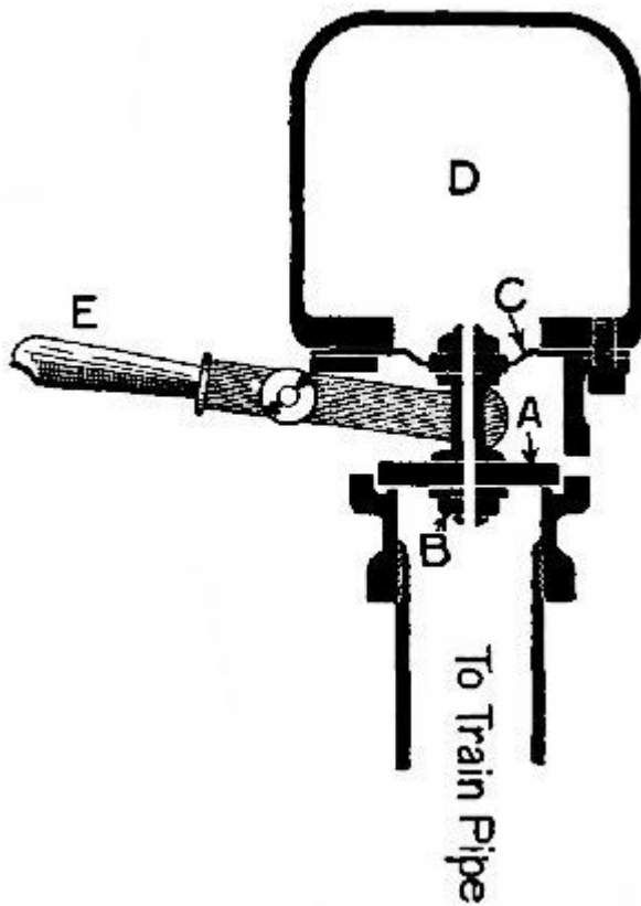
FIG. 87.—Guard's valve for applying the Vacuum brake.
