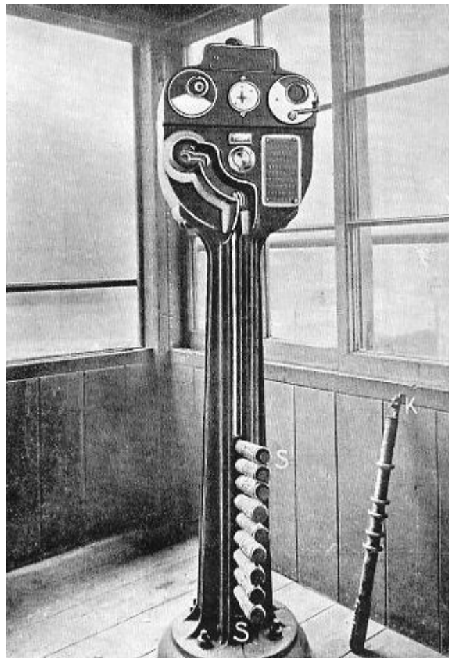
FIG. 101.—An electric train staff holder: s s, staffs in the slot of the instrument. Leaning against the side of the cabin is a staff showing the key κ at the end for unlocking a siding points between two stations. The
