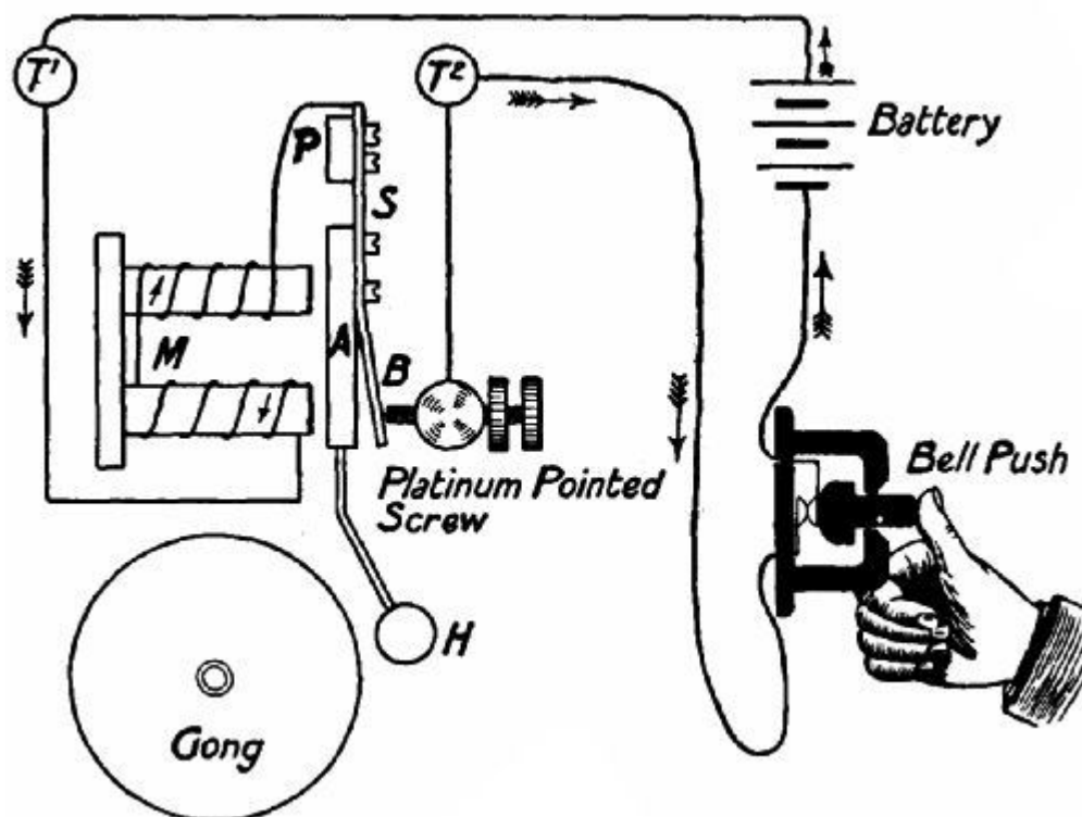
FIG. 52.—Sketch of an electric-bell circuit.
