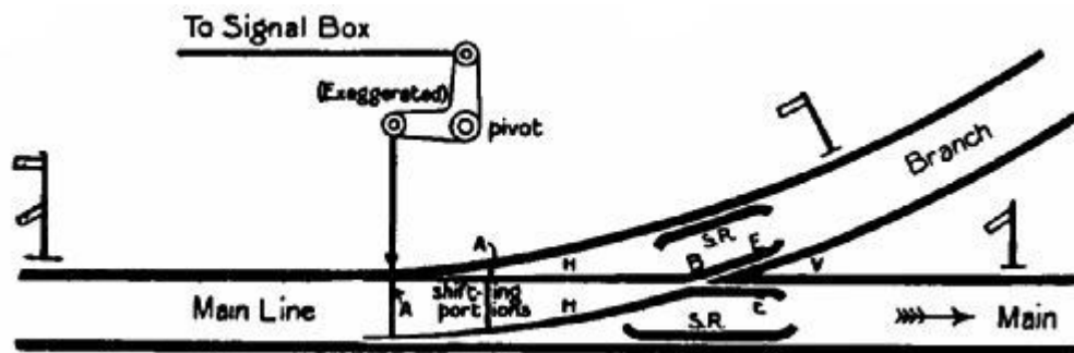
FIG. 98.—Points open to main line.
