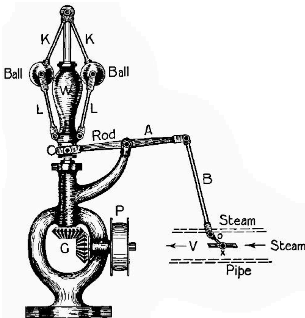
FIG. 33.—A speed governor.
