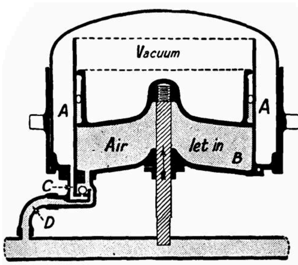
FIG. 86.—Vacuum brake "on."
