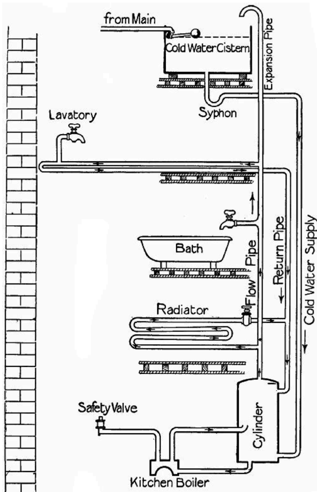
FIG. 193.—The "cylinder" system of hot-water supply.
