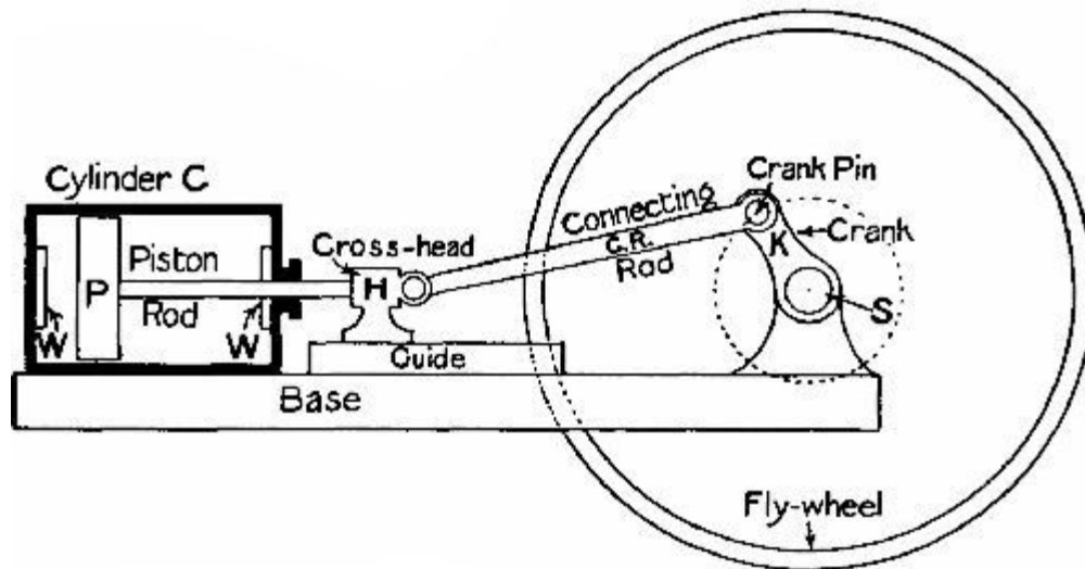
FIG. 17.—Sketch showing parts of a horizontal steam-engine.
