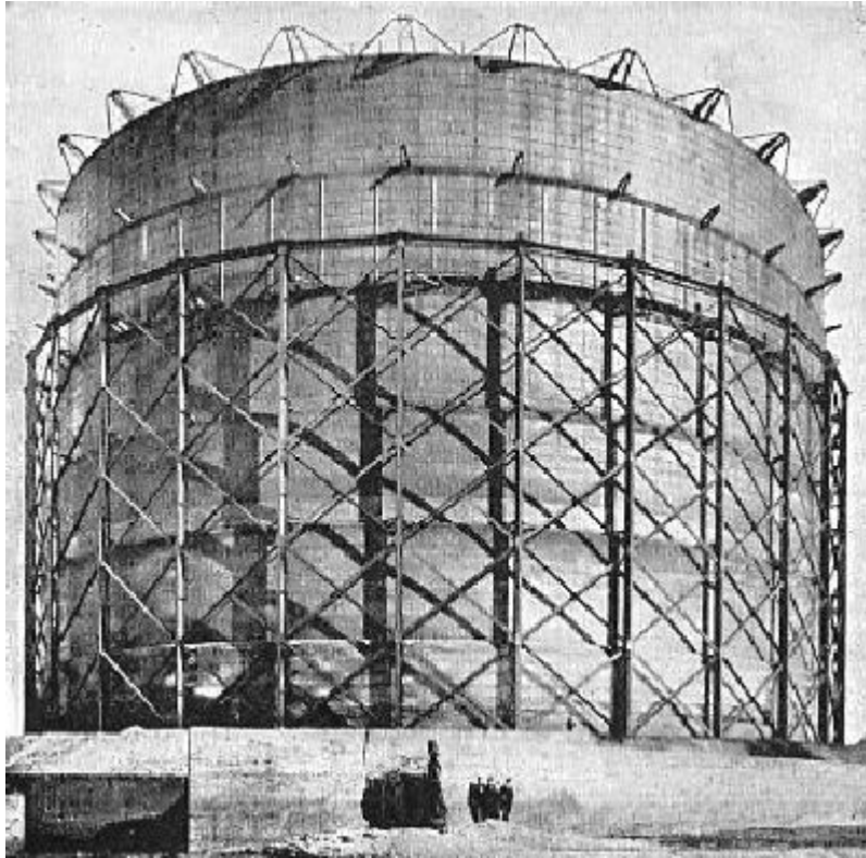
FIG. 196.—The largest gasholder in the world: South Metropolitan Gas Co., Greenwich Gas Works. Capacity, 12,158,600 cubic feet.
