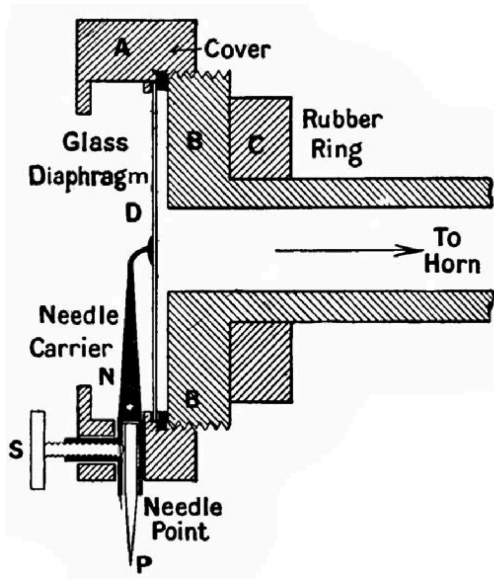
FIG. 151c.—Section of a gramophone reproducer.
