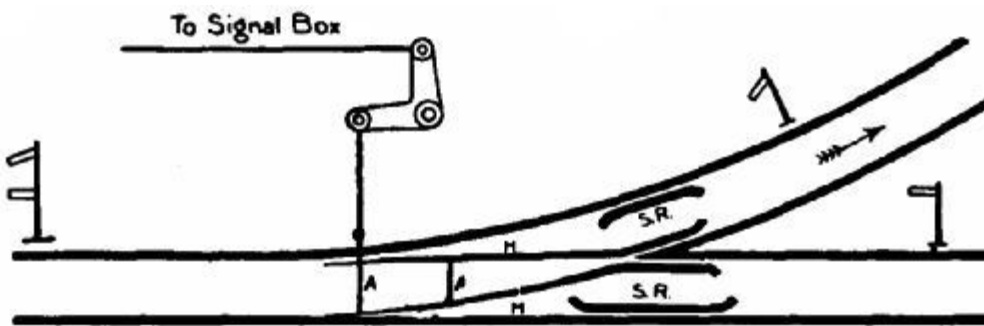
FIG. 99.—Points open to branch line.
