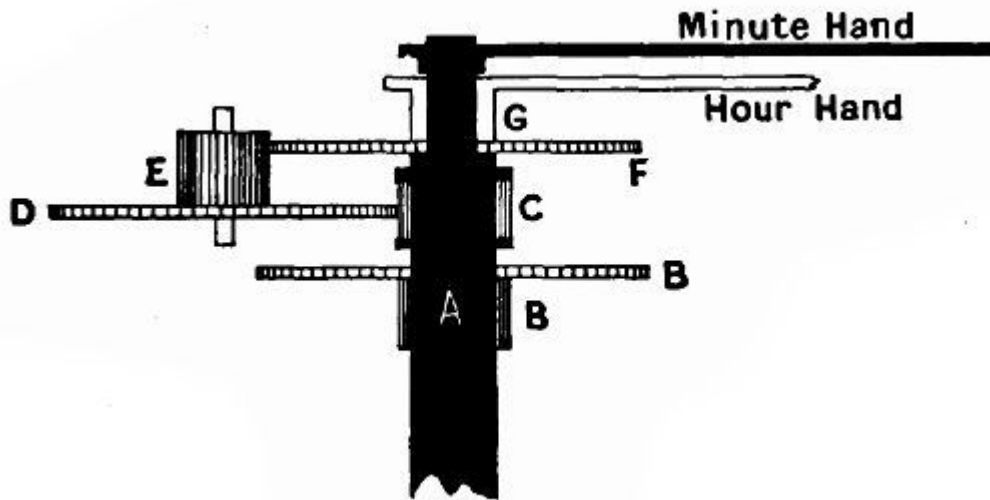
FIG. 211.—The hour-hand train of a clock.
