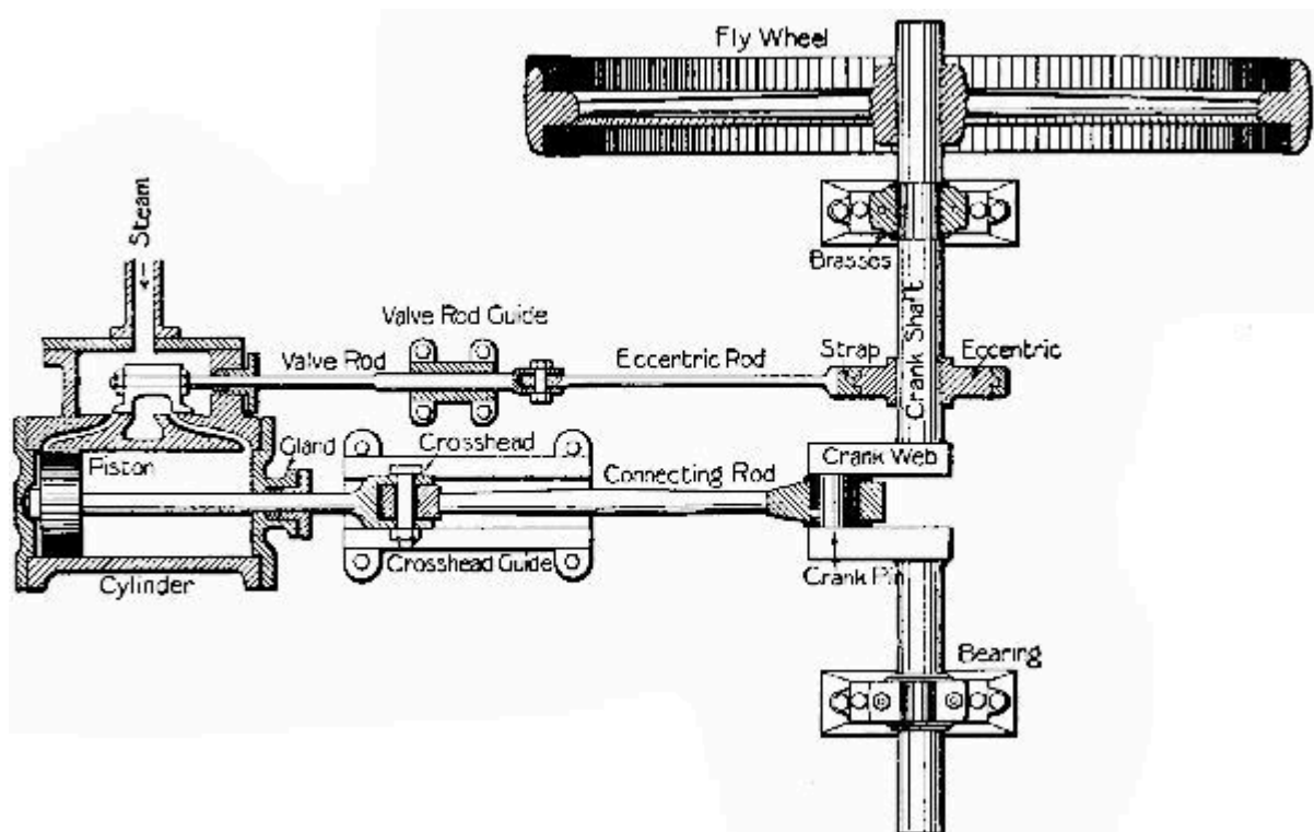
FIG. 18.—Sectional plan of a horizontal engine.
