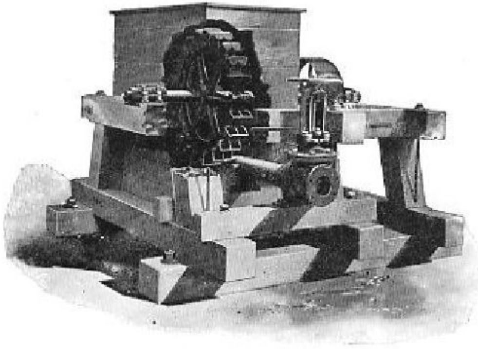
FIG. 188.—Pelton wheel mounted, with nozzle in position.
