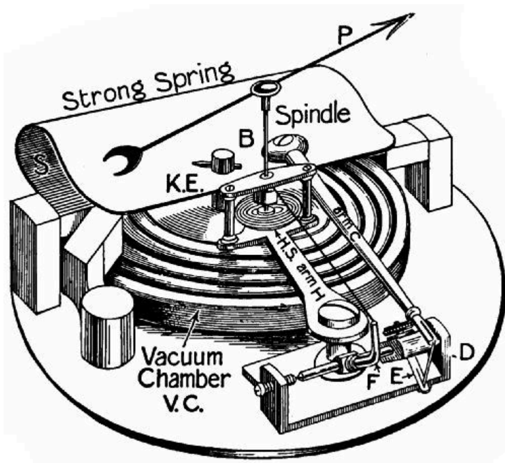
FIG. 155.—An aneroid barometer.
