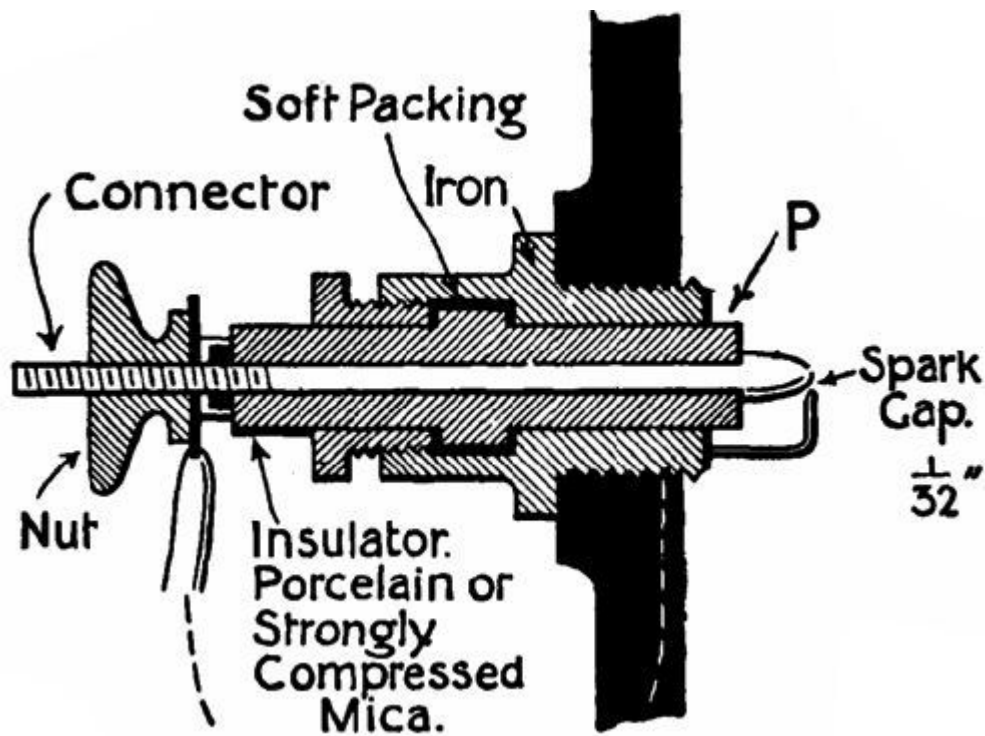
FIG. 46.—Section of a sparking-plug.
