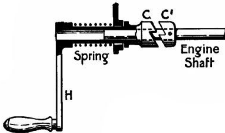
FIG. 41.—The starting-handle.
