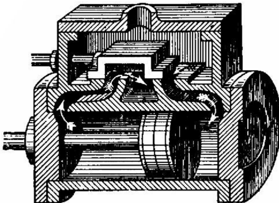
FIG. 22.—Perspective section of cylinder.
