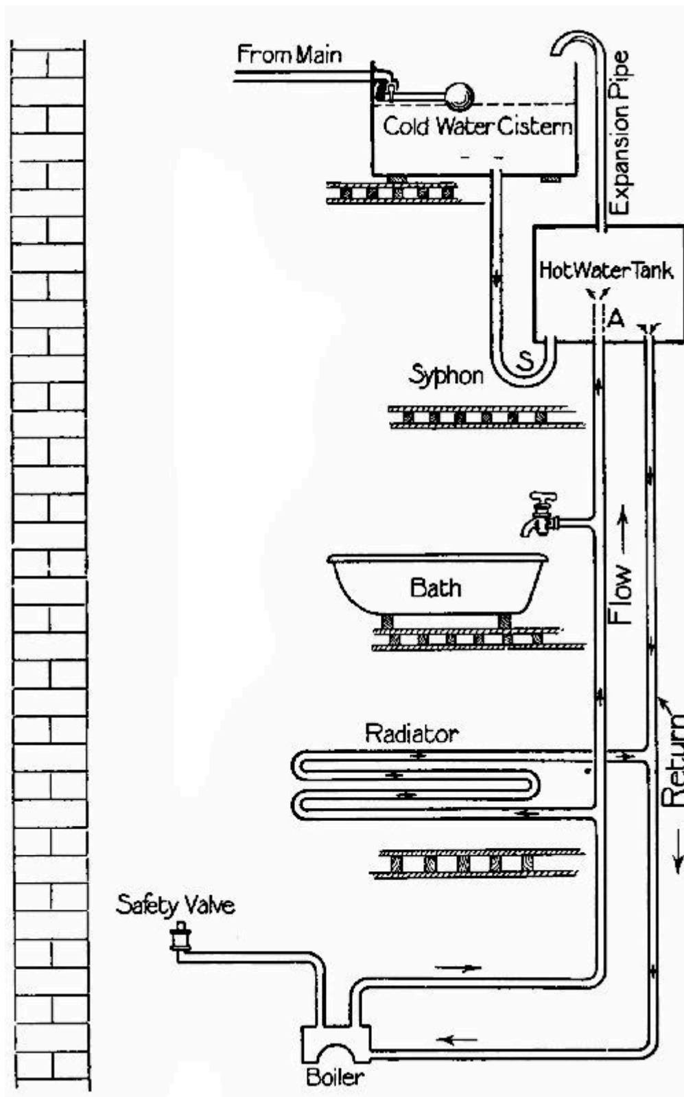
FIG. 192.—The "tank" system of hot-water supply.
