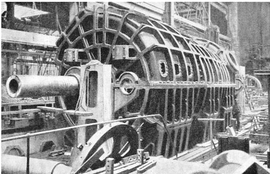
One of the low-pressure turbines of the Carmania, in casing. Its size will be inferred from comparison with the man
