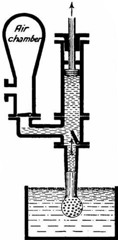
FIG. 175. Force-pump; suction stroke. FIG. 176. Force-pump; delivery stroke.
