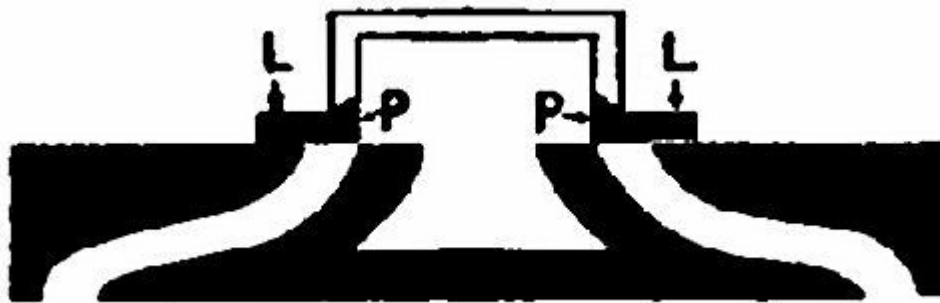
FIG. 27.—A slide-valve with "lap."
