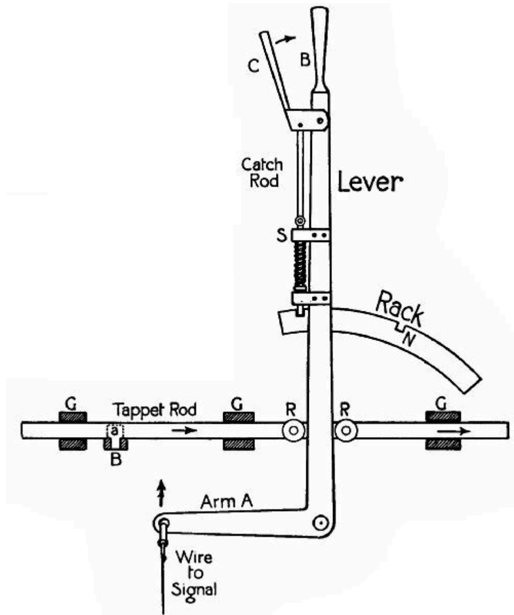
FIG. 93. —A signal lever and its connections. To move the lever, C is pressed towards B raising the catch-rod from its
