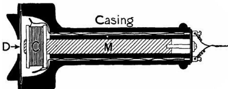
FIG. 62.—Section of a Bell telephone.
