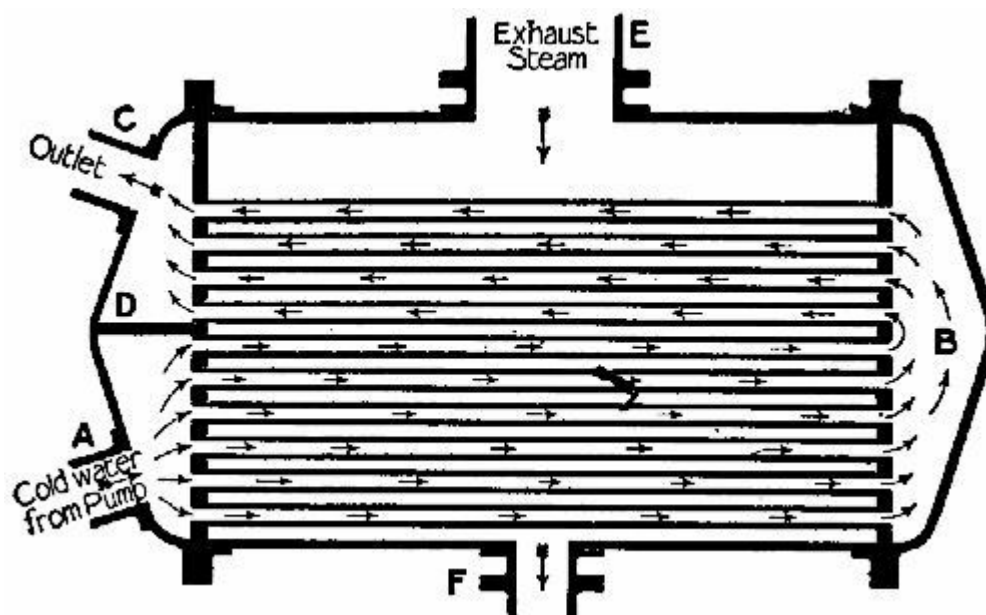
FIG. 35.—The marine condenser.
