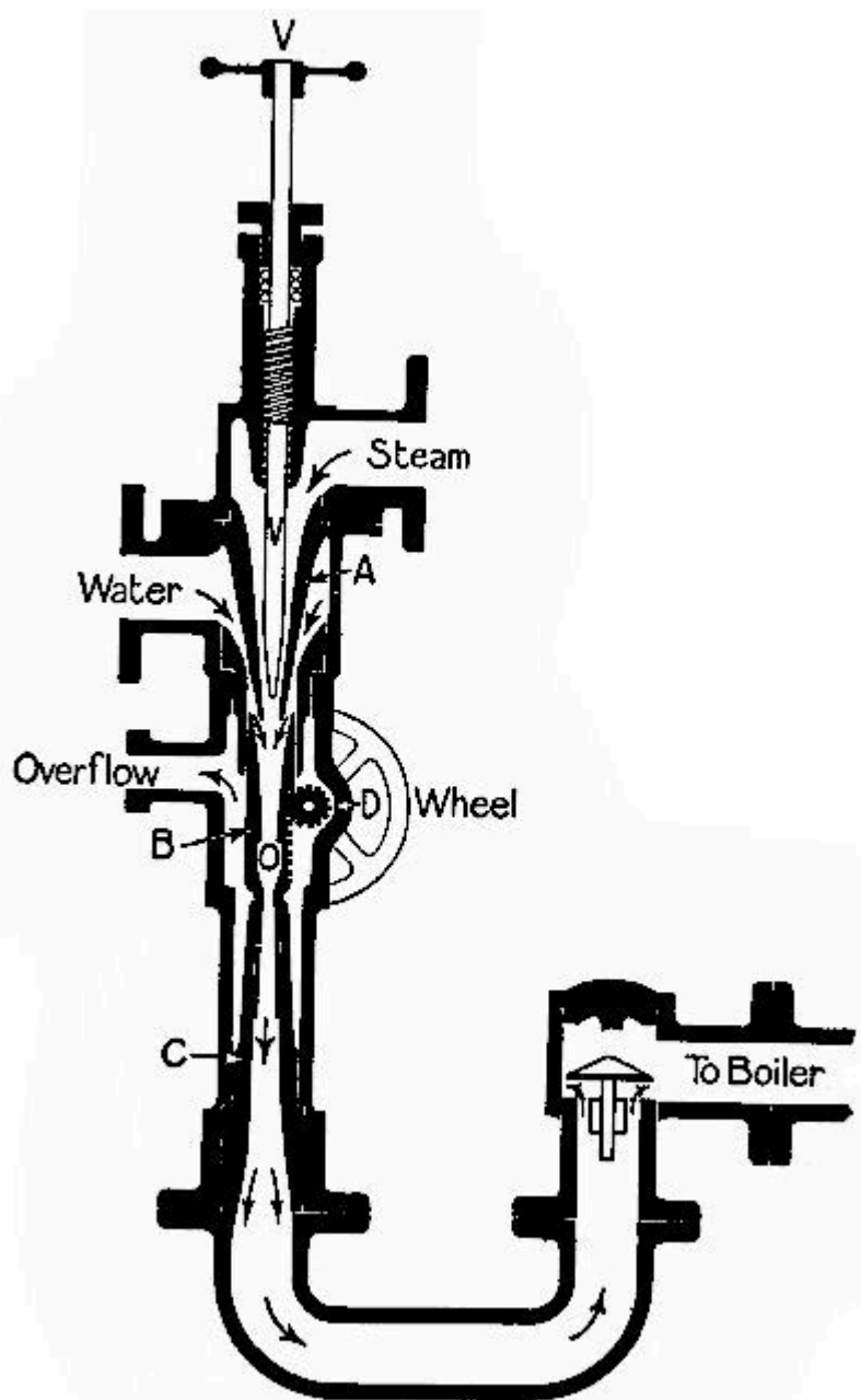
FIG. 16.—The Giffard injector.
