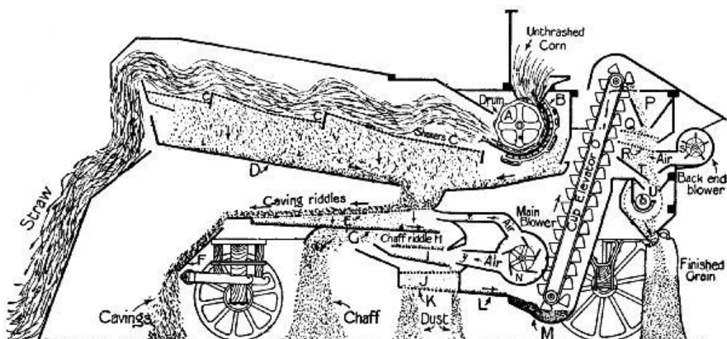
FIG. 226.—Section of a threshing machine.
