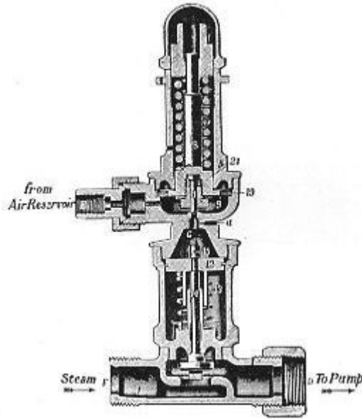
FIG. 90.—Air-pump of Westinghouse brake.
