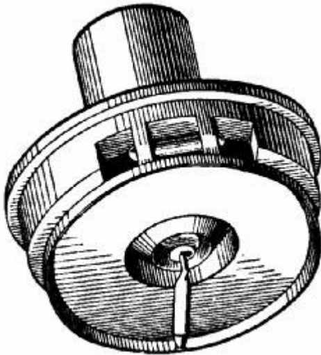
FIG. 148.—Perspective view of a phonograph recorder.
