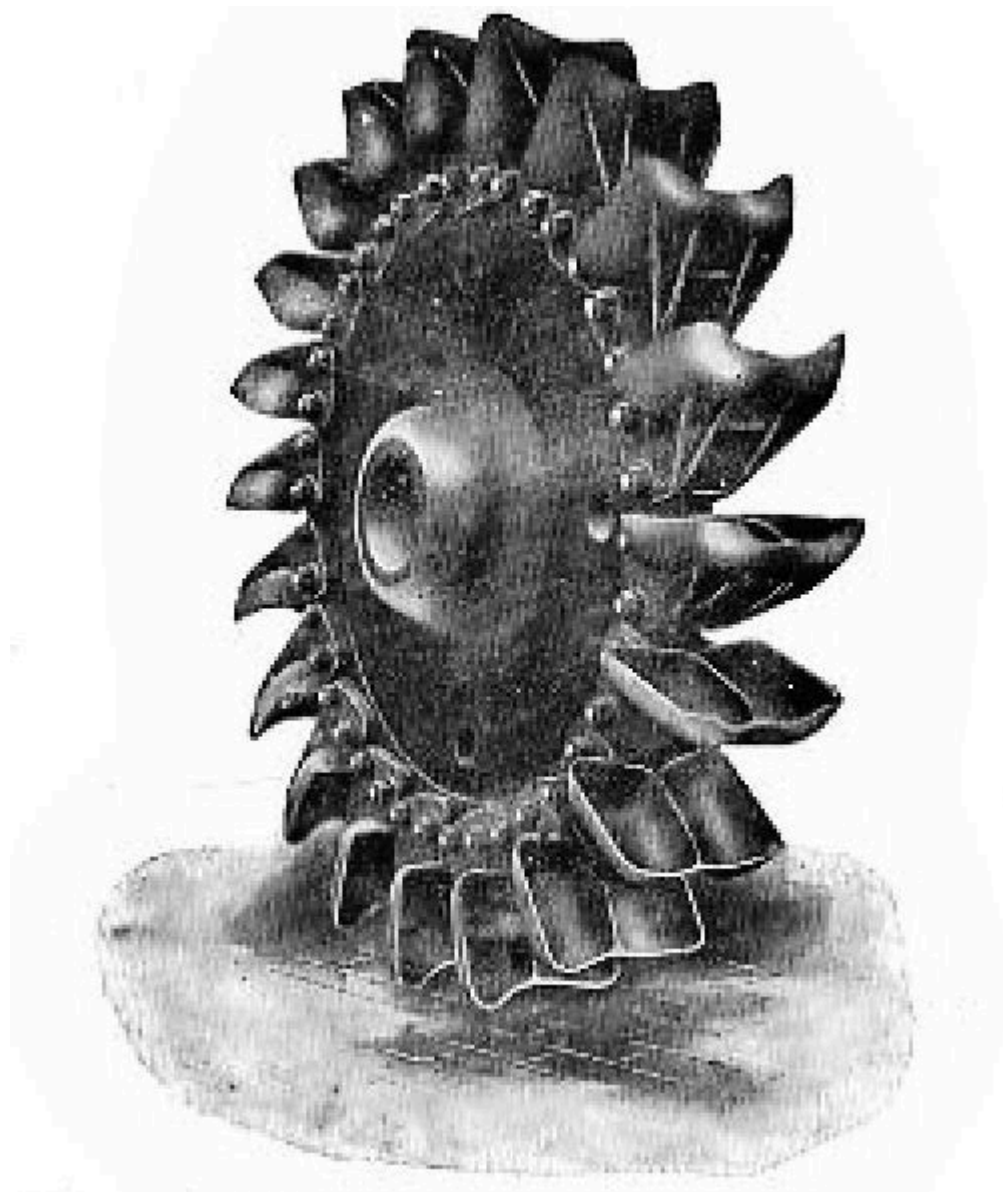
FIG. 187.—A Pelton wheel which develops 5,000 horse-power. Observe the shape of the double buckets.
