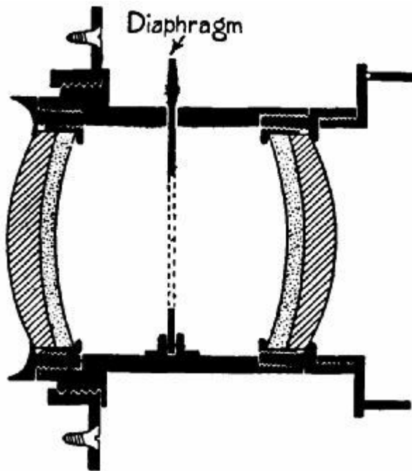
FIG. 115.—Section of a rectilinear lens.
