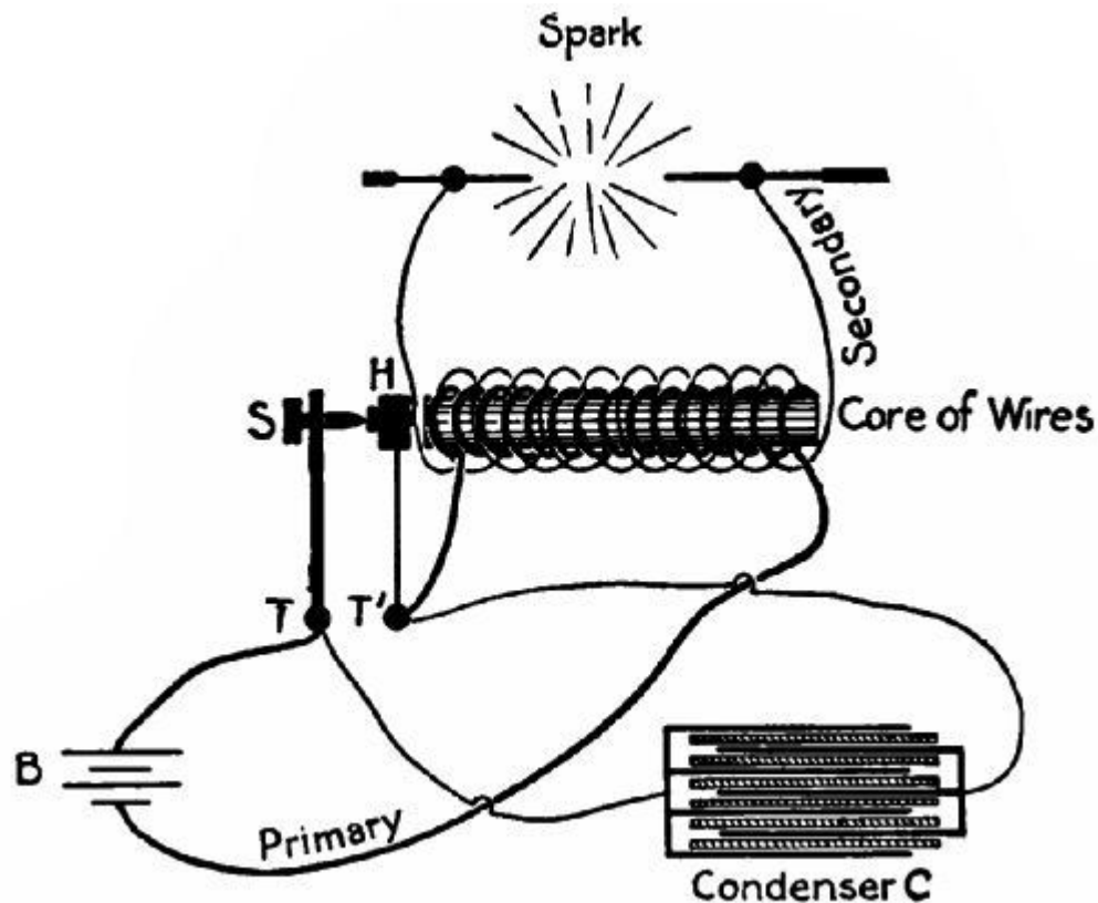
FIG. 53.—Sketch of an induction coil.
