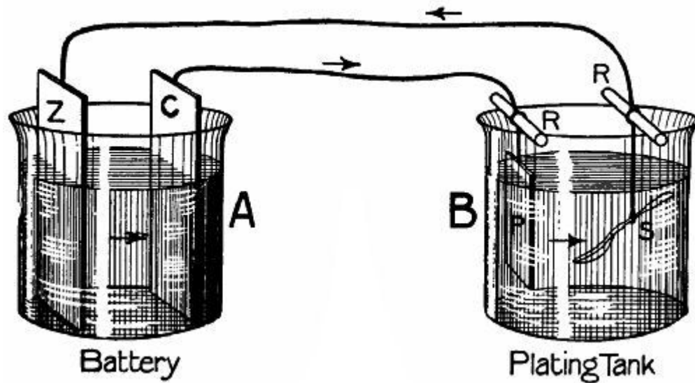
FIG. 84.—An electroplating outfit.
