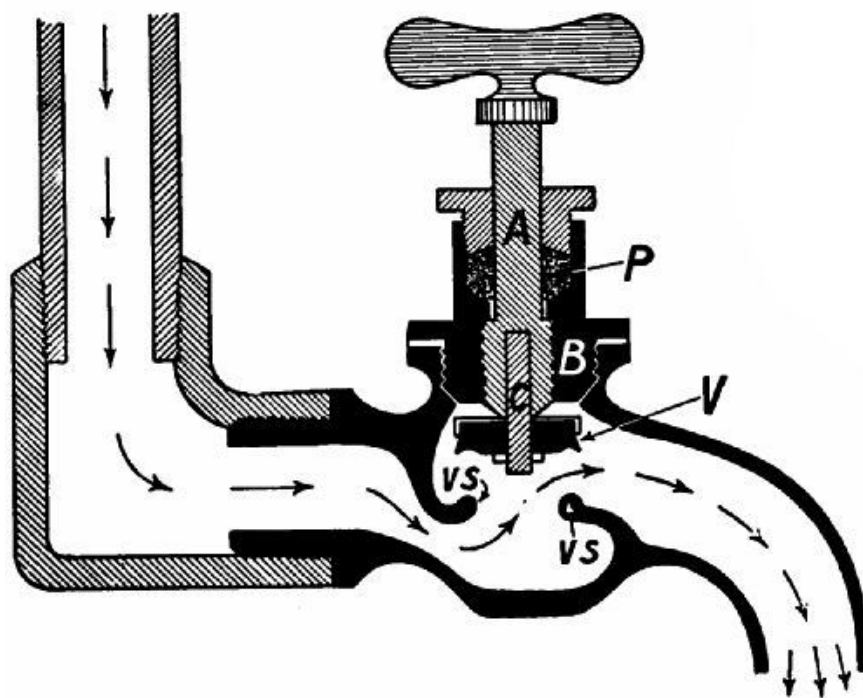
FIG. 181.—A screw-down water cock.
