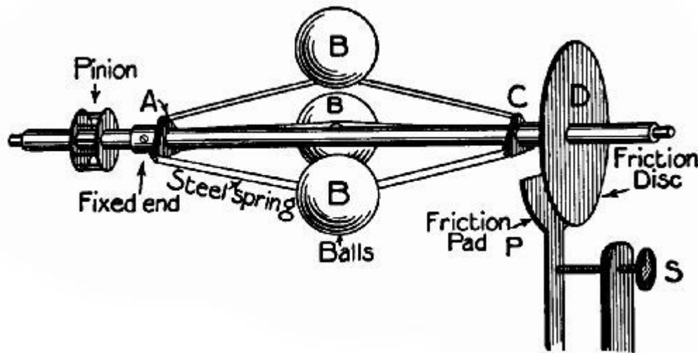
FIG. 146.—The "governor" of a phonograph.
