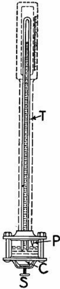
FIG. 152.—A Fortin barometer.
