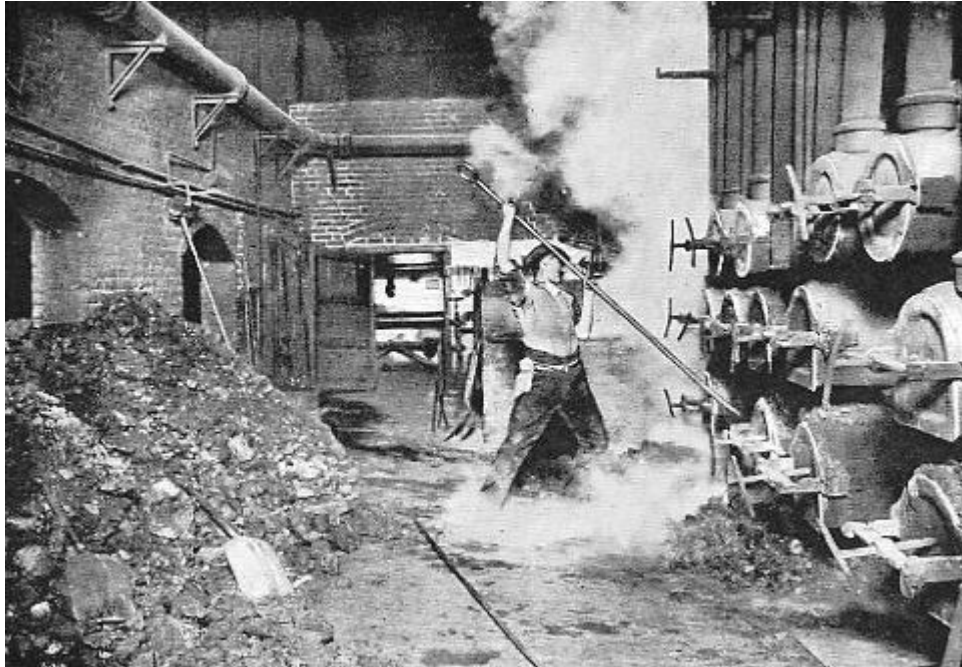
FIG. 197.—Drawing retorts. (Photo by F. Marsh.)
