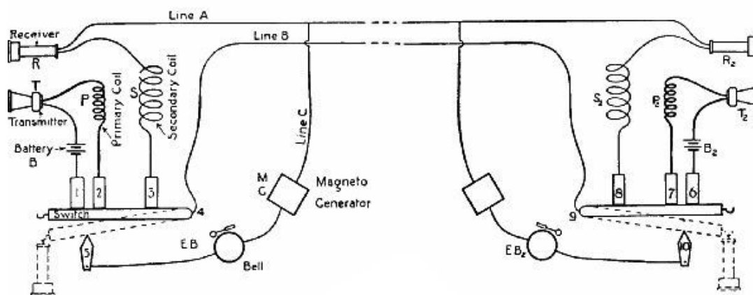
FIG. 64.—A diagrammatic representation of a telephonic circuit.
