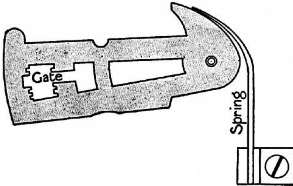
FIG. 216.—Tumbler of Chubb lock.
