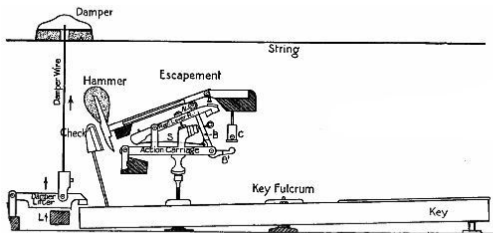
FIG. 135.—The striking mechanism of a "grand" piano.
