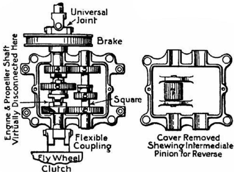
FIG. 48.—The gear-box of a motor car.
