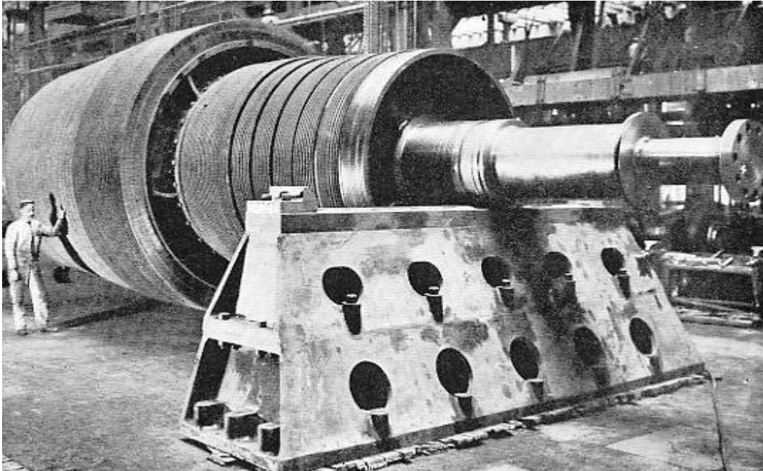
One of the turbine drums of the Carmania. Note the rows of vanes. The drum is here being tested for perfect balance on two absolutely level supports.
