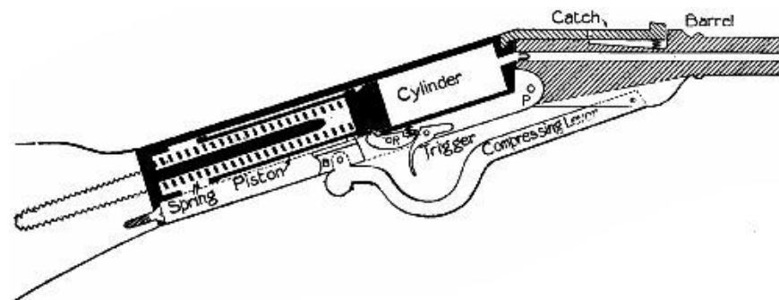
FIG. 168.—Section of the mechanism of an air-gun.
