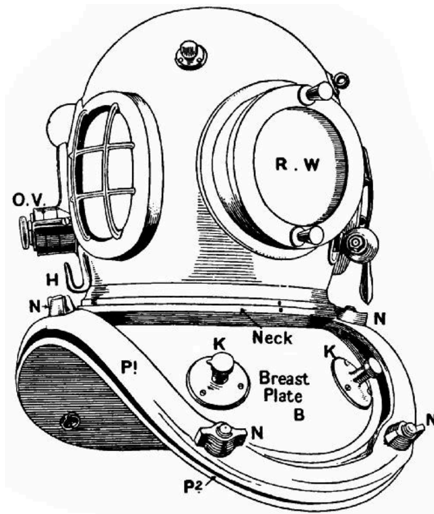
FIG. 161.—A diver's helmet.
