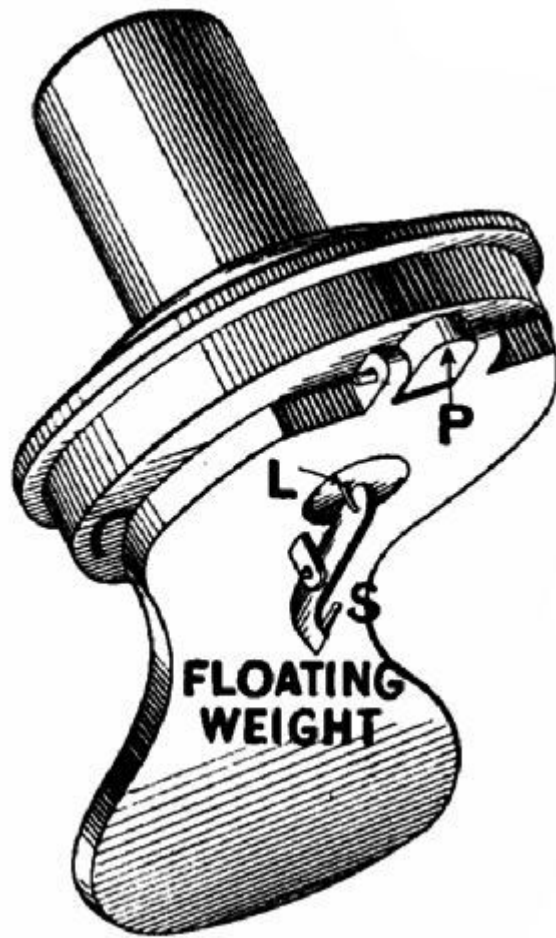
FIG. 150.—Perspective view of a phonograph reproducer.
