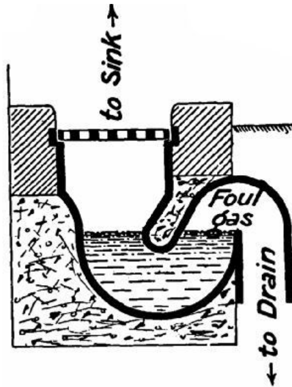
FIG. 186.—A trap for foul air.
