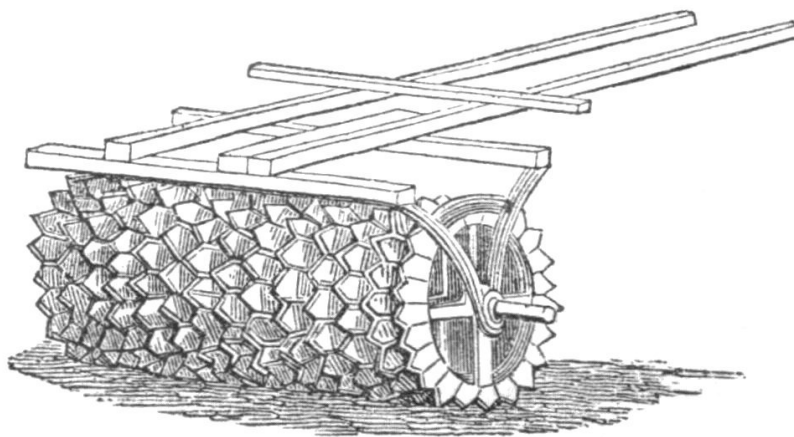
CROSSKILL'S PATENT CLOD-CRUSHER ROLLER.
