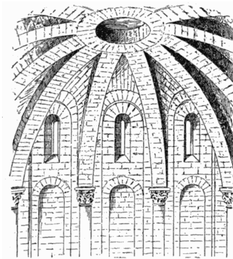
28. MONASTERY CHURCH AT MOISSAC. VAULT OF THE HALL KNOWN AS THE HALL OF THE CAPTAINS ABOVE THE PORCH
