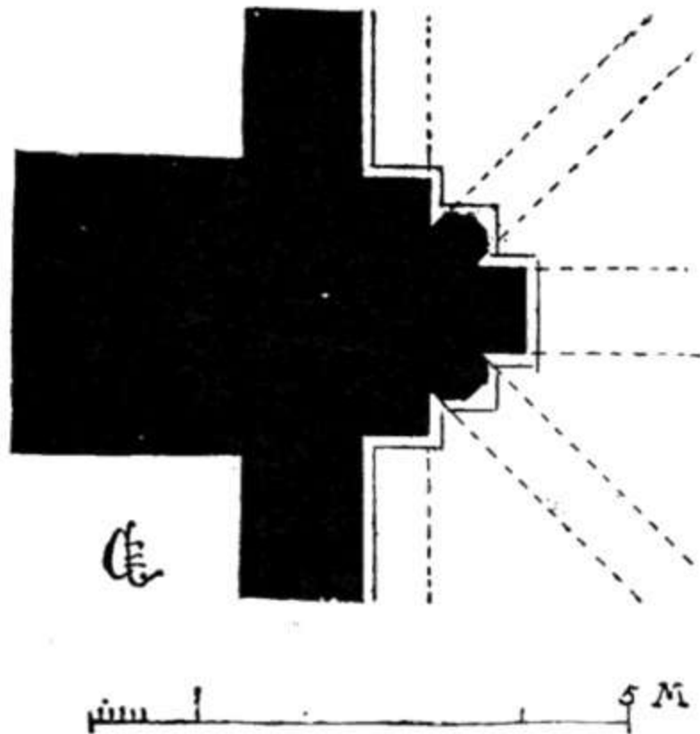
16. PLAN OF A SUMMER OF THE NAVE VAULT OF LA STE. TRINITÉ AT LAVAL
