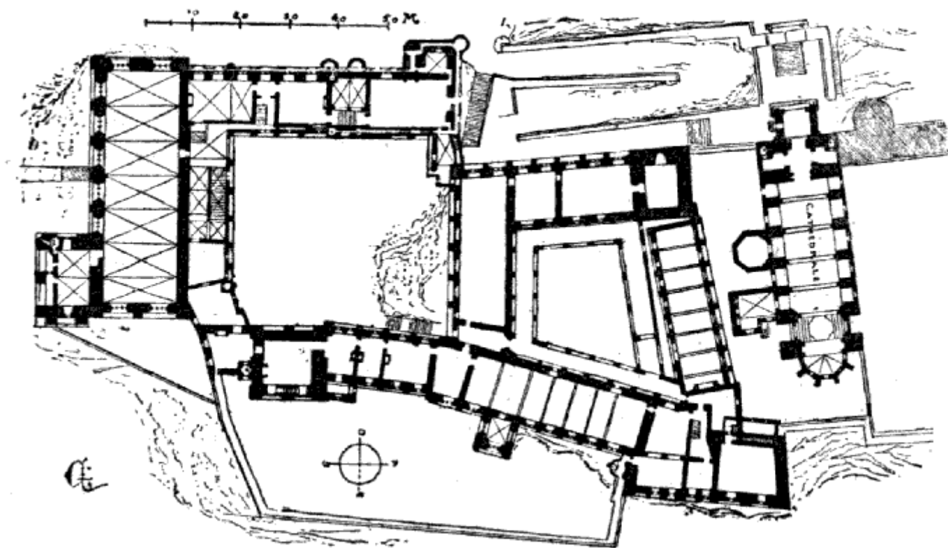
235. PALACE OF THE POPES AT AVIGNON. PLAN
