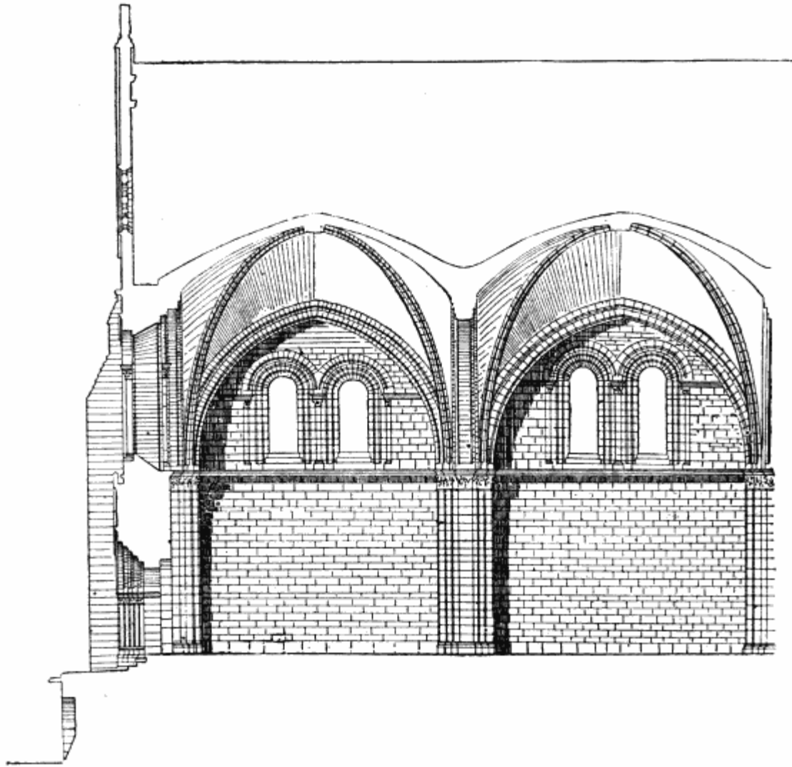
12. LONGITUDINAL SECTION OF TWO BAYS IN THE NAVE OF LA STE. TRINITÉ AT LAVAL
