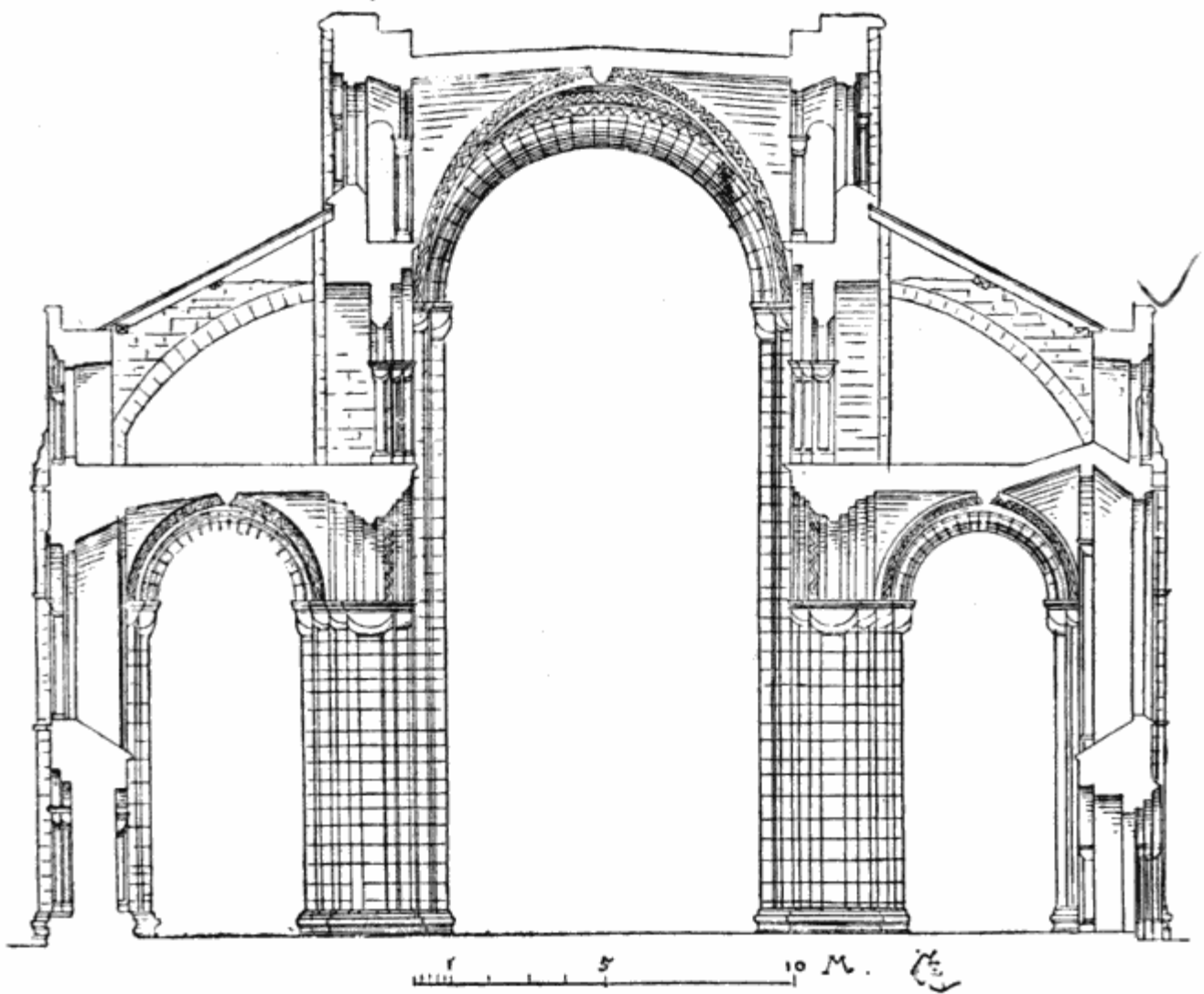
24. DURHAM CATHEDRAL. TRANSVERSE SECTIONS
