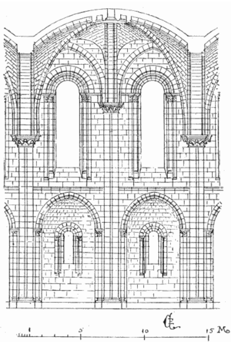
20. LONGITUDINAL SECTION OF A BAY OF LA STE. TRINITÉ AT ANGERS
