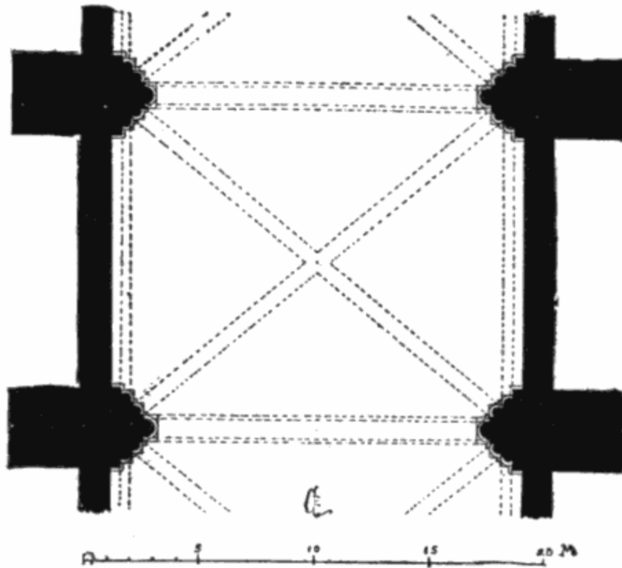
11. PLAN OF A BAY OF THE NAVE IN THE CHURCH OF LA STE. TRINITÉ AT LAVAL
