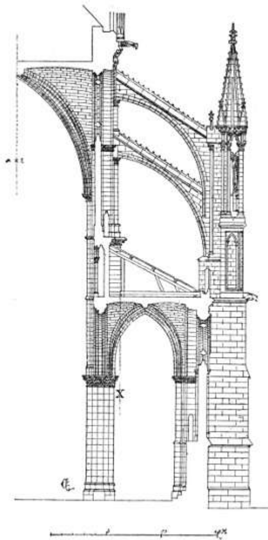
45. RHEIMS CATHEDRAL. SECTION OF THE NAVE
