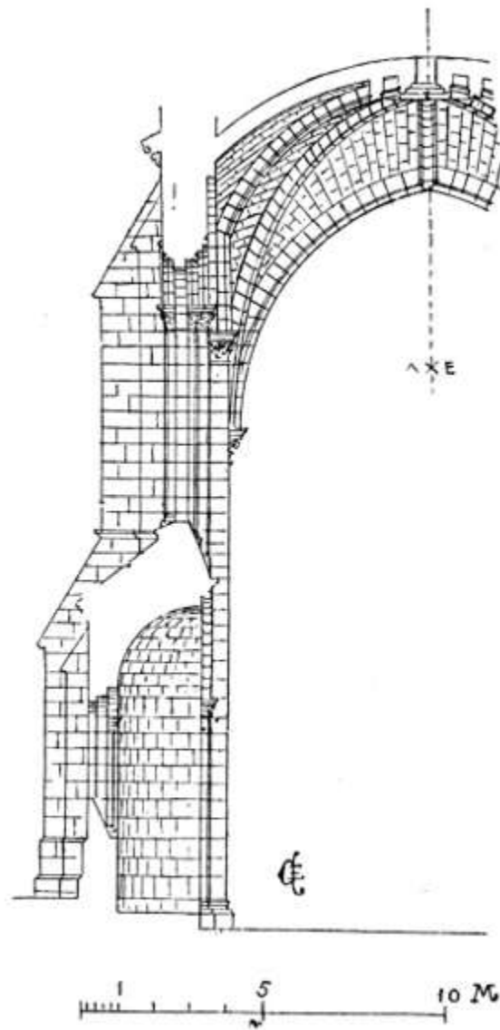
21. TRANSVERSE SECTION OF A BAY OF LA STE. TRINITÉ AT ANGERS
