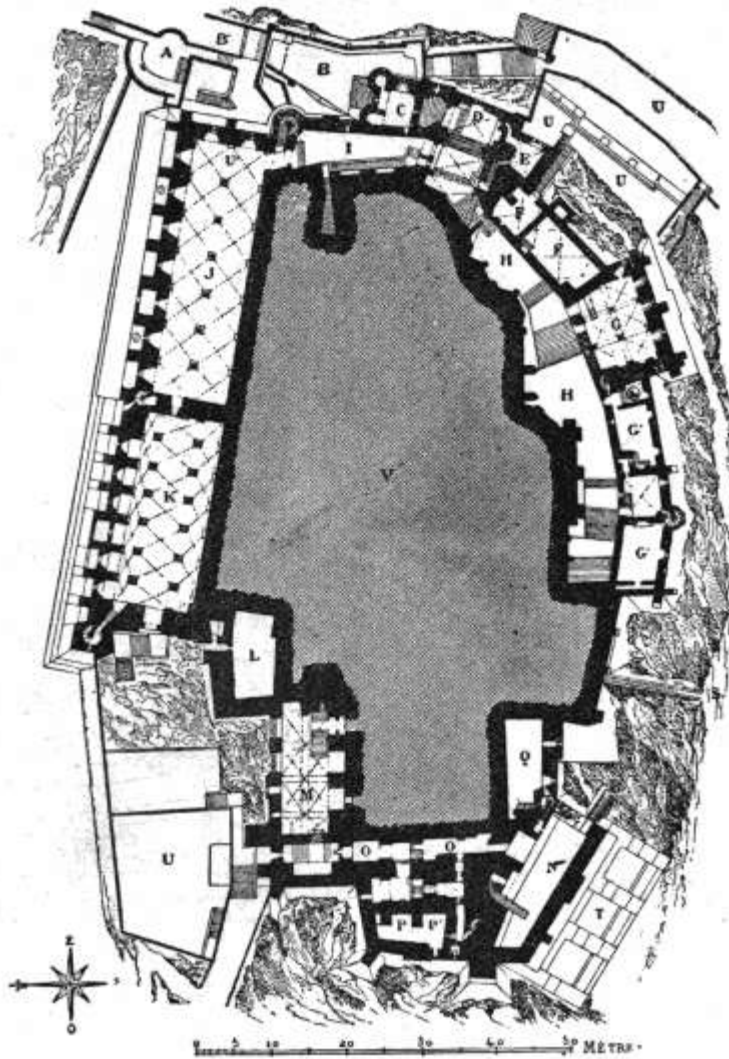
150. ABBEY OF MONT ST. MICHEL. PLAN AT THE LEVEL OF THE GUARD-ROOM, ALMONRY, AND CELLAR
