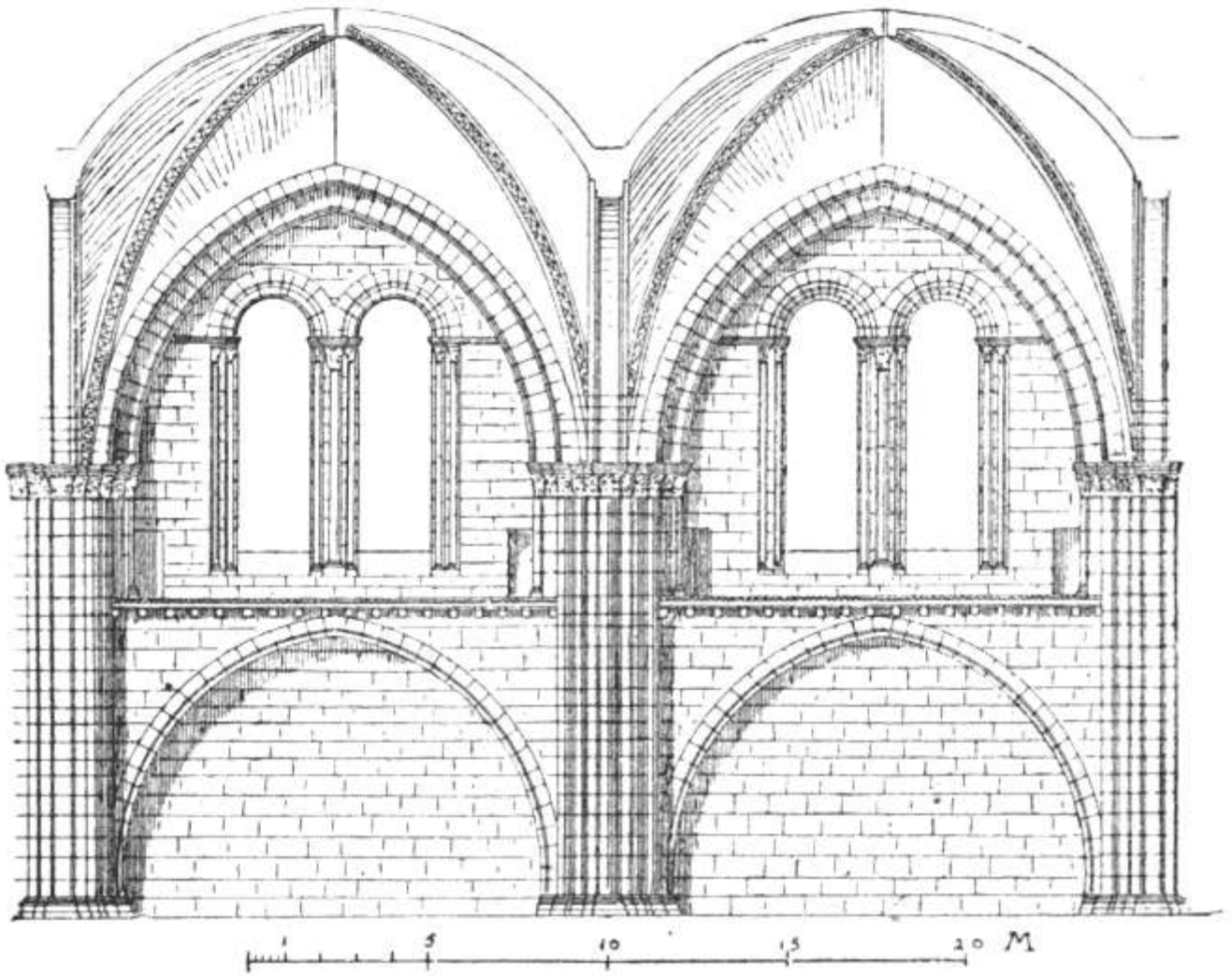
13 AND 14. COMPARATIVE SECTIONS OF THE CHURCHES OF ANGOULÊME AND ANGERS
