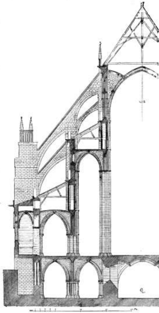
43. BOURGES CATHEDRAL. SECTION OF THE NAVE
