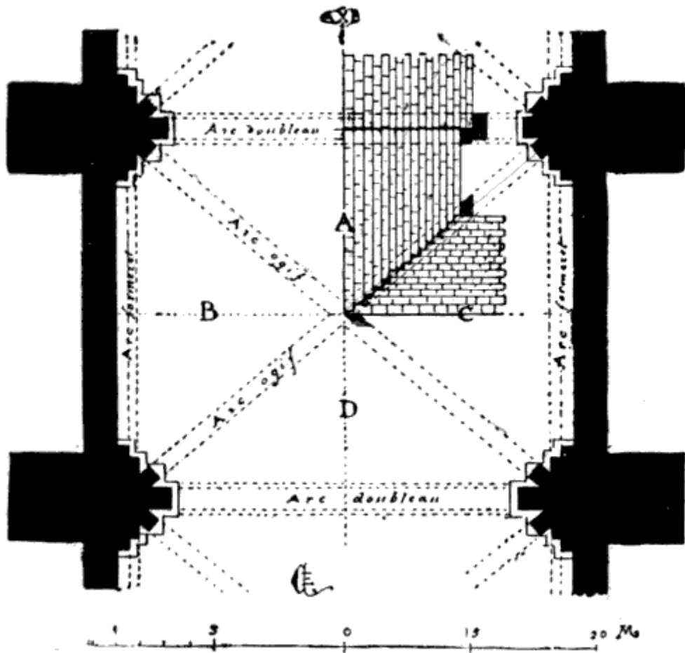
7. PLAN OF VAULT ON INTERSECTING ARCHES
