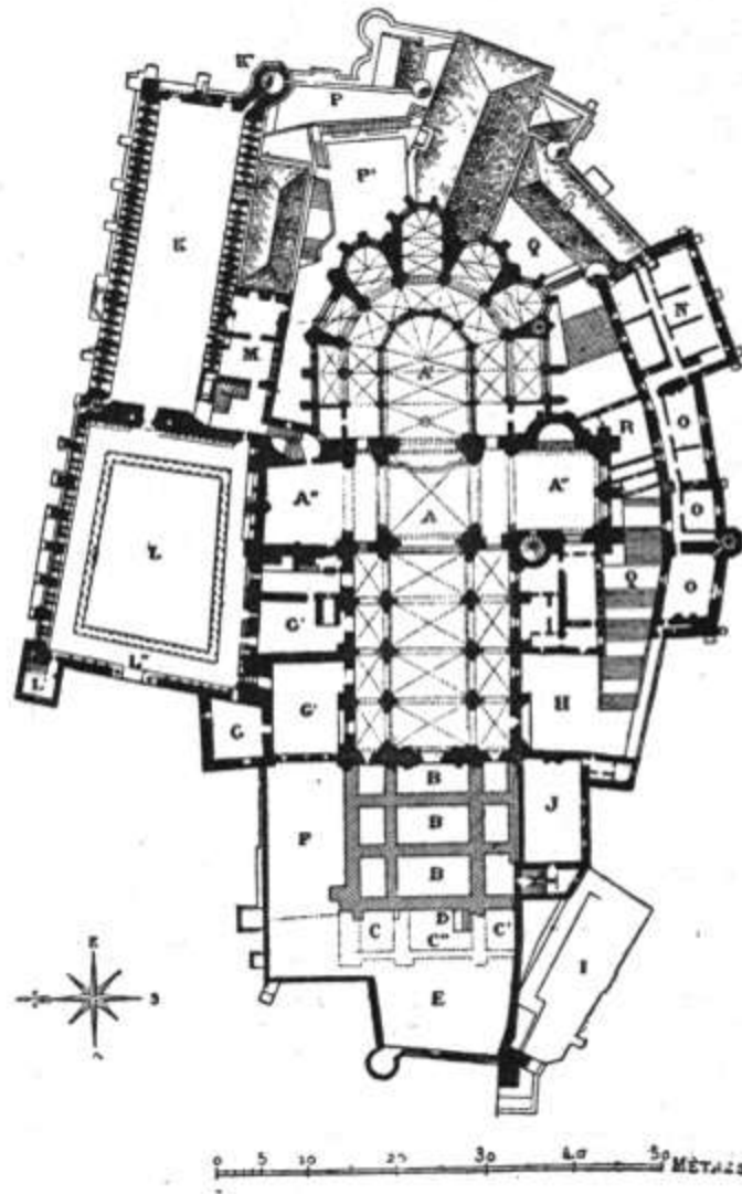
152. ABBEY OF MONT ST. MICHEL. PLAN AT THE LEVEL OF THE UPPER CHURCH, THE CLOISTERS, AND THE DORMITORY
