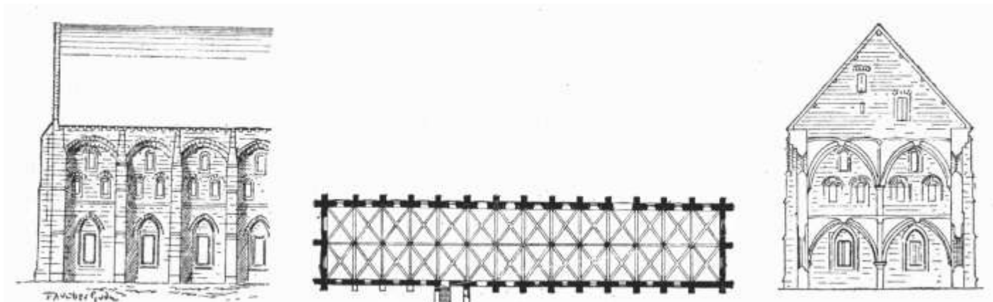
203. GRANARY OF THE ABBEY OF VAUCLAIR
