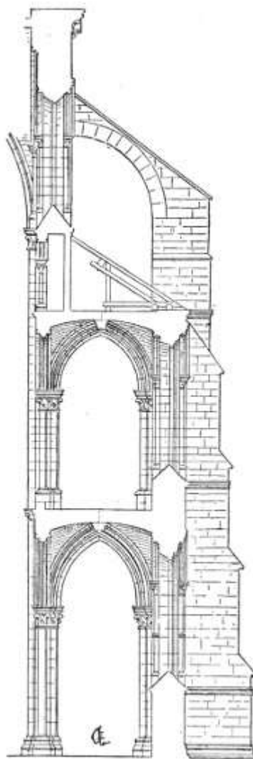
30. SOISSONS CATHEDRAL. SOUTH TRANSEPT. SECTION OF FLYING BUTTRESS
