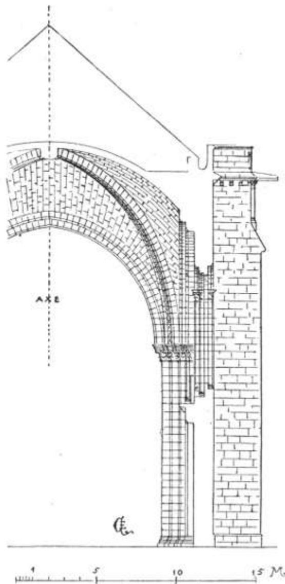
22. SECTION OF A SINGLE-AISLED CHURCH VAULTED ON INTERSECTING ARCHES WITH BUTTRESSES
