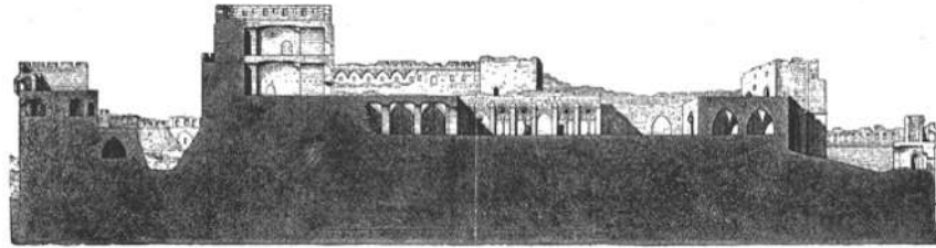
166. FORTRESS OF KALAAT-EL-HOSN IN SYRIA (KRAK OF THE KNIGHTS). SECTION, AS RESTORED BY M. G. REY
