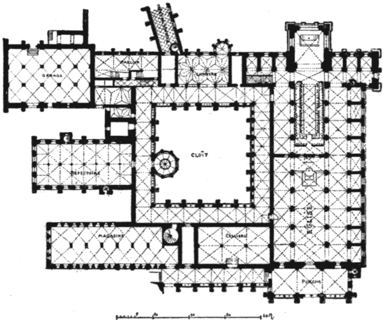
141. CISTERCIAN ABBEY OF MAULBRONN (WURTEMBERG). PLAN
