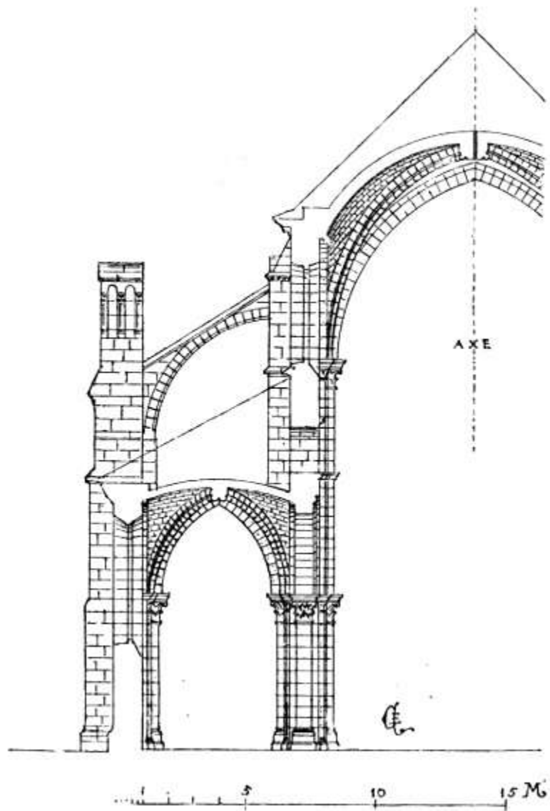
23. SECTION OF A THREE-AISLED CHURCH VAULTED ON INTERSECTING ARCHES WITH FLYING BUTTRESSES
