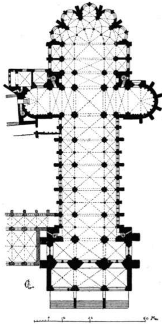
25. ABBEY CHURCH AT NOYON. PLAN
