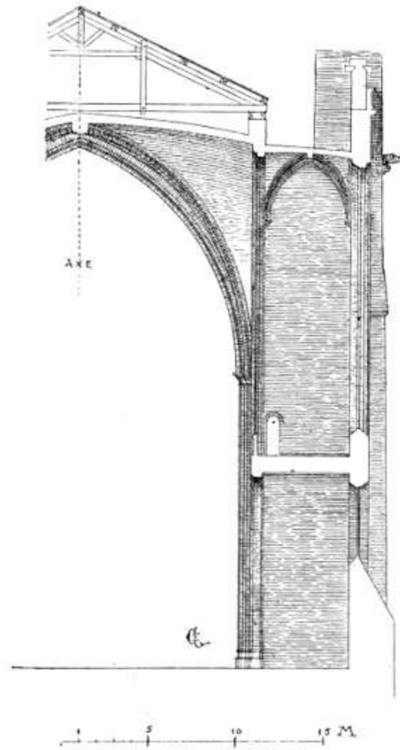
71. ALBI CATHEDRAL. SECTION OF THE NAVE
