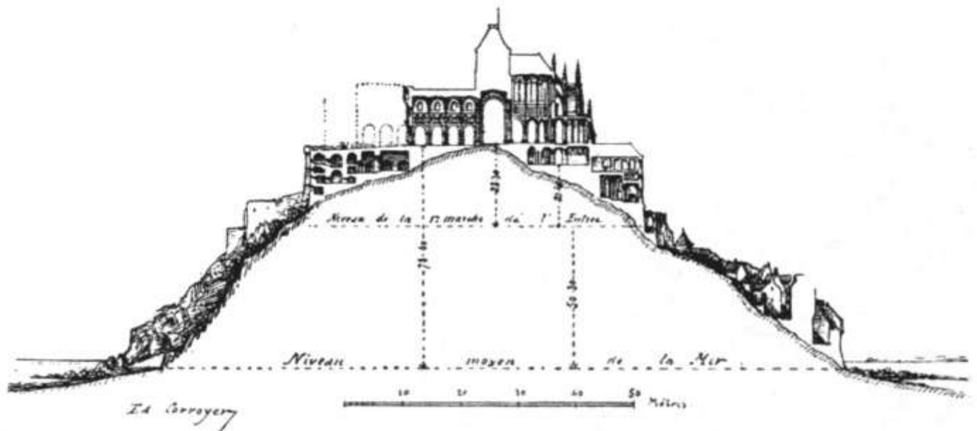
154. ABBEY OF MONT ST. MICHEL. LONGITUDINAL SECTION, FROM WEST TO EAST
