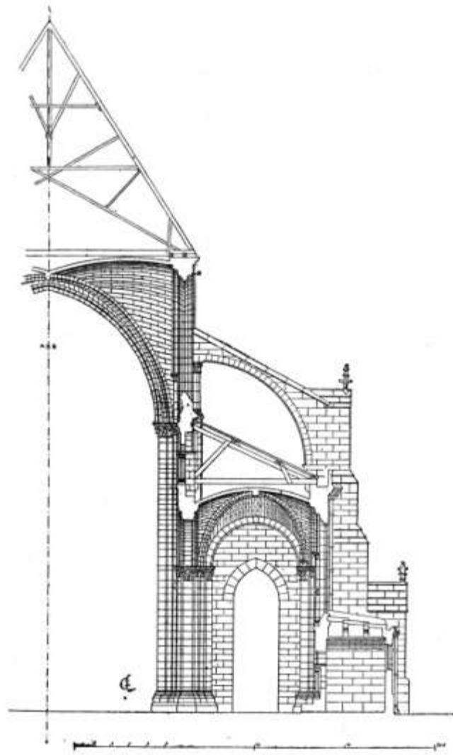
41. SENS CATHEDRAL. SECTION OF A BAY OF THE NAVE
