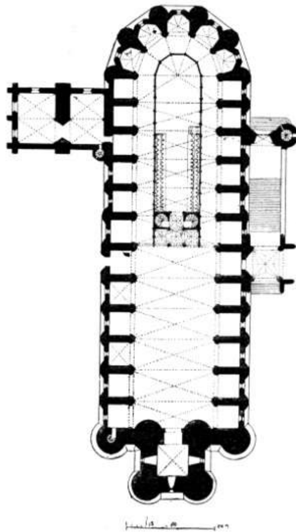
70. ALBI CATHEDRAL. PLAN
