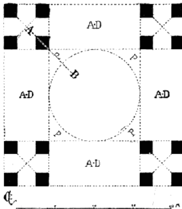
1. PLAN OF A CUPOLA OF THE ABBEY CHURCH OF ST. FRONT AT PÉRIGUEUX
