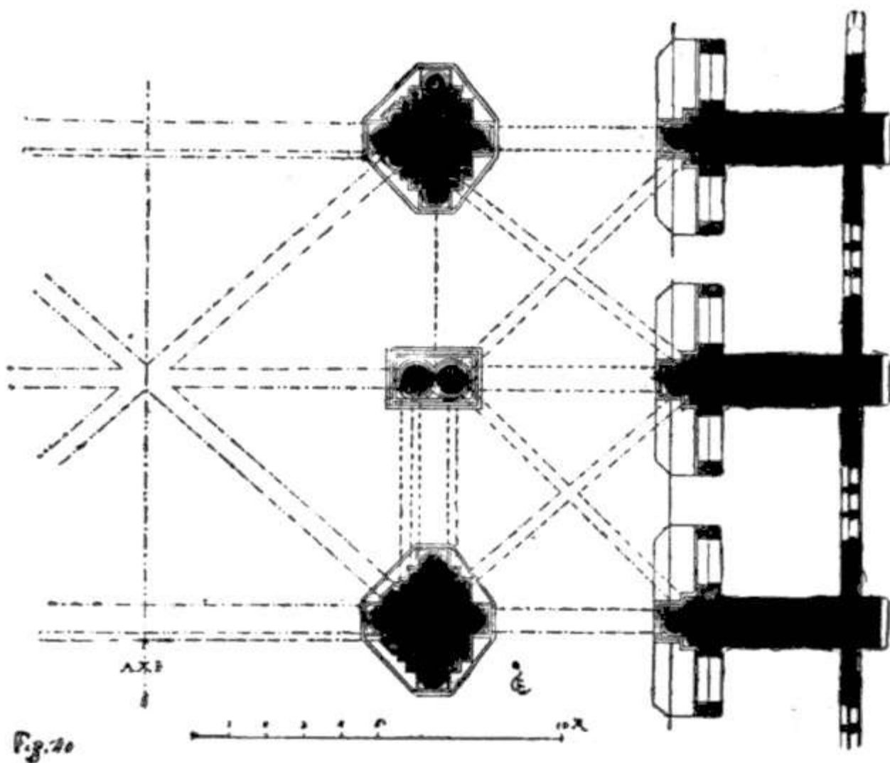
40. SENS CATHEDRAL. PLAN OF A BAY. VAULT IN SQUARE COMPARTMENTS OF TWO BAYS
