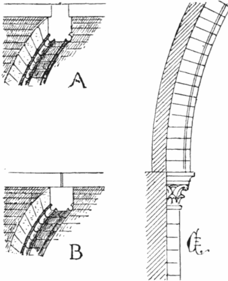
8. SECTION OF AN INTERSECTING ARCH
