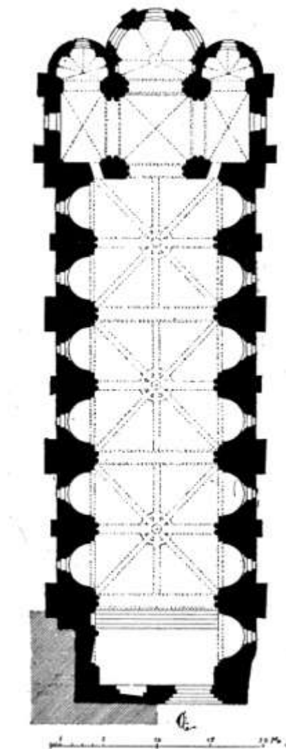
19. PLAN OF THE CHURCH OF LA STE. TRINITÉ AT ANGERS
