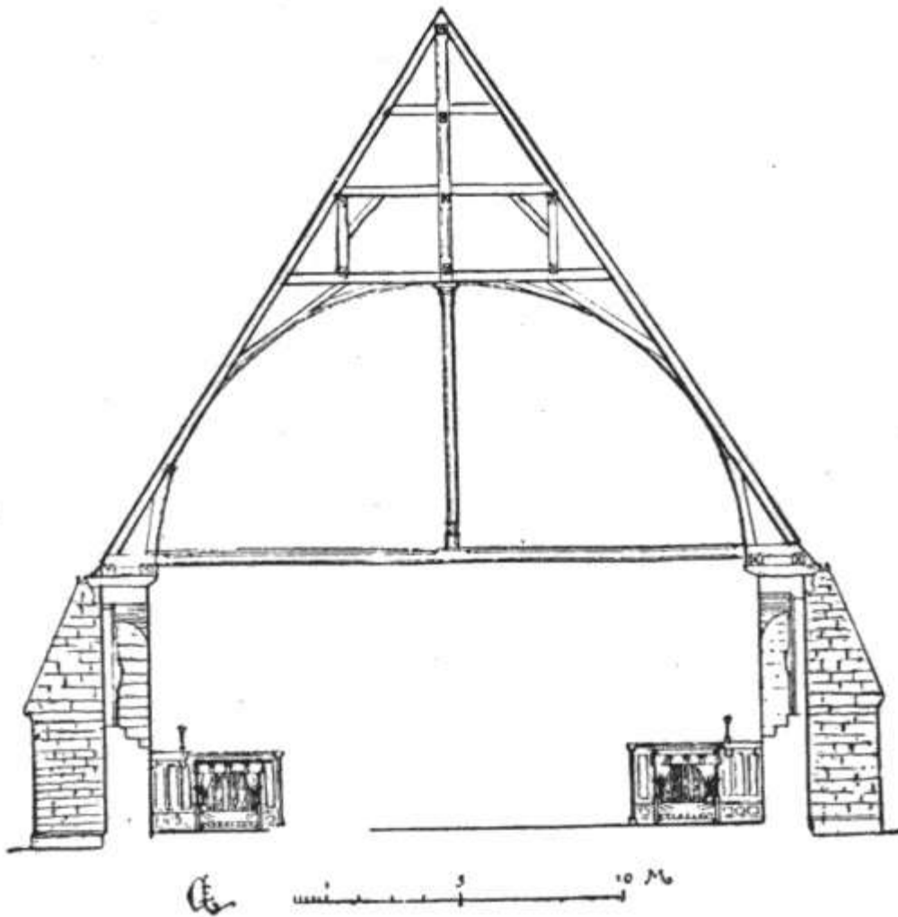
207. HOSPITAL AT TONNERRE. SECTION OF THE GREAT HALL
