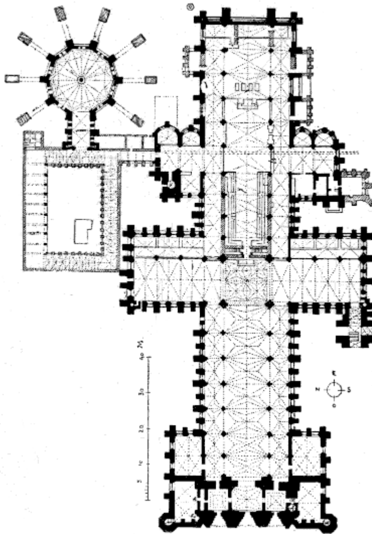
60. LINCOLN CATHEDRAL. PLAN
