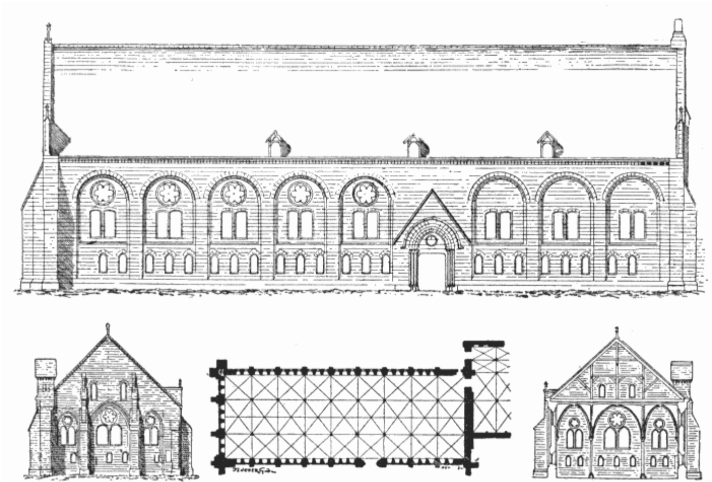
205. ABBEY OF OURSCAMPS (OISE, THIRTEENTH CENTURY). HOSPITAL. AS RESTORED BY A. VERDIER
