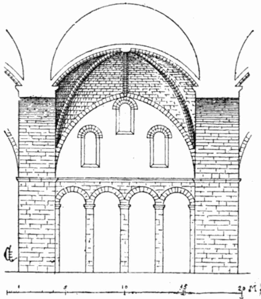
6. SECTION OF A BAY IN THE CHURCH OF ST. AVIT-SÉNIEUR
