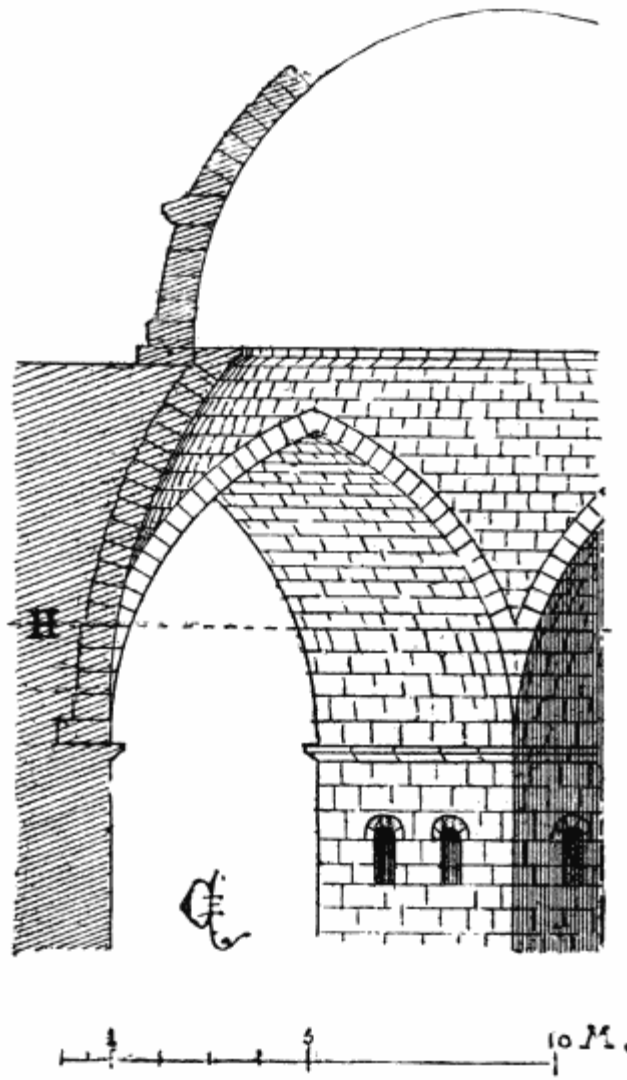
3. SECTION OF A PENDENTIVE ON THE DIAGONAL A TO B IN PLAN, FIG.
