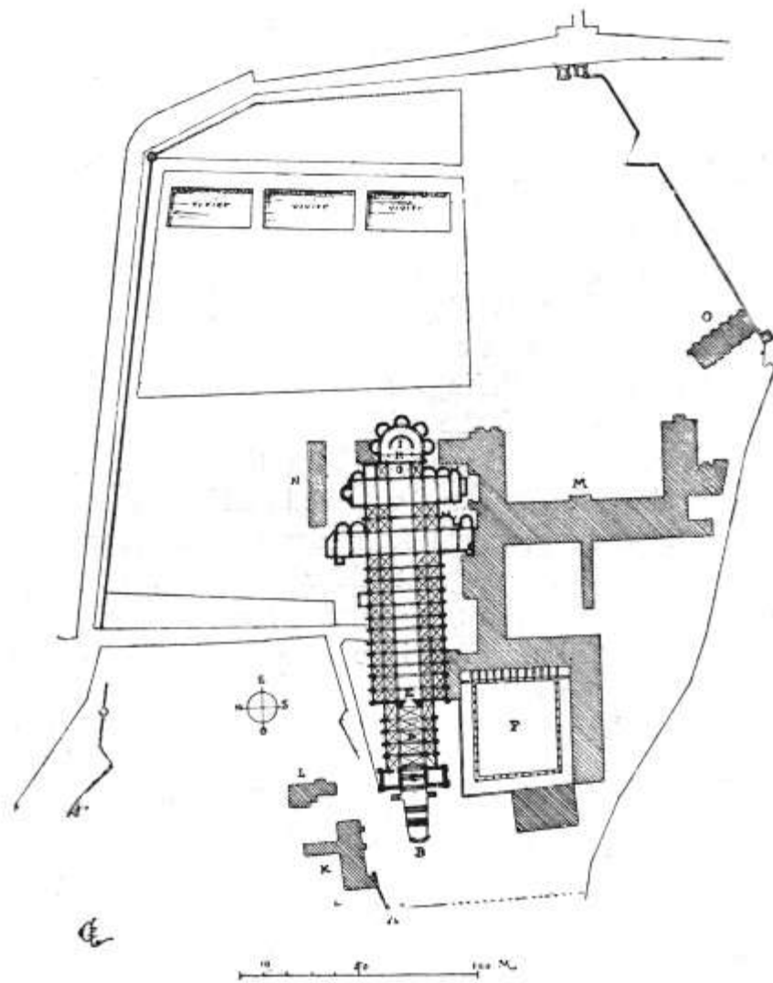
134. ABBEY OF CLUNY. PLAN
