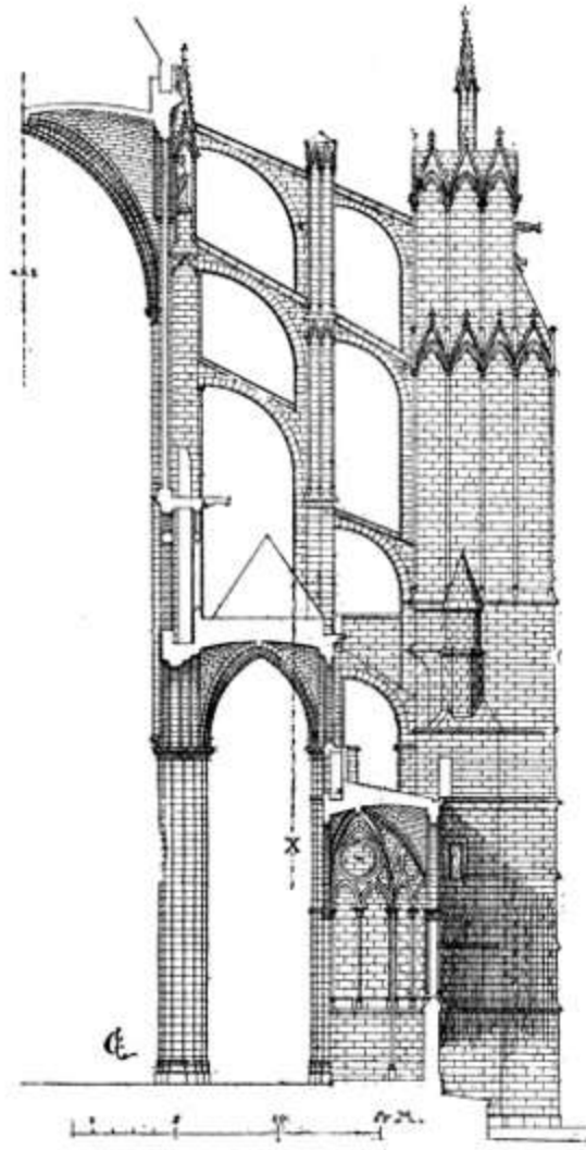
51. BEAUVAIS CATHEDRAL. TRANSVERSE SECTION
