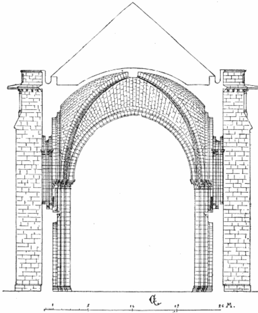
10. TRANSVERSE SECTION OF THE NAVE OF ST. MAURICE AT ANGERS
