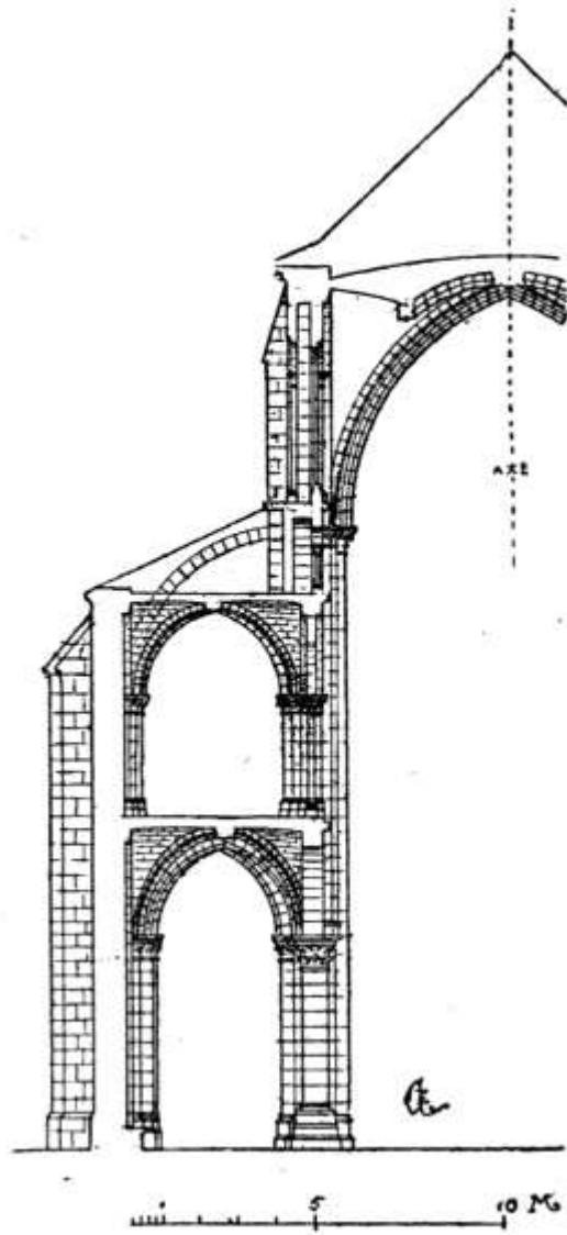
26. TRANSVERSE SECTION OF NOYON CHURCH
