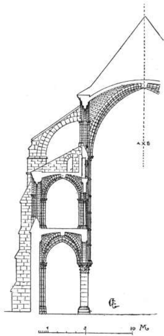
36. CATHEDRAL OF LAON. SECTION OF THE NAVE
