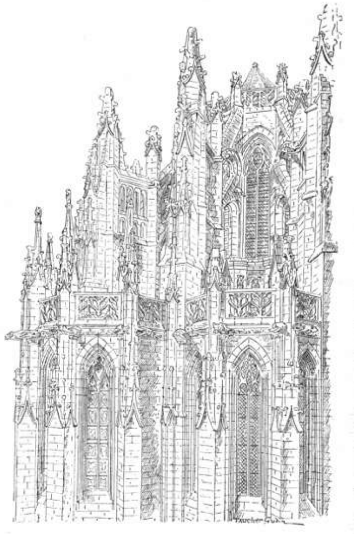
77. ABBEY OF MONT ST. MICHEL. DETAILS OF THE APSE (LATE FIFTEENTH CENTURY)
