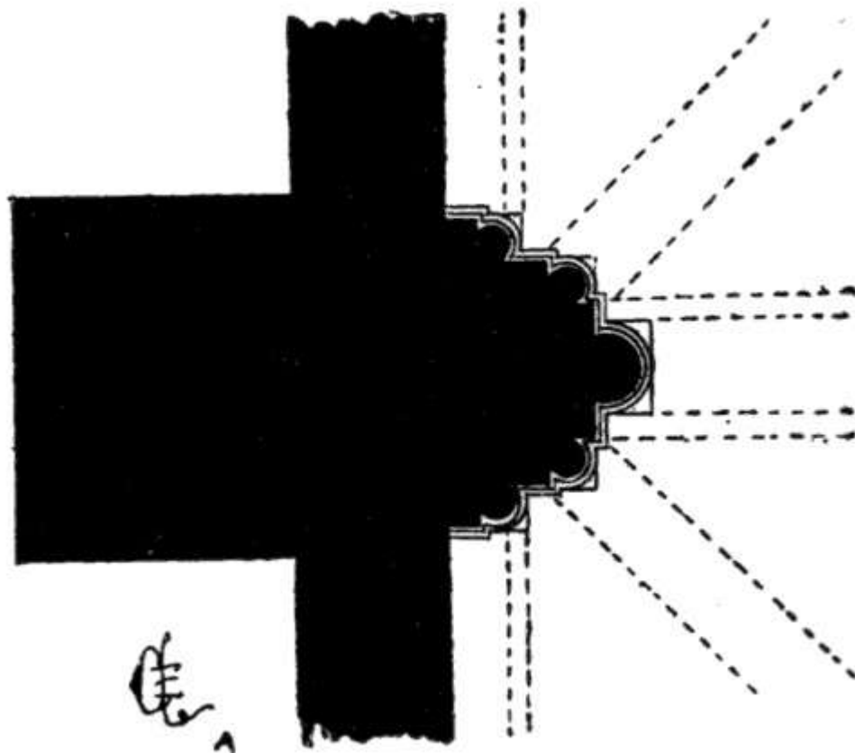
17. PLAN OF ONE OF THE PIERS OF THE NAVE OF LA STE. TRINITÉ AT LAVAL
