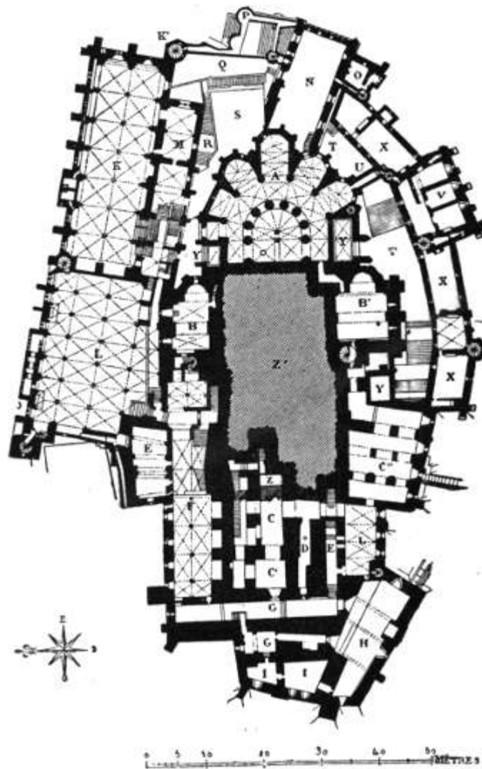
151. ABBEY OF MONT ST. MICHEL. PLAN AT THE LEVEL OF THE LOWER CHURCH, THE REFECTORY, AND THE CHAPTER-HOUSE, OR KNIGHTS' HALL.
