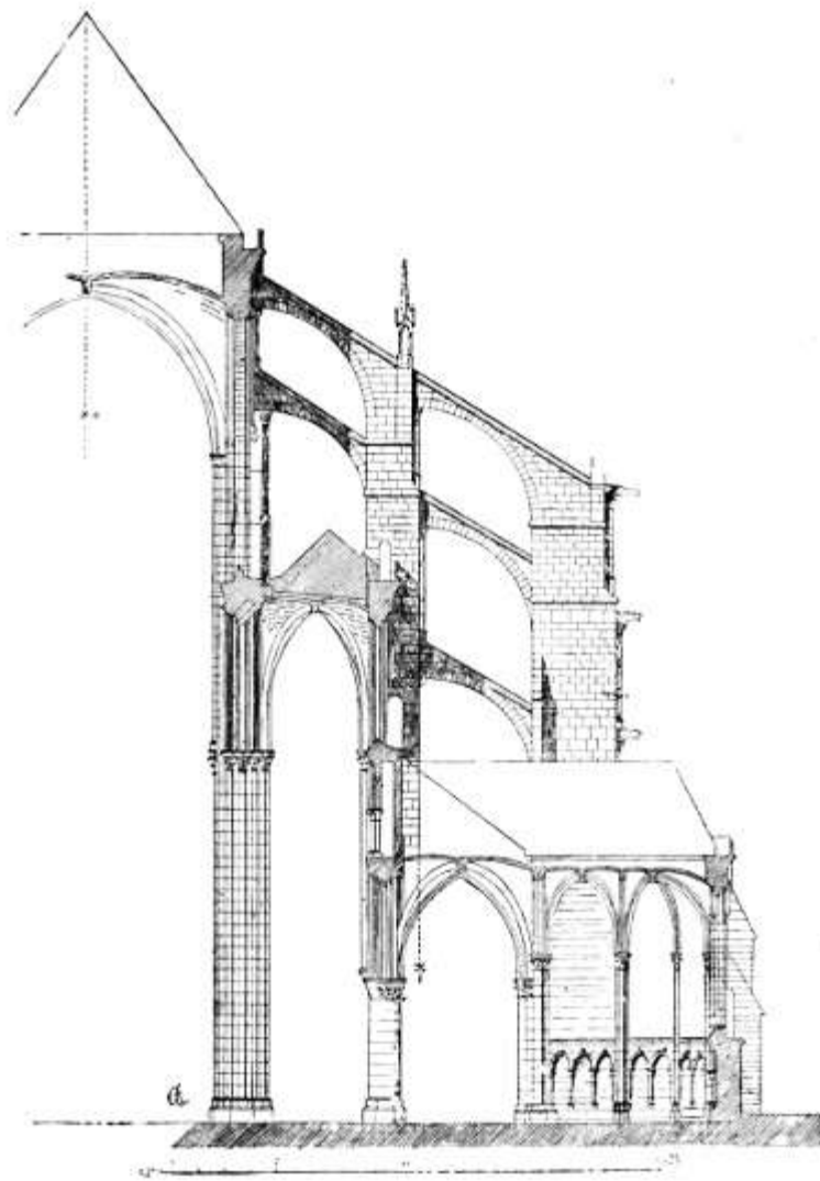
55. MANS CATHEDRAL. SECTION OF THE CHOIR
