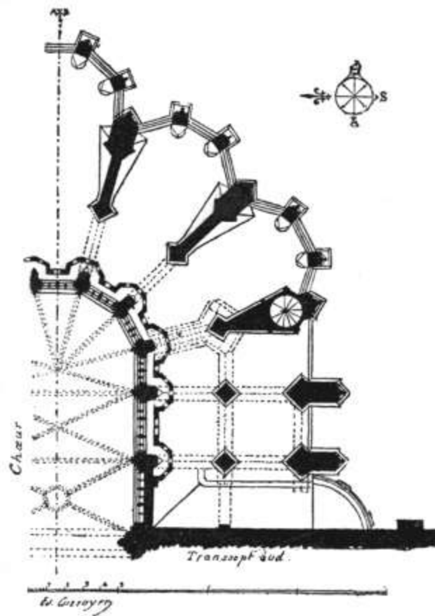
76. ABBEY OF MONT ST. MICHEL. PLAN OF THE CHOIR ABOVE THE LOWER CHAPEL
