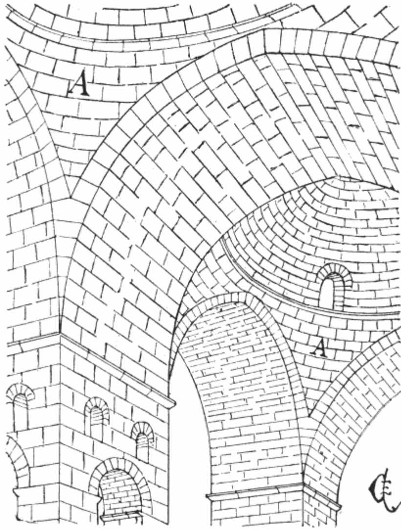
2. PENDENTIVE (MARKED A) OF A CUPOLA OF THE ABBEY CHURCH OF ST. FRONT
