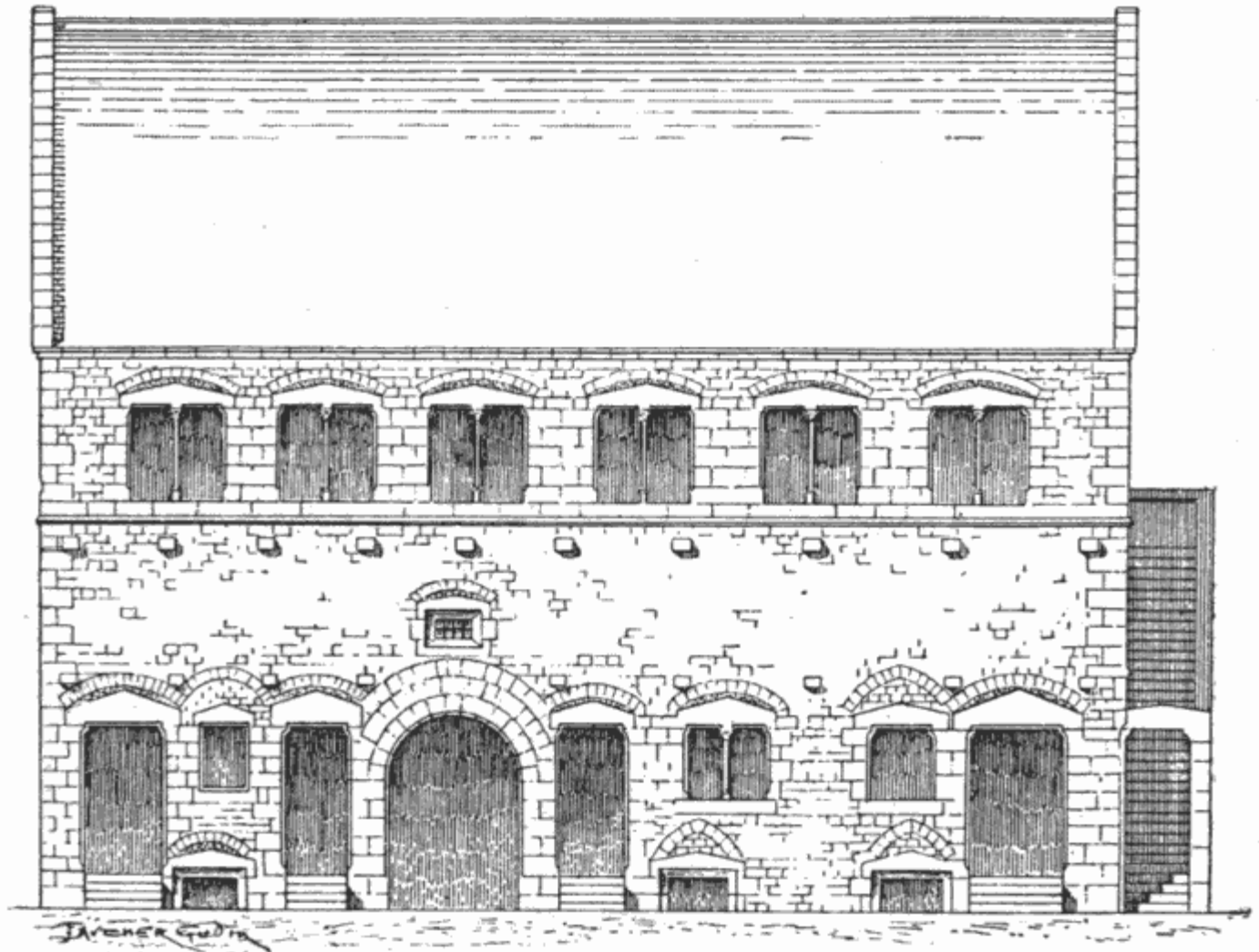
202. TITHE-BARN AT PROVINS
