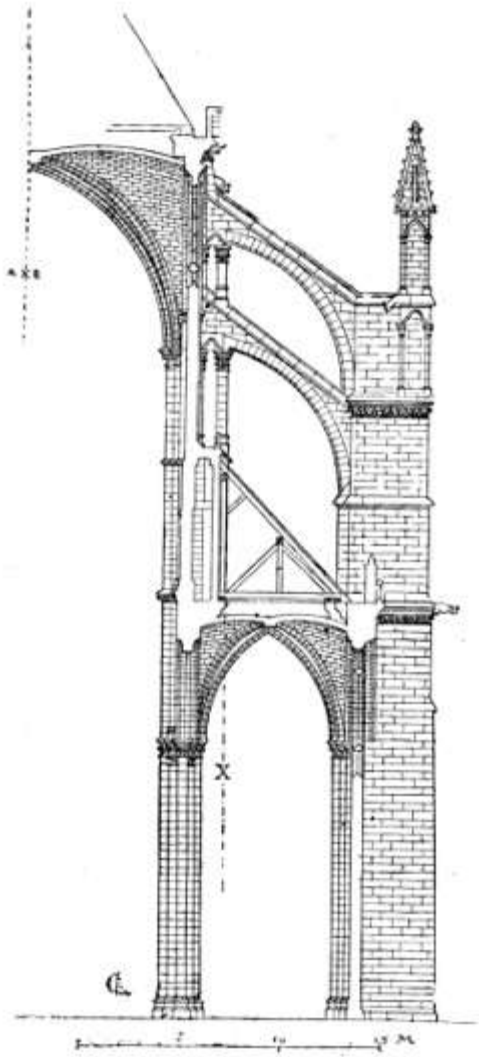
48. AMIENS CATHEDRAL. SECTION THROUGH THE NAVE
