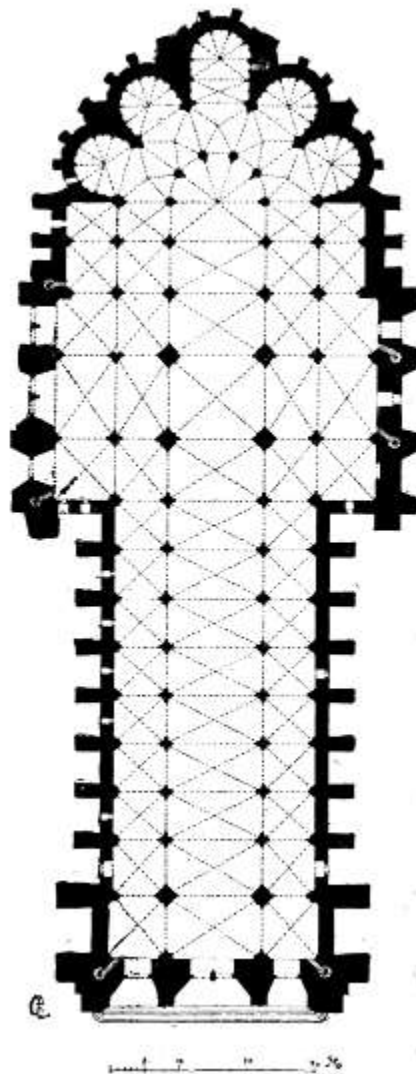
44. RHEIMS CATHEDRAL. PLAN
