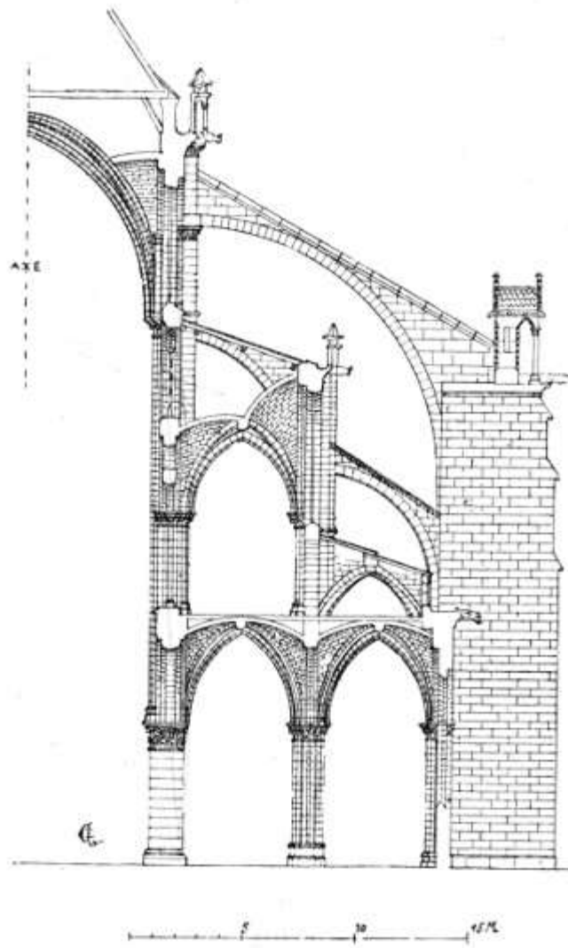
38. NOTRE DAME DE PARIS. SECTION OF THE NAVE
