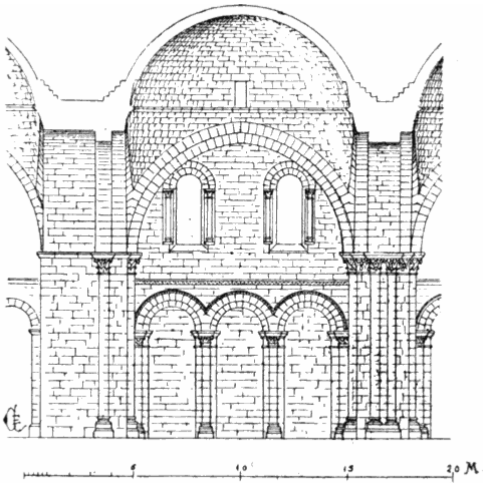
5. SECTION OF A BAY OF THE CUPOLAS OF ANGOULÊME
