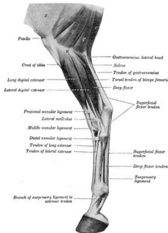
Fig. 42—Muscles of lower part of thigh, leg and foot; lateral view, o', Fascia lata; q, q', q", biceps femoris; r, semitendinosus; 21', lateral condyle of tibia. The extensor brevis is visible in the angle between the long and lateral extensor tendons. (After Ellenberger-Baum, Anat. für Künstler.) (From Sisson's "Anatomy of the Domestic Animals.")
