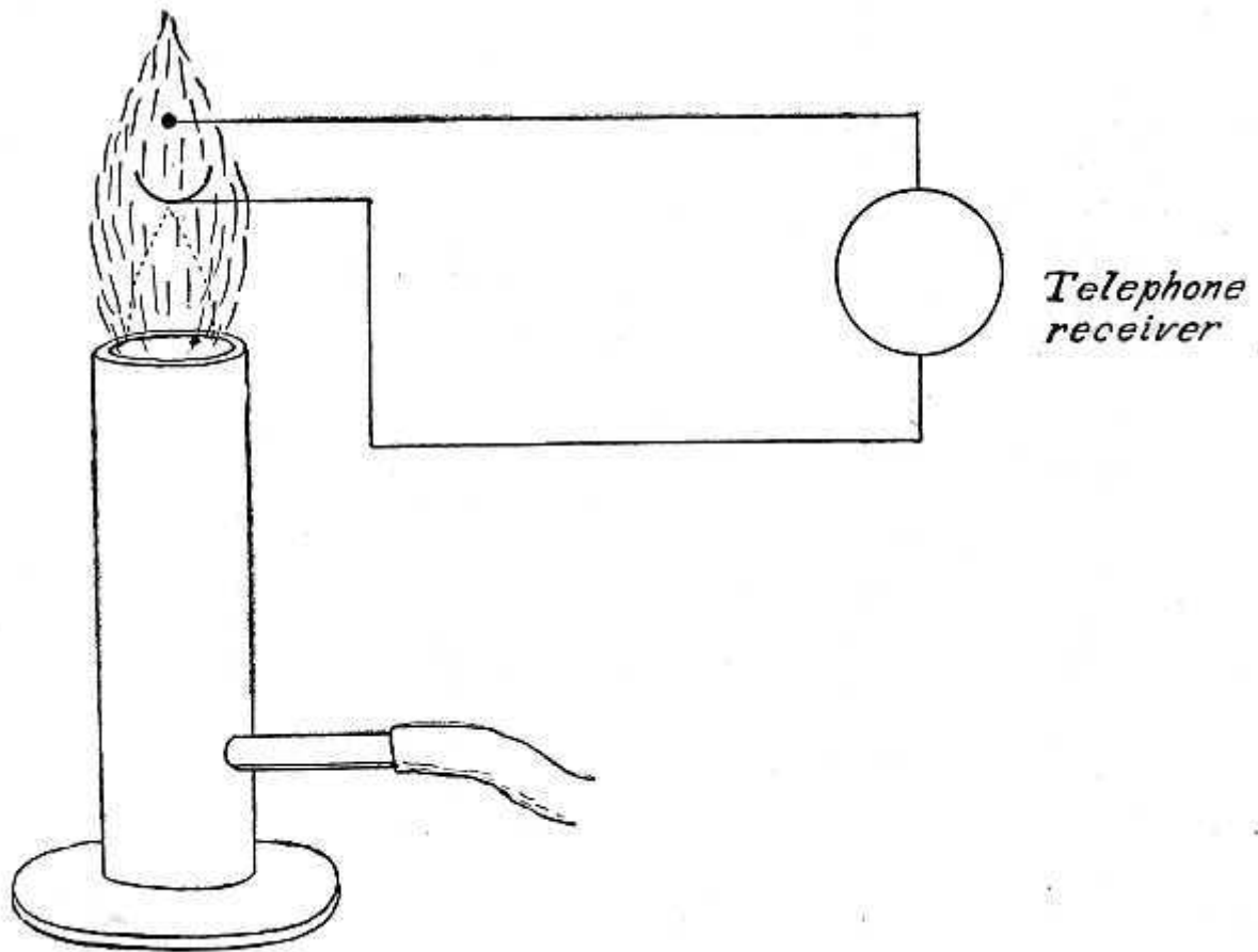
FIG. 112—A GAS FLAME IS SENSITIVE TO ELECTRIC WAVES
