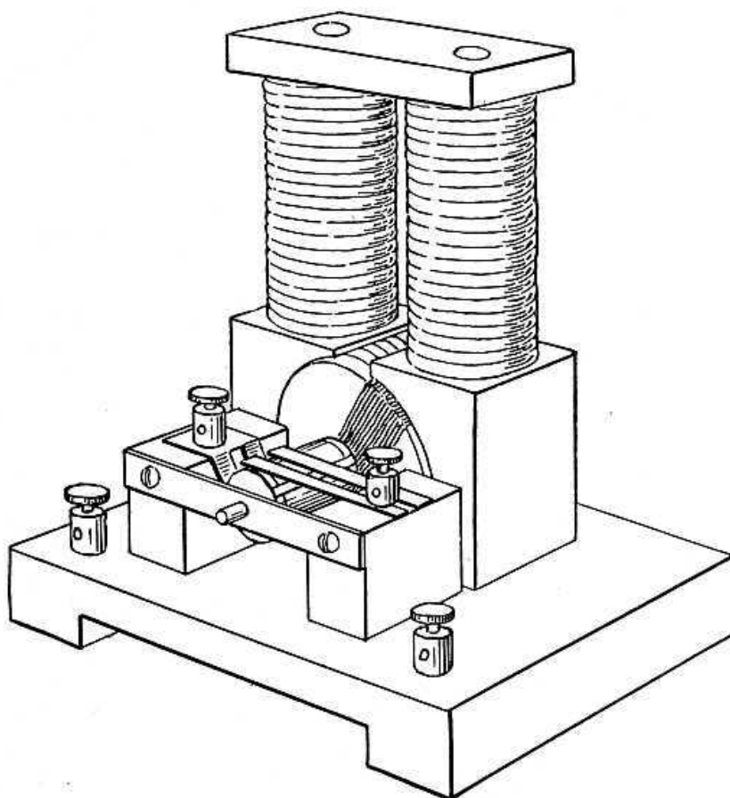
FIG. 45—A DYNAMO WITH SIEMENS' ARMATURE
