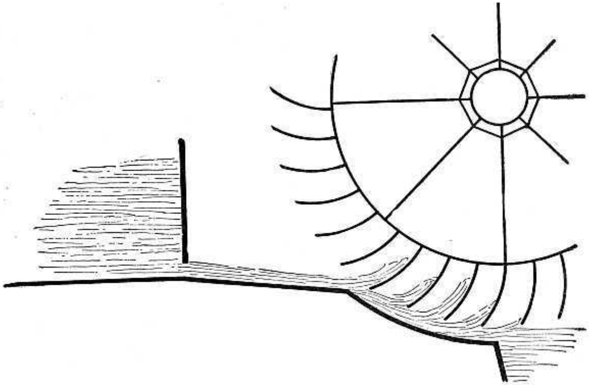
FIG. 83—AN UNDERSHOT WATER-WHEEL WITH CURVED BLADES
