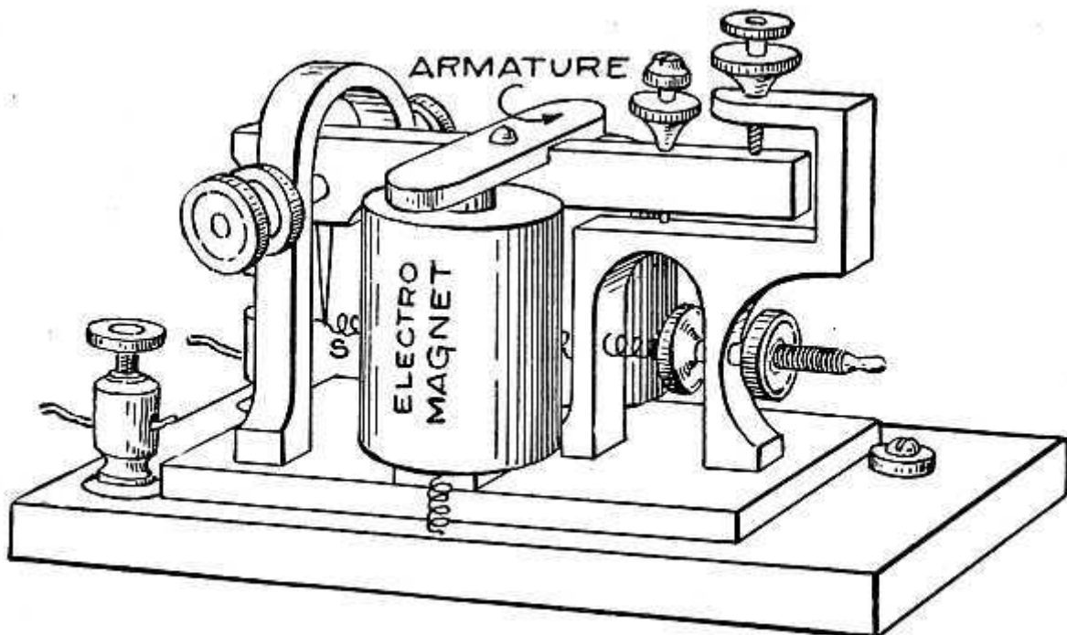
FIG. 61—A TELEGRAPH SOUNDER
