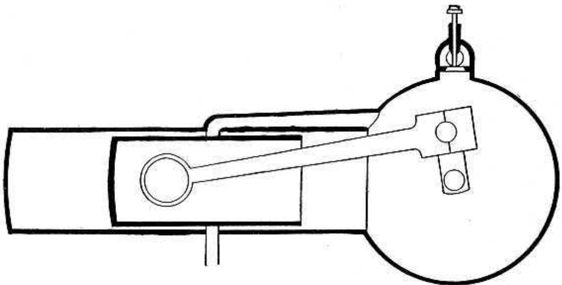
FIG. 78—TWO-CYCLE GAS-ENGINE. CRANK AND CONNECTING-ROD ARE ENCLOSED WITH THE PISTON
