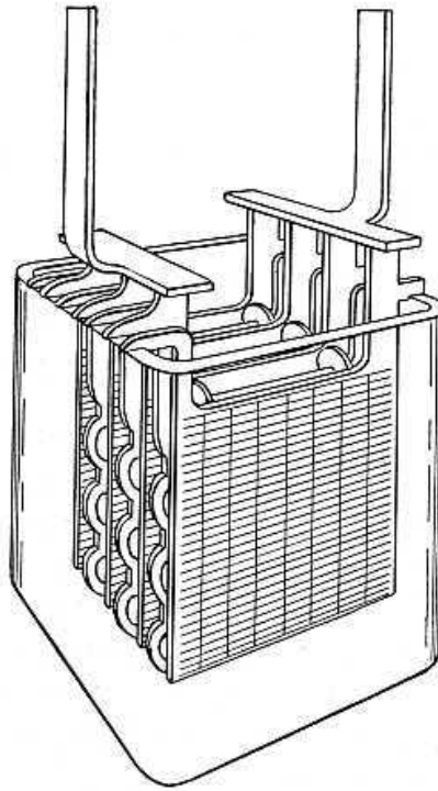
FIG. 40—A STORAGE BATTERY, SHOW- ING THE "GRIDS"
