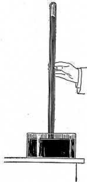
FIG. 4—TORRICELLI'S EXPERIMENT
