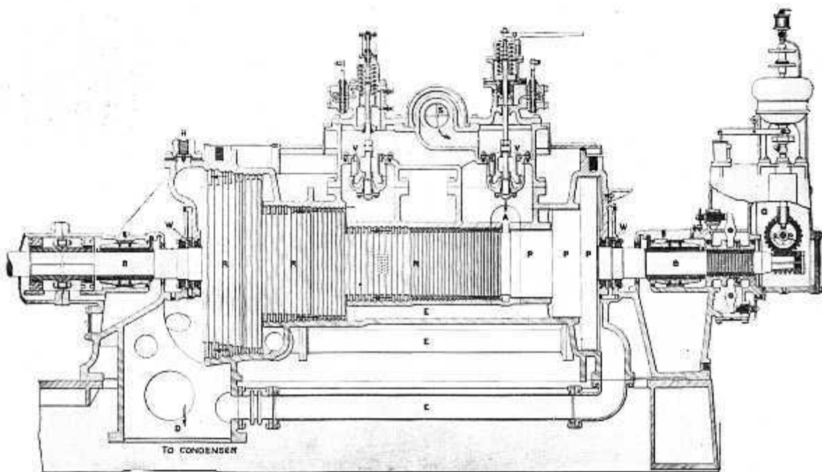
FIG. 87—DIAGRAM OF TURBINE SHOWN IN FIG. 86
