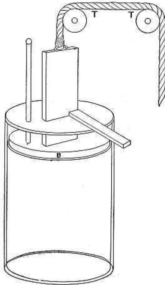
FIG. 12—PAPIN'S ENGINE
