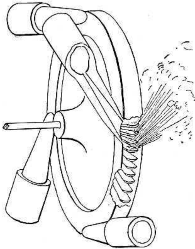
FIG. 85—DE LAVAL STEAM-TURBINE
