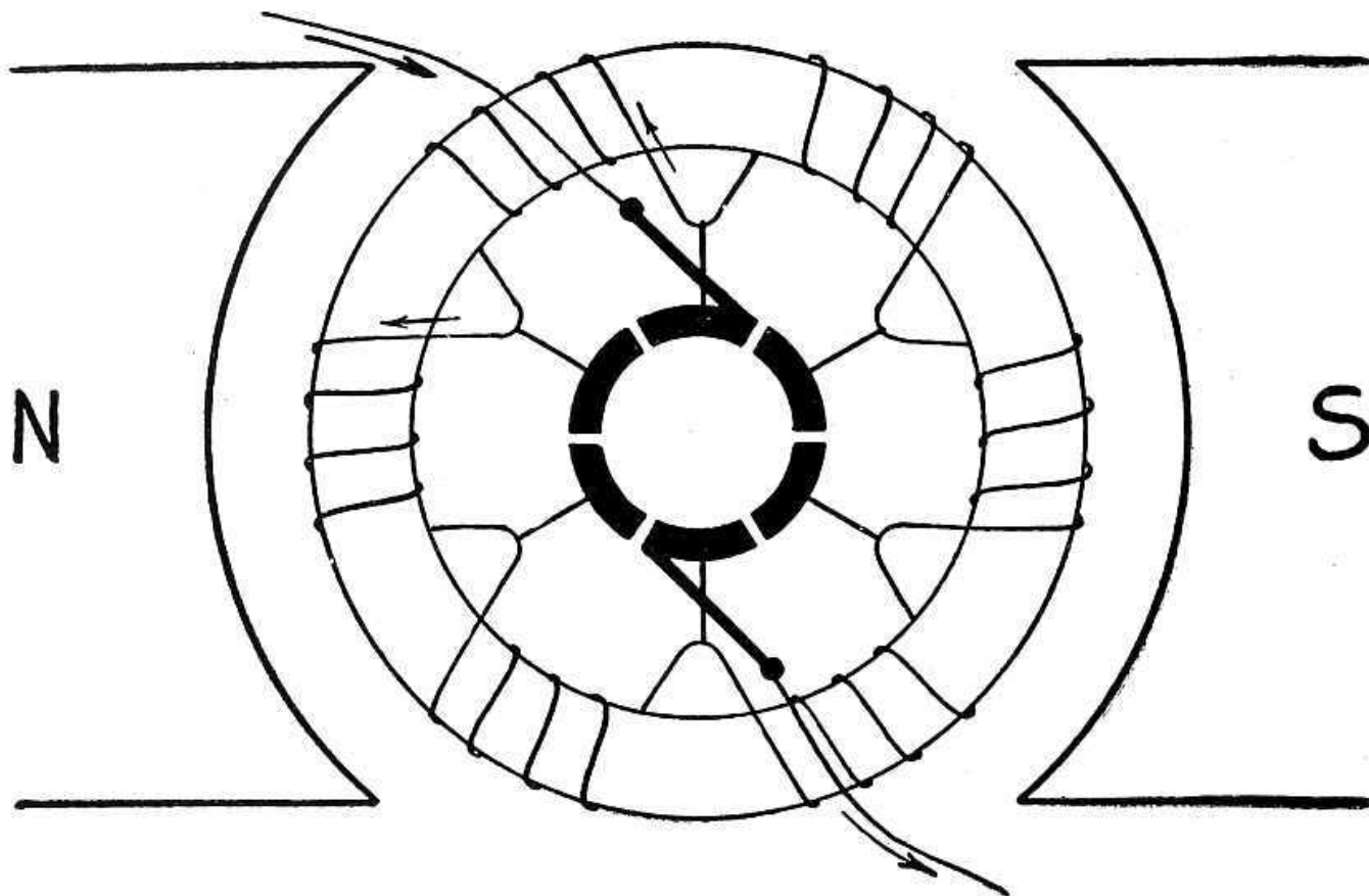
FIG. 46—RING ARMATURE
