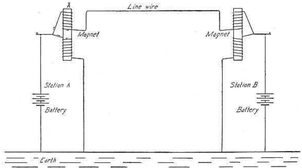
FIG. 66—HOW TWO MESSAGES ARE SENT OVER ONE WIRE AT THE SAME TIME
