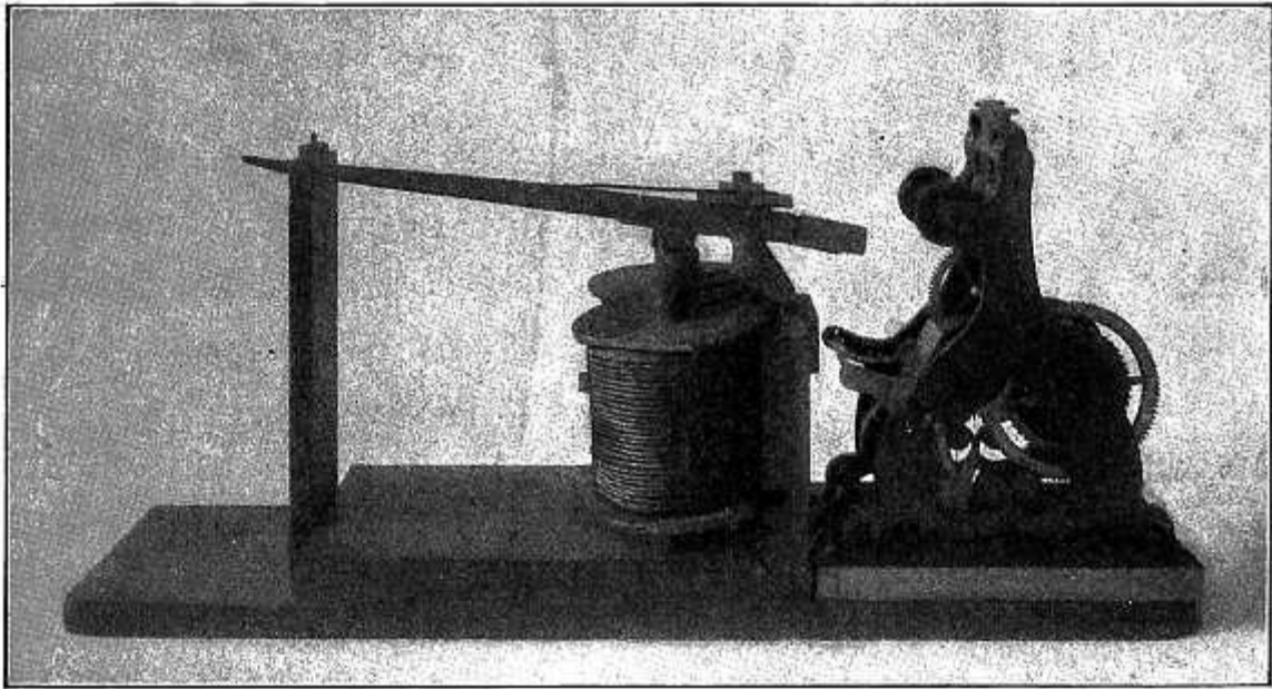
FIG. 65—FIRST TELEGRAPH INSTRUMENT USED FOR COMMERCIAL WORK
