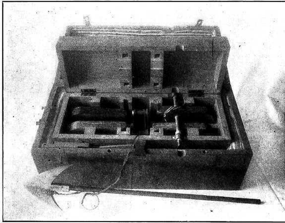
FIG. 47—FIRST DYNAMO PATENTED IN THE UNITED STATES FIG. 47—FIRST DYNAMO PATENTED IN THE UNITED STATES
