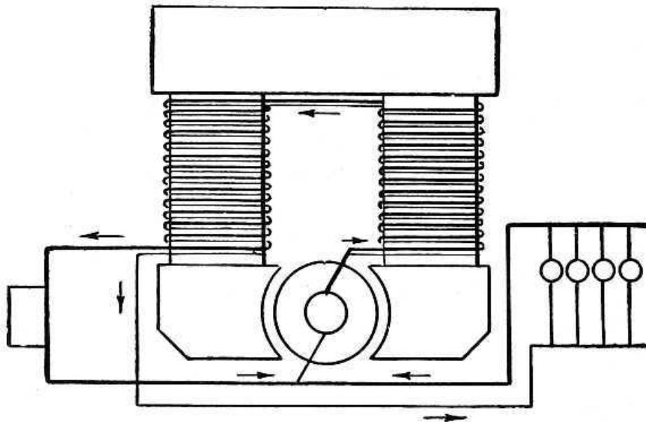
FIG. 51—A COMPOUND-WOUND DYNAMO
