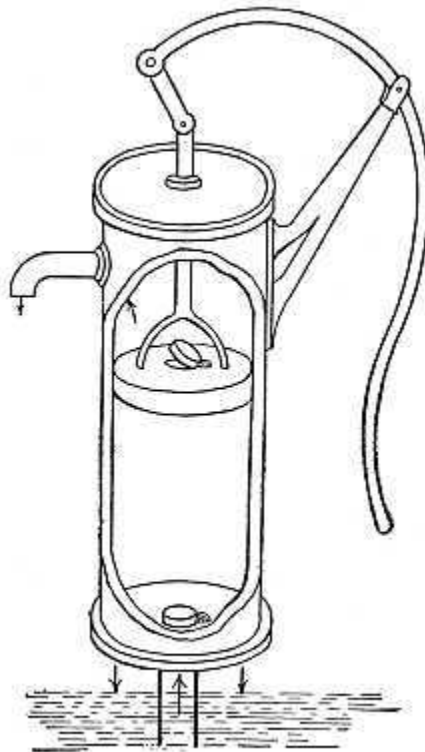
FIG. 7—A LIFT-PUMP
