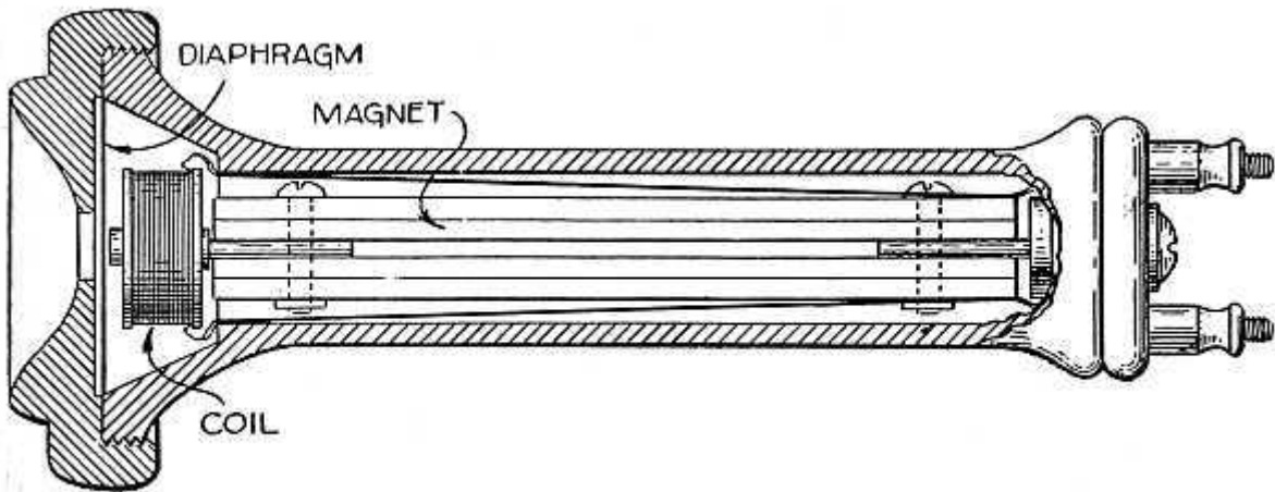
FIG. 69—A TELEPHONE RECEIVER
