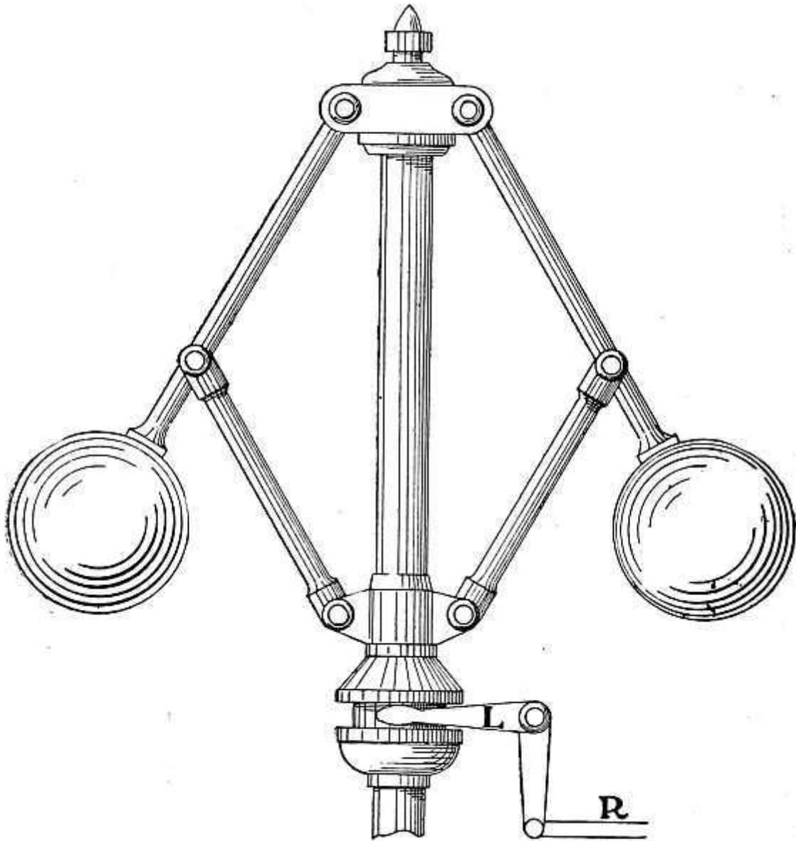
FIG. 15—A FLY-BALL GOVERNOR
