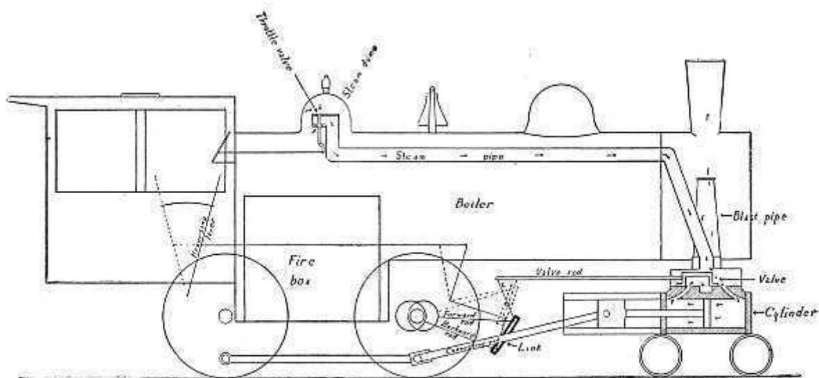
FIG. 81—HOW A LOCOMOTIVE WORKS
