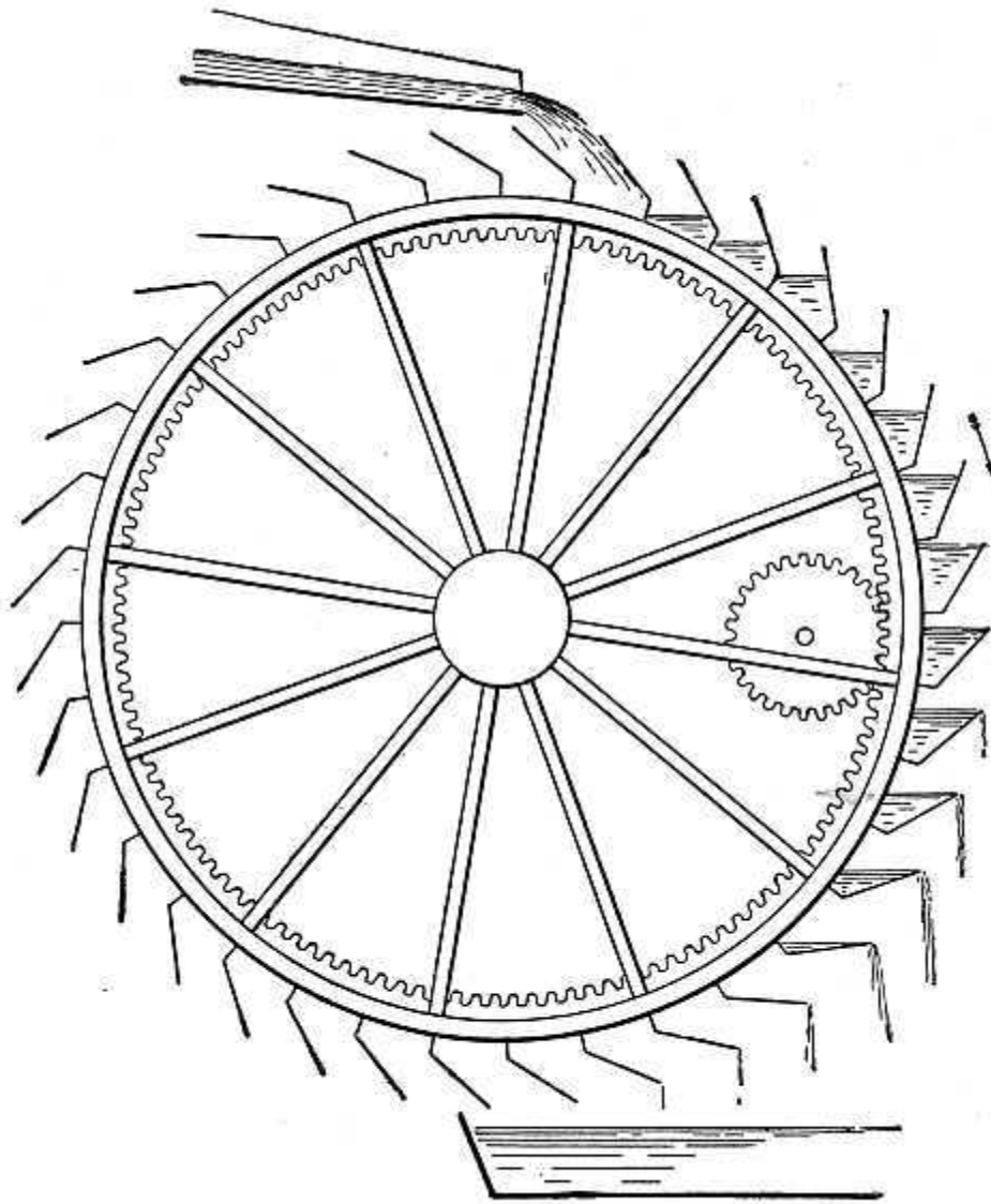
FIG. 84—AN OVERSHOT WATER-WHEEL
