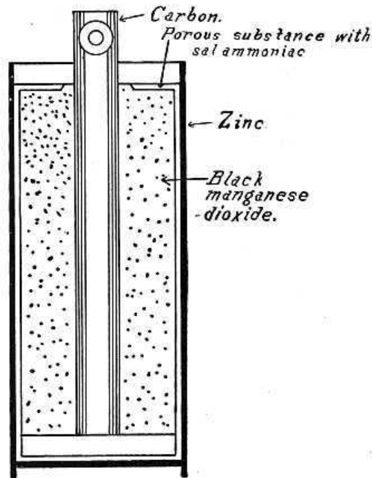
FIG. 39—SHOWING WHAT IS IN A DRY BATTERY
