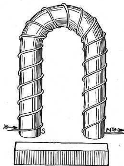
FIG. 42—STURGEON'S ELECTRO-MAGNET
