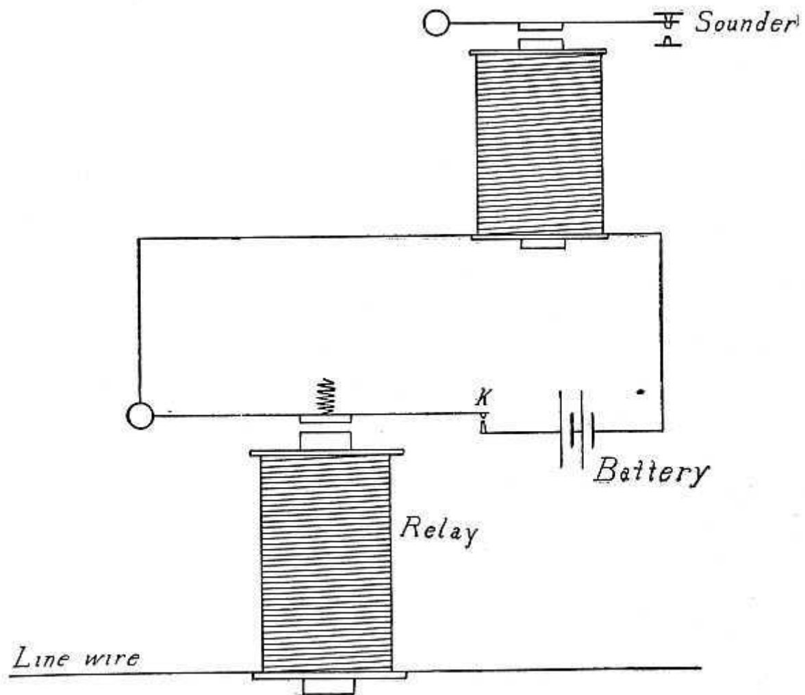
FIG. 63—A TELEGRAPHIC CIRCUIT WITH RELAY AND SOUNDER
