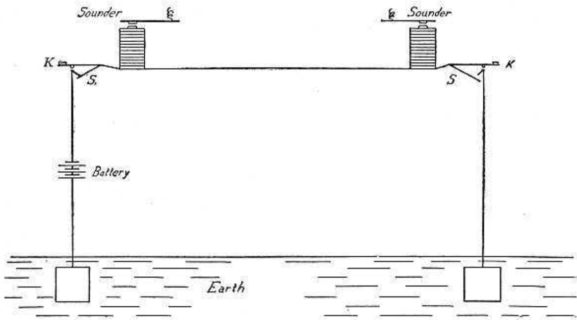
FIG. 64—A SIMPLE TELEGRAPHIC CIRCUIT
