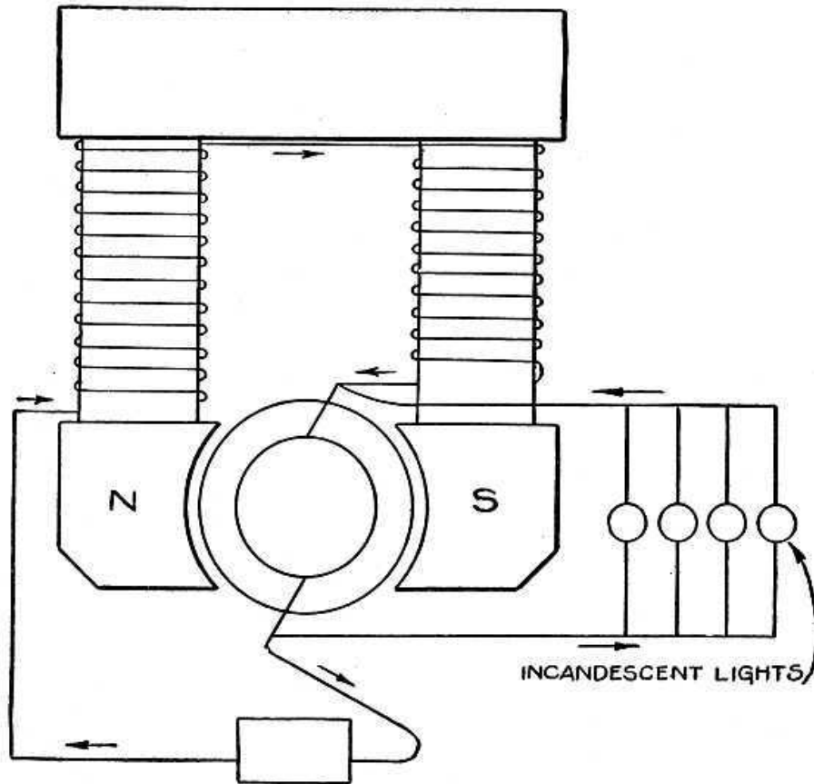
FIG. 50—A SHUNT-WOUND DYNAMO
