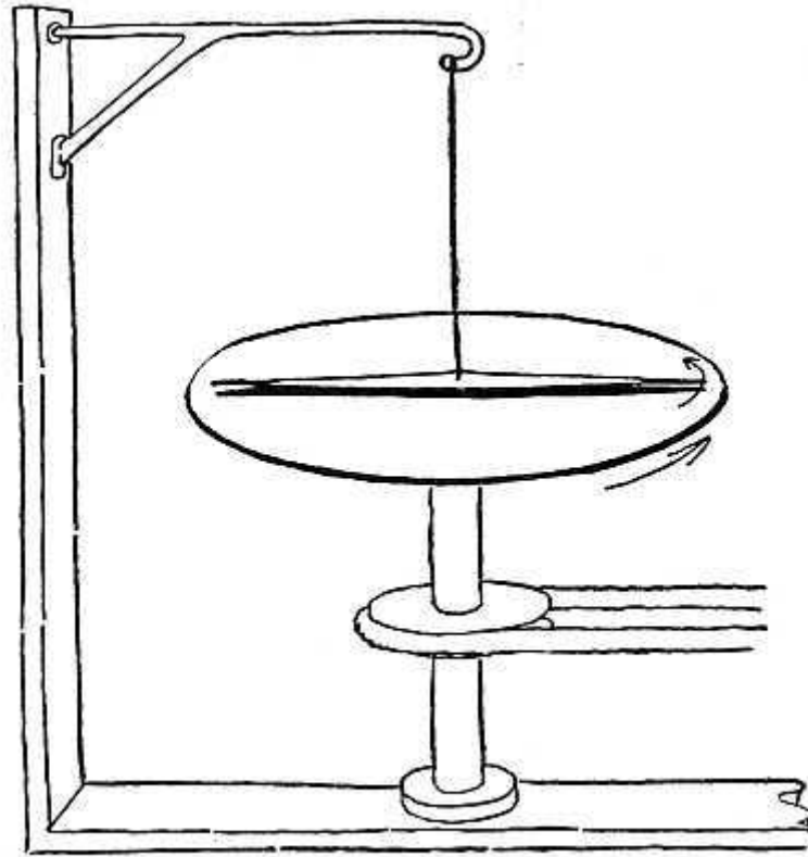
FIG. 26—ARAGO'S EXPERIMENT
