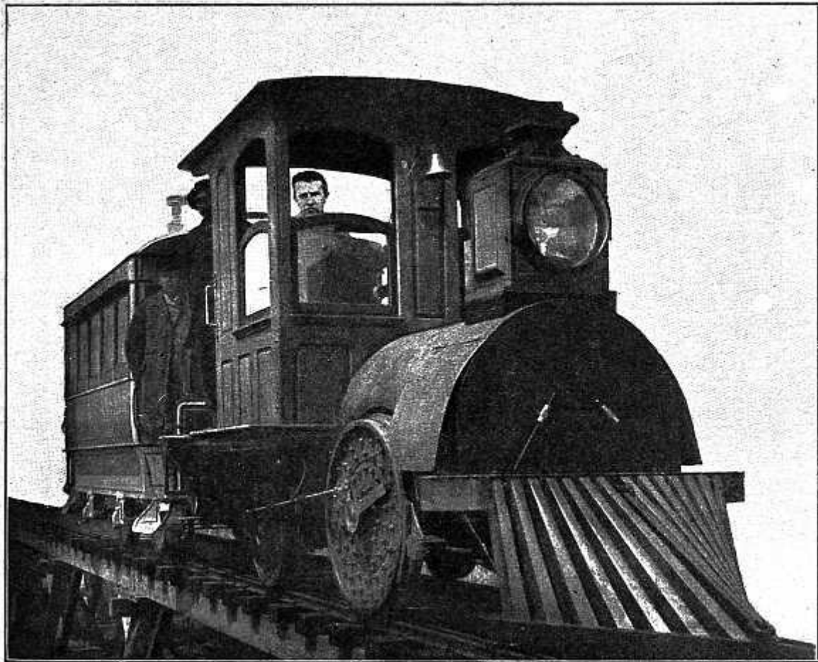
FIG. 56—EDISON'S FIRST PASSENGER LOCOMOTIVE
