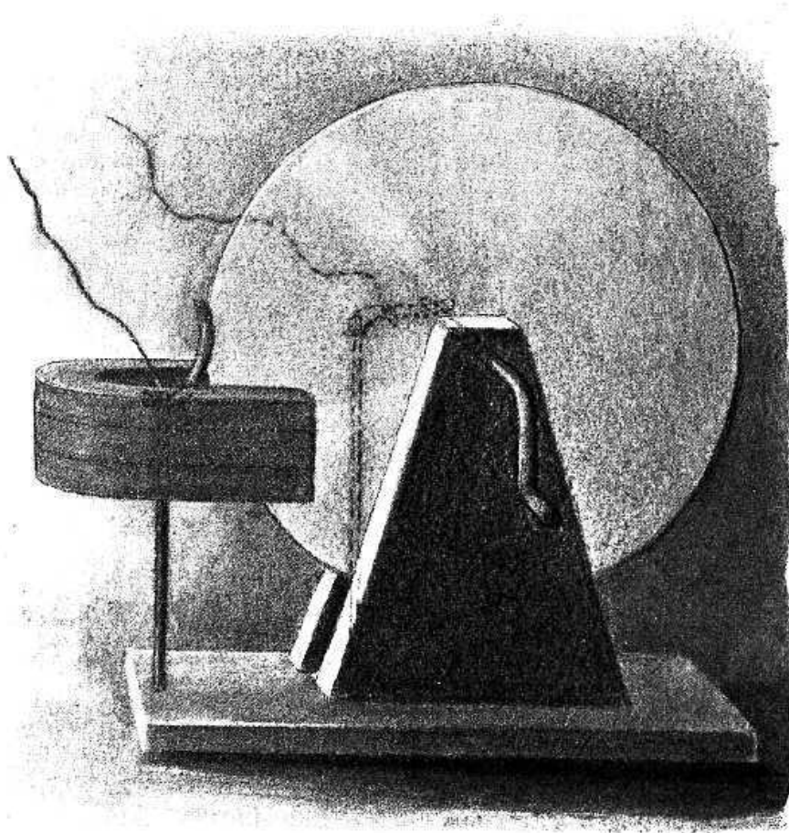
FIG. 32—FARADAY'S FIRST DYNAMO
