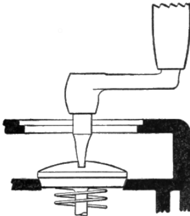
Fig. 30. Valve Grinding.
