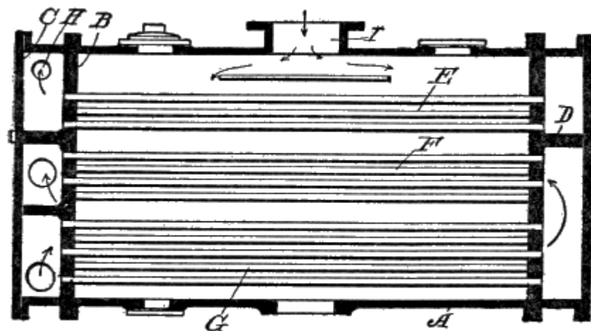
Fig. 71. Feed Water Heater.
