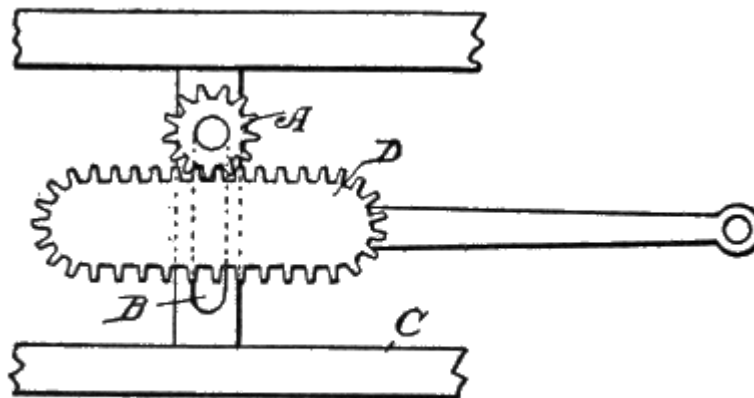
Fig. 109. Crank Motion Substitute.
