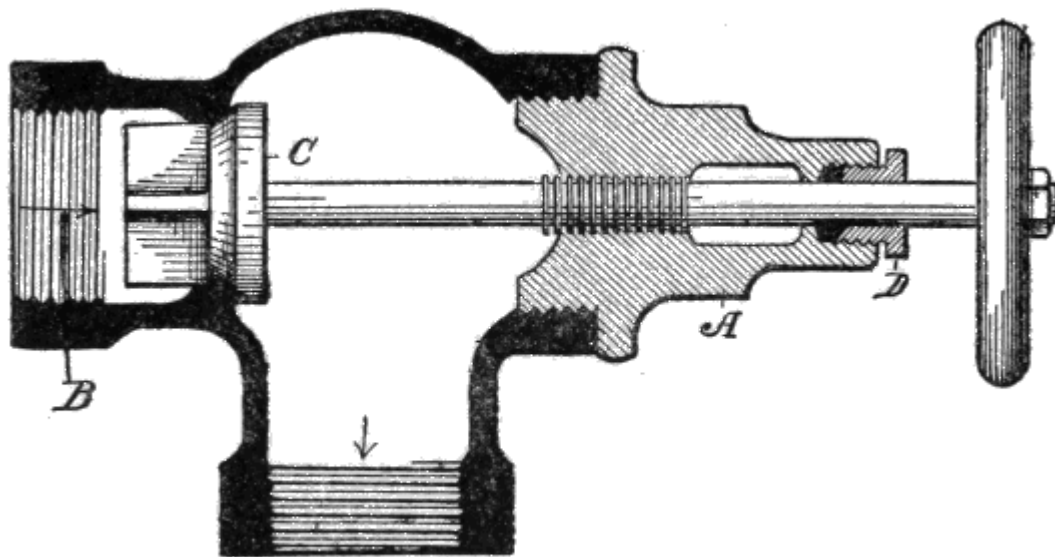
Fig. 77. Angle Valve.
