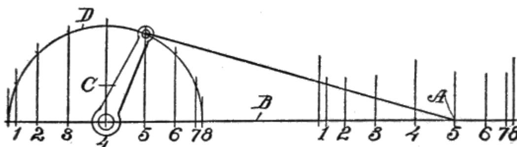
Fig. 107. Illustrating Crank-pin Movement.
