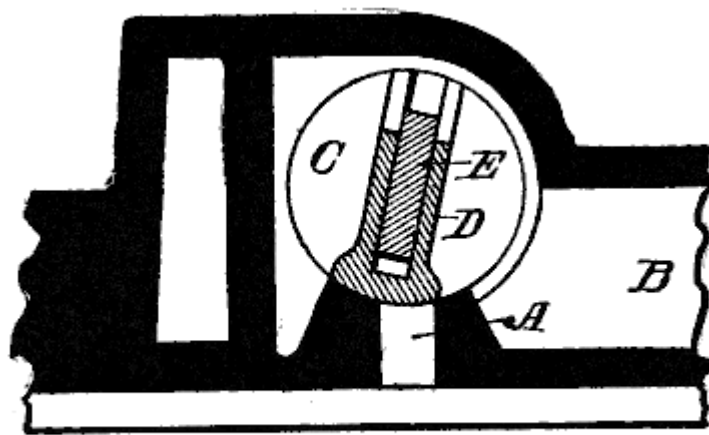
Fig. 75. Corliss Valve.
