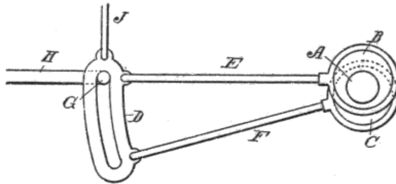
Fig. 61. Double Eccentric Reversing Gear.
