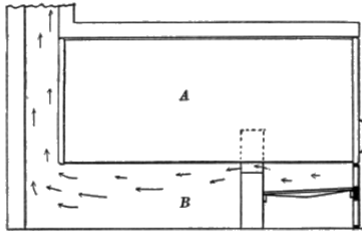
Fig. 3. Primitive Boiler
