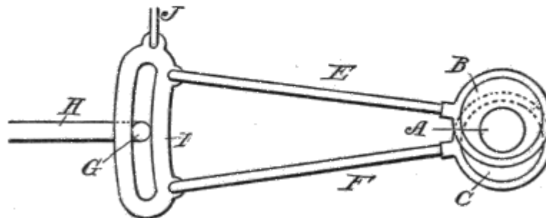
Fig. 62. Reversing Gear, Neutral.
