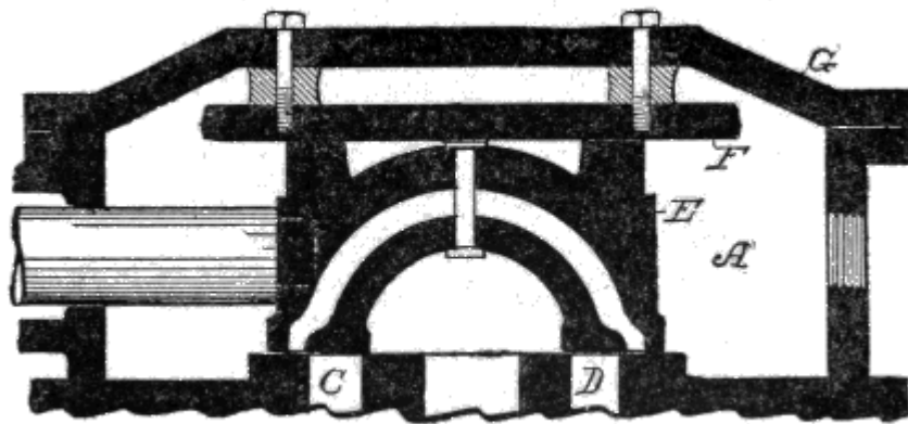
Fig. 65. Balanced Slide Valve.
