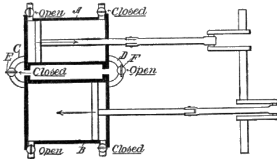
Fig. 16. Compound Engine.
