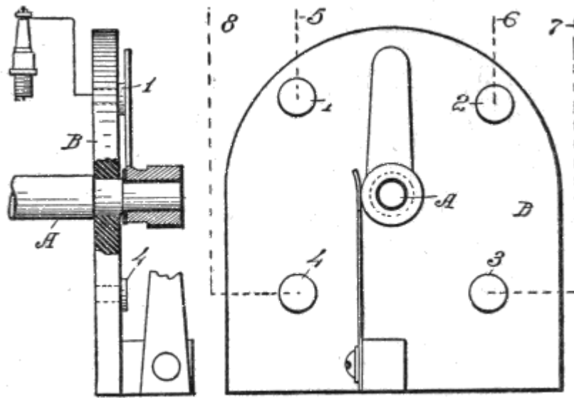
Fig. 57. The Distributer.
