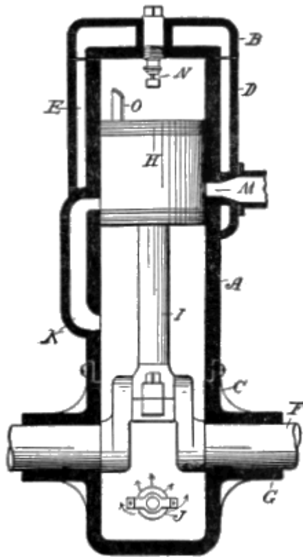
Fig. 23. Two-cycle. First position.
