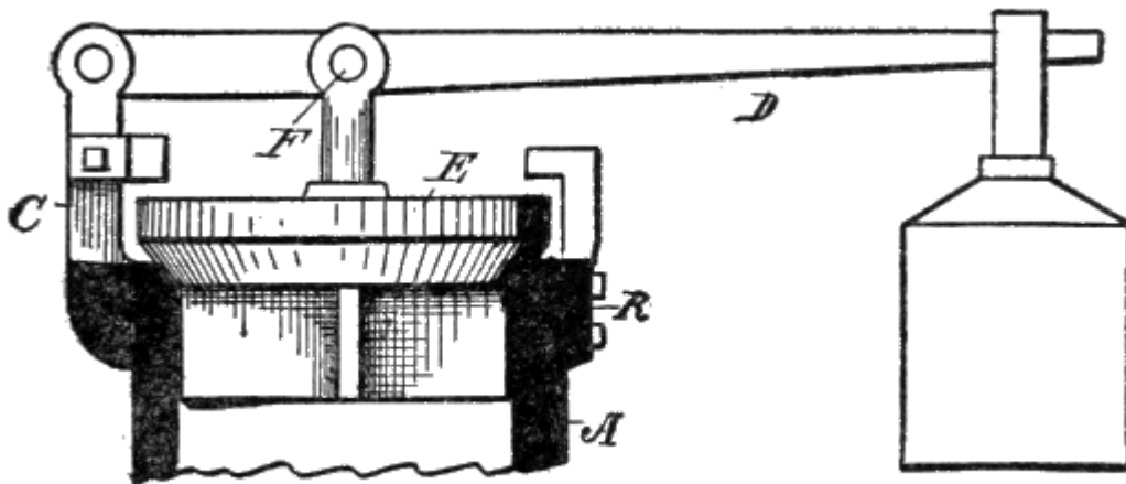
Fig. 86. Blow-off Valve.
