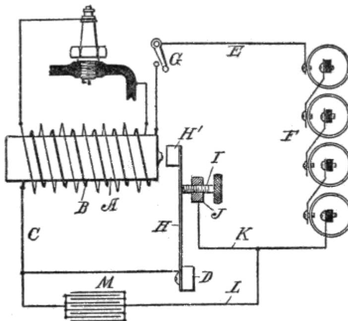
Fig. 56. Vibrator Coil and Connections.
