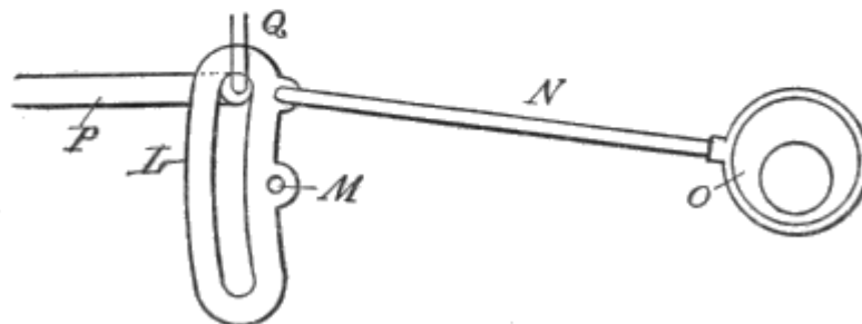
Fig. 64. Single Eccentric Reversing Gear.
