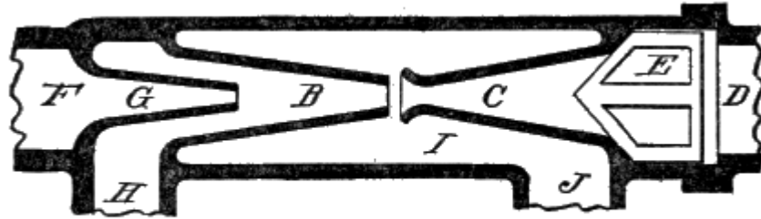
Fig. 69. The Original Injector.
