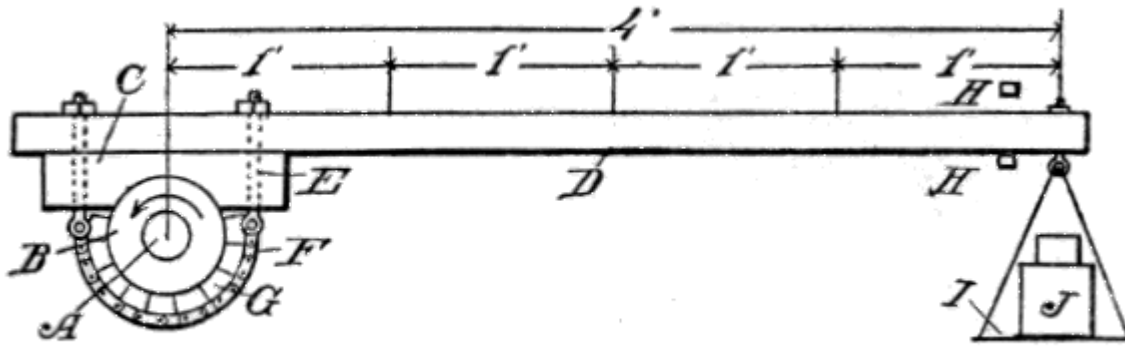
Fig. 60. The Prony Brake.
