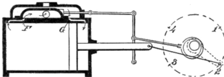
Fig. 12. Simple Valve Motion. Second position.
