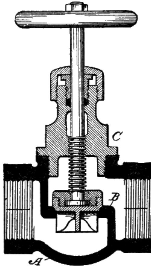
Fig. 74. Globe Valve
