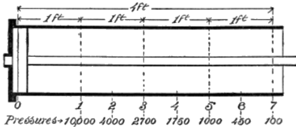
Fig. 13. Effective pressure in a Cylinder.
