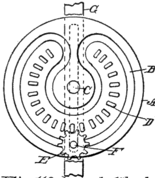
Fig. 110. mangle Wheel.
