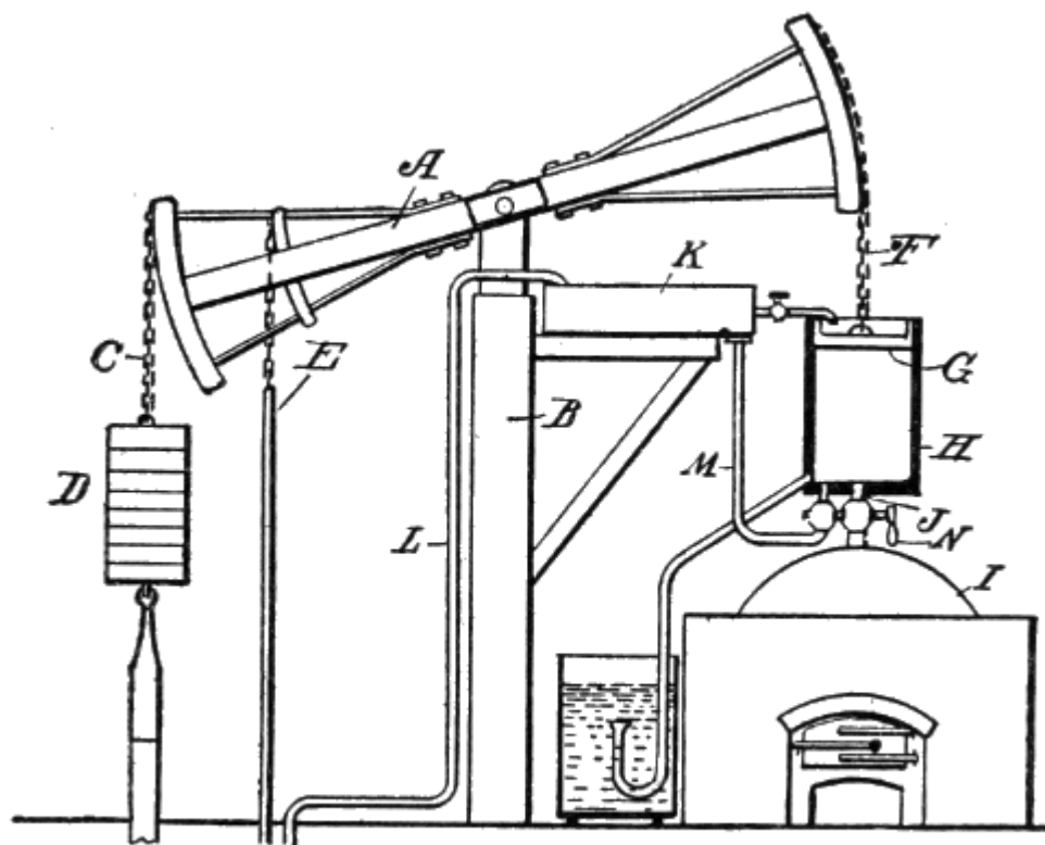
Fig. 10. Steam-Atmospheric Engine.
