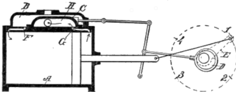
Fig. 11 Simple Valve Motion. First position.
