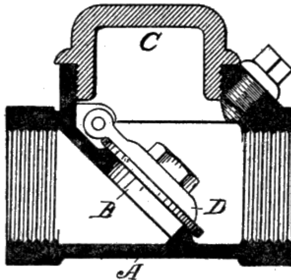
Fig. 72. Check Valve.
