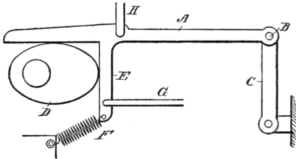
Fig. 97. Pivoted Follower for Cam.
