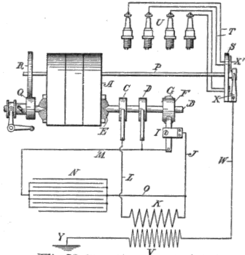
Fig. 58. Circuiting with Distributer
