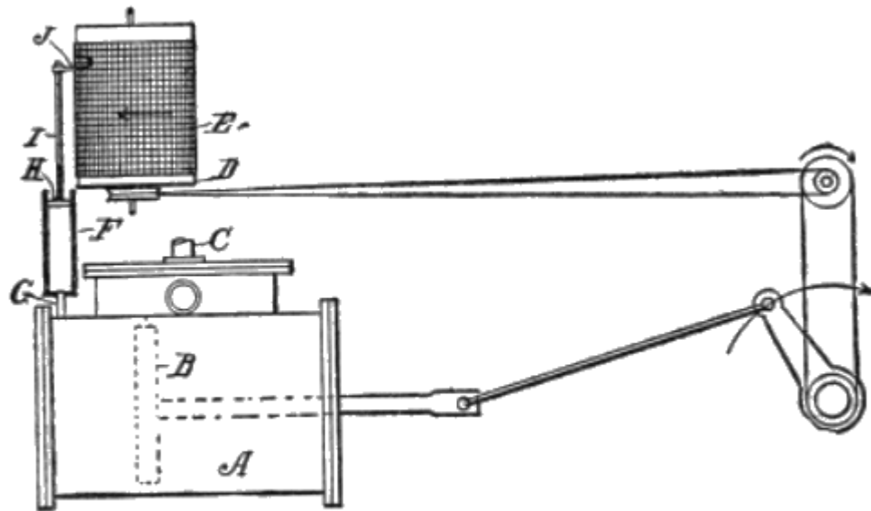
Fig. 15. Indicating the Engine.
