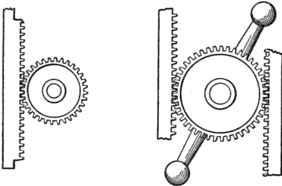
Fig. 101. Rack and Pinion. Fig. 102. Rack motion.
