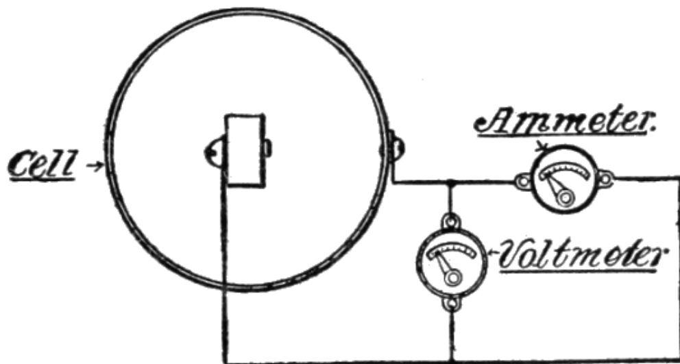
Fig. 38. Circuit Testing.
