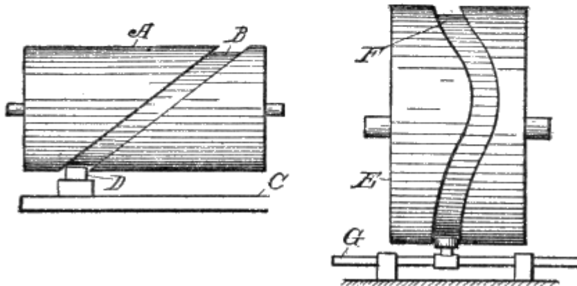
Fig. 95. Grooted Cam. Fig. 96. Reciprocating Motion.
