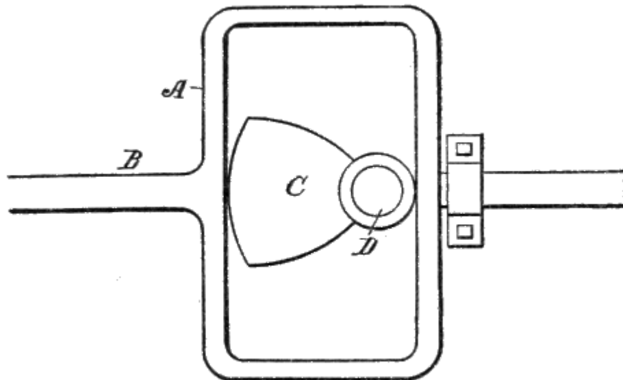
Fig. 100. Triangularly-formed Eccentric.
