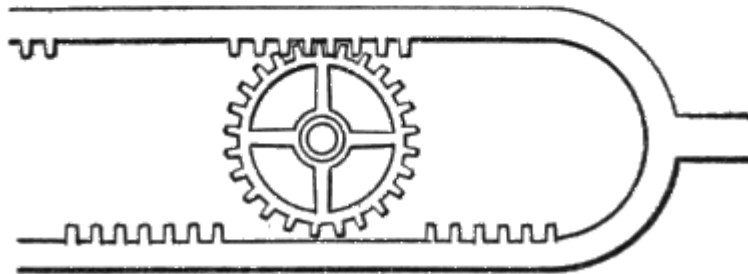
Fig. 105. Alternate Circular Motion.
