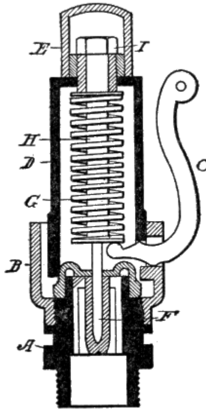
Fig. 87. Safety Pop Valve.
