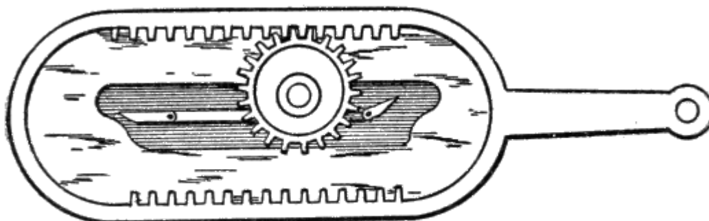
Fig. 106. Controlling Pinion for Mangle Rack.
