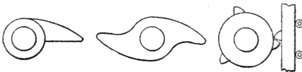
Fig. 91. Single Wiper. Fig. 92. Double Wiper. Fig. 93. Tilting Cam.
