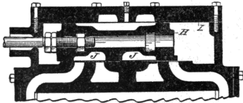
Fig. 66. Valve Chest. Double Port Exhaust.
