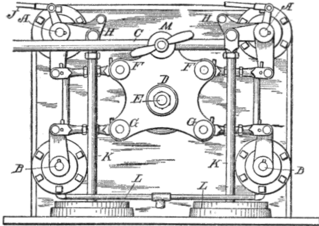
Fig. 76. Corliss Valve-operating mechanism.
