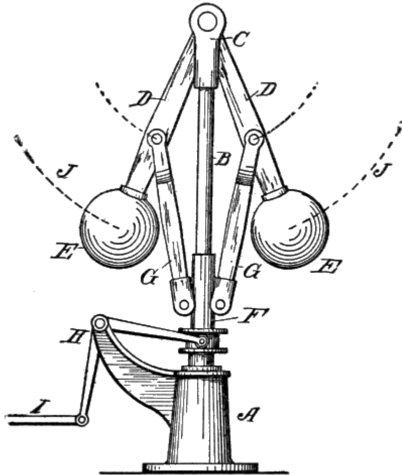
Fig. 68. Watt's Governor.
