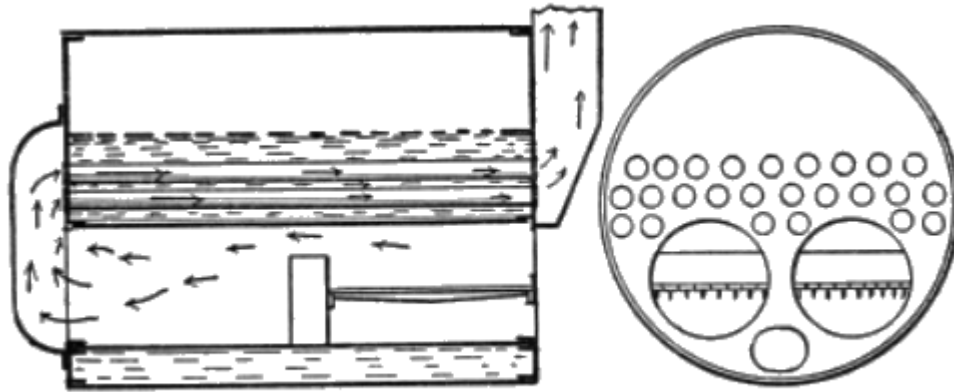
Fig. 5. Cornish, or Scotch Boiler.
