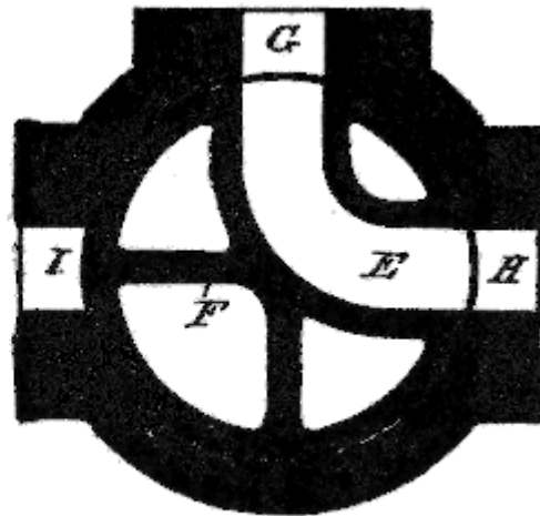
Fig. 79. Two-way Rotary
