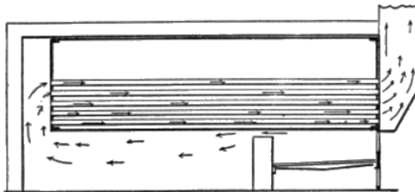
Fig. 4. Return Tubular Boiler
