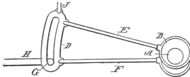
Fig. 63. Reversing Gear: Reversed.
