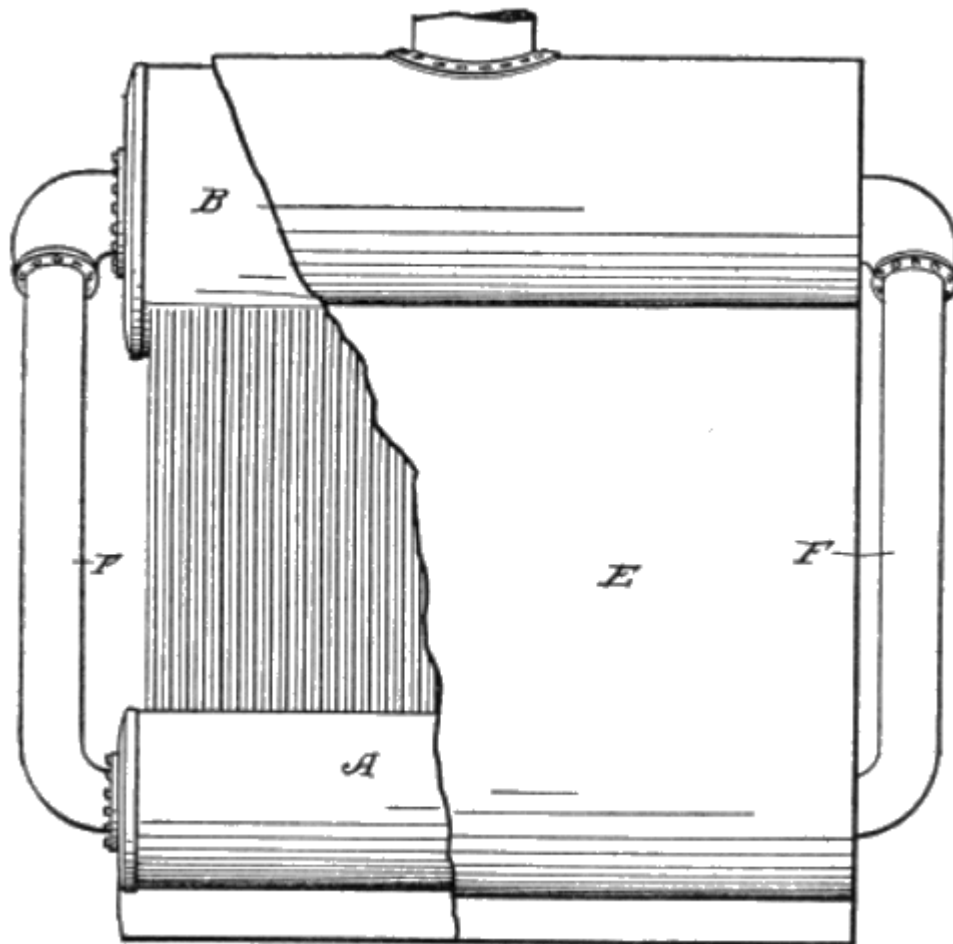
Fig. 7. Water Tube Boiler: Side View
