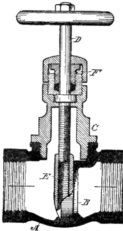
Fig. 73. Gate Valve.
