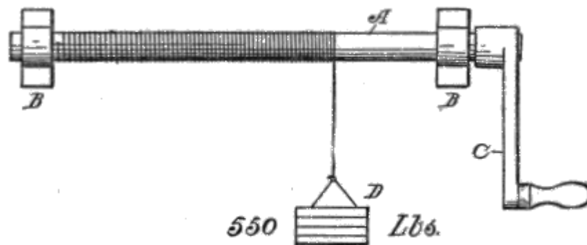
Fig. 59. Illustrating the Unit of Time.
