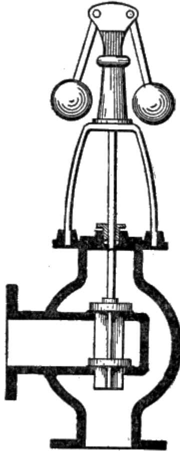
Fig. 67. Balanced Throttle Valve.
