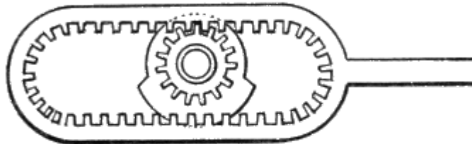
Fig. 104. Mangle Rack Motion.
