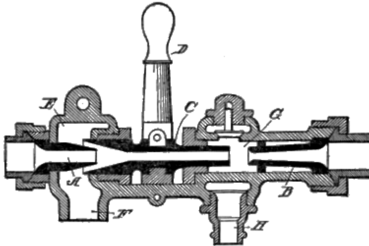
Fig. 70. Injector with Movable Combining Tube
