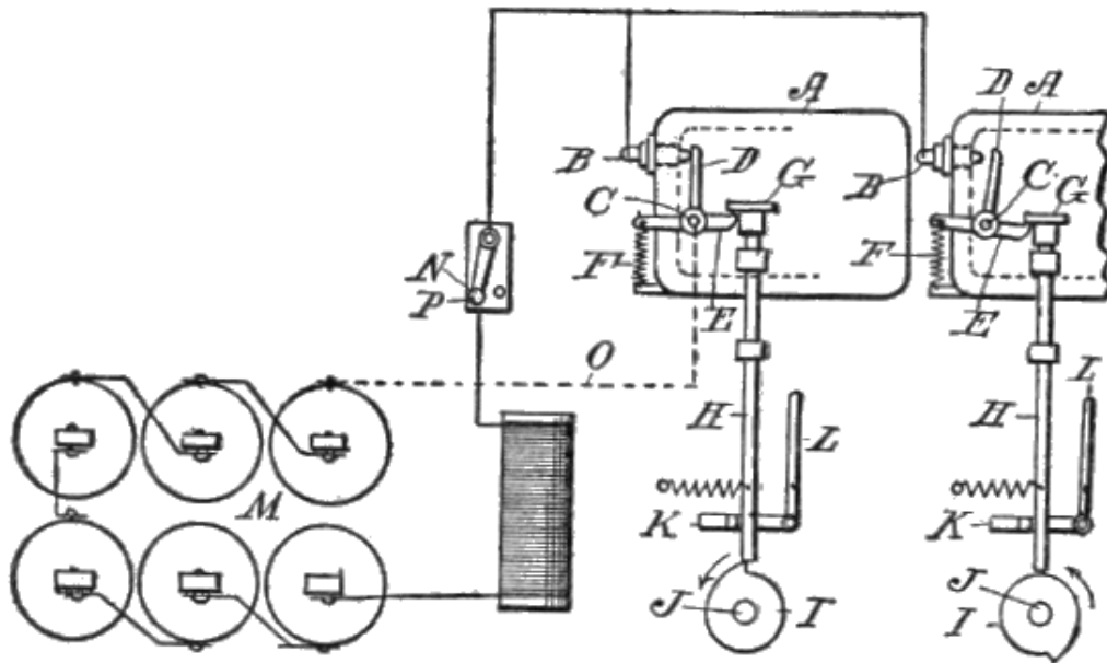
Fig. 39. Make and Break . with Battery.
