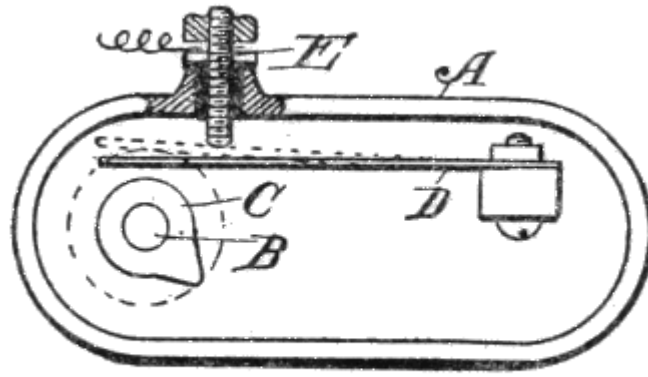
Fig. 52. Contact maker.
