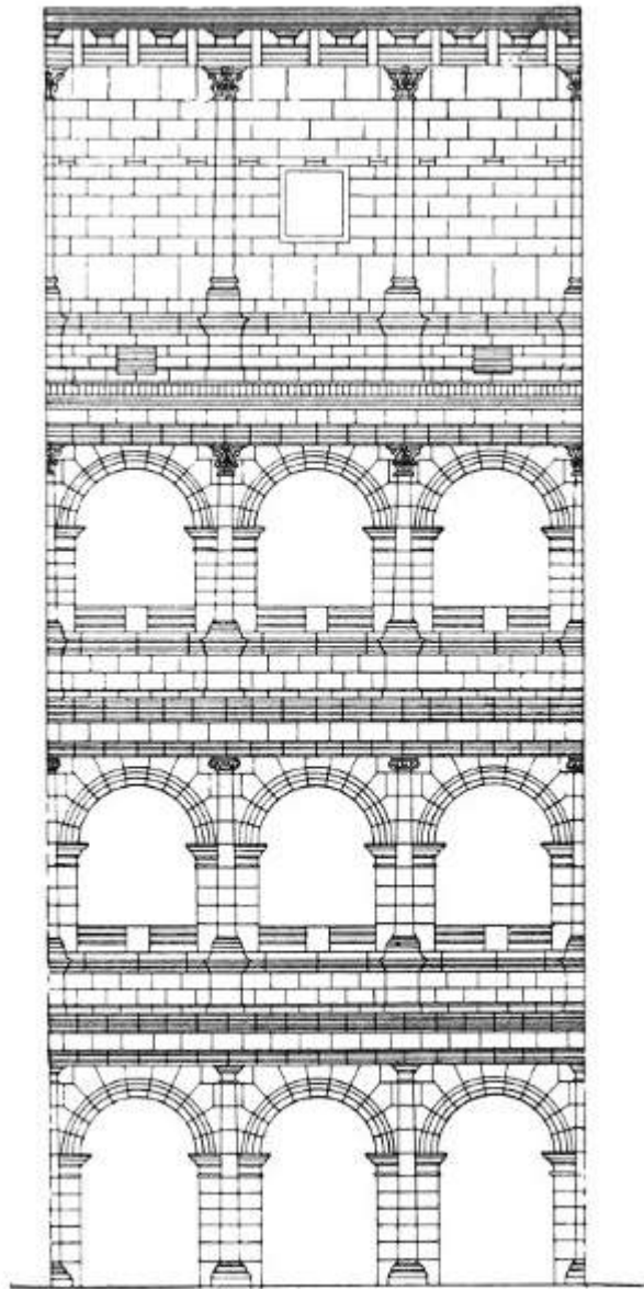
CONSTRUCTIVE & DECORATIVE USE OF ROUND ARCH & PILASTER FLAVIAN AMPHITHEATRE (COLOSSEUM) ROME.
