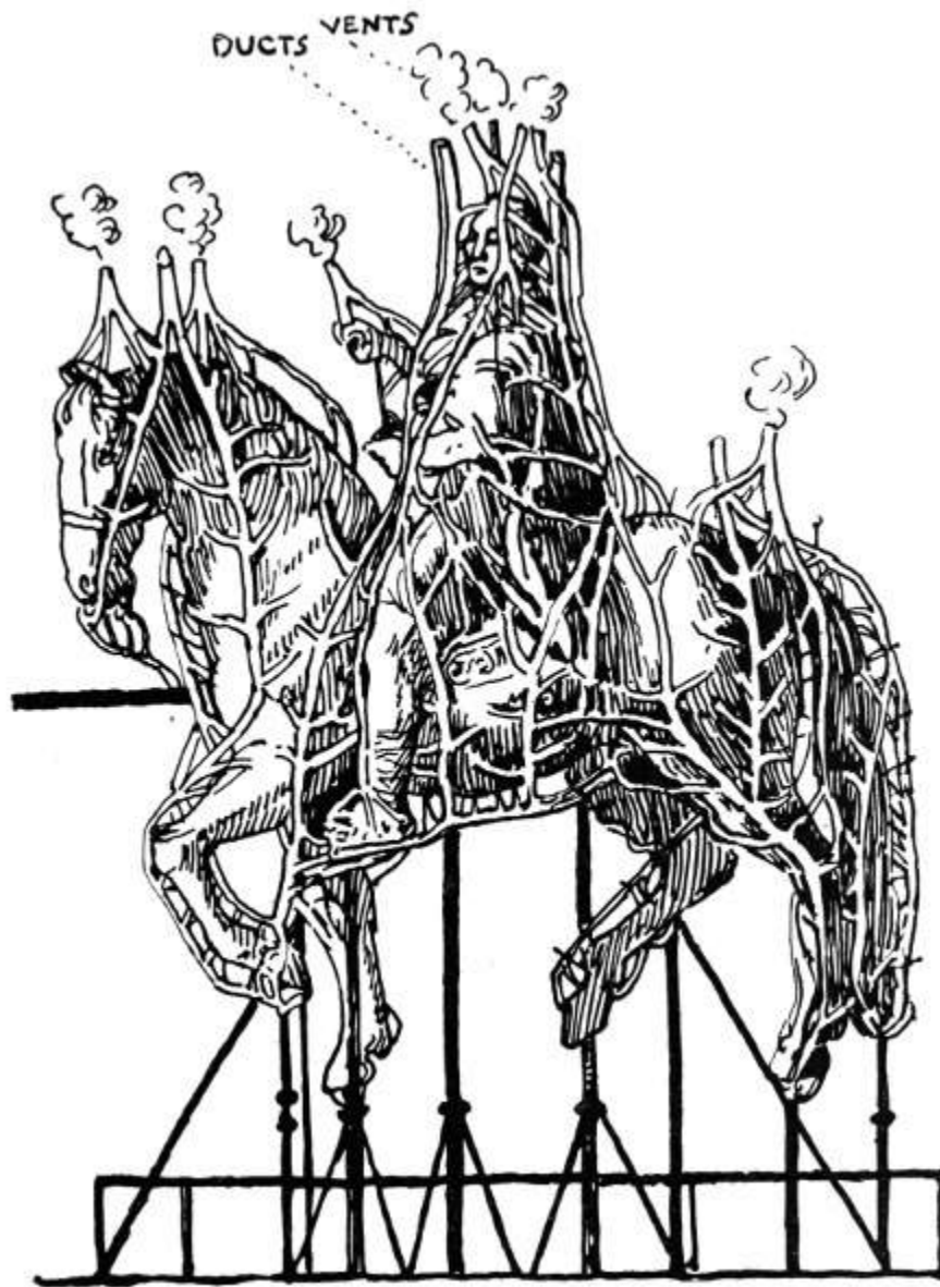
BRONZE STATUE OF LOUIS XV. BY BOUCHARDON, SHOWING DISTRIBUTION OF DUCTS AND VENTS. 4
