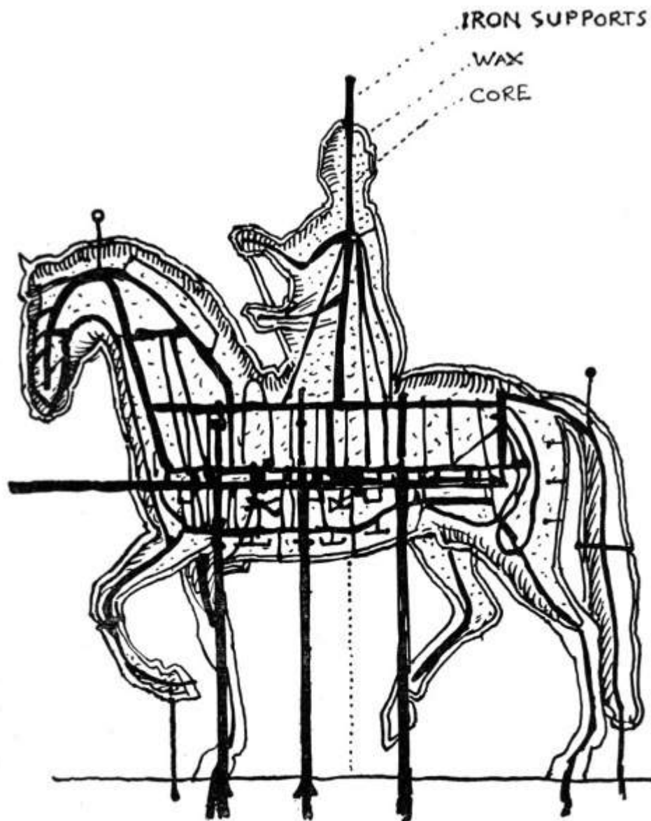
BRONZE STATUE OF LOUIS XV. BY BOUCHARDON, SHOWING INTERNAL IRON-WORK AND CORE. 3
