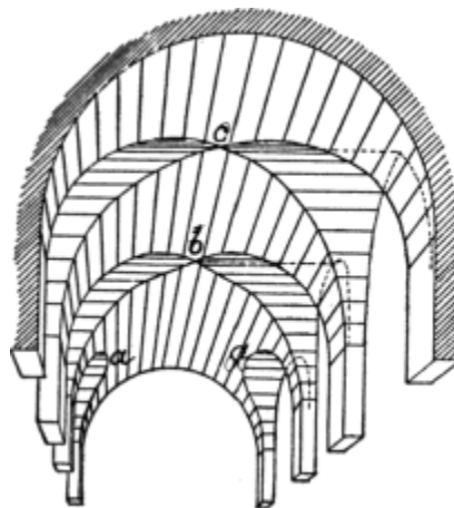
FIG. 109.—PENETRATIONS AND INTERSECTIONS OF VAULTS.
