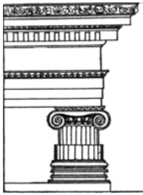
FIG. 28.—GREEK IONIC ORDER. (MILETUS.)
