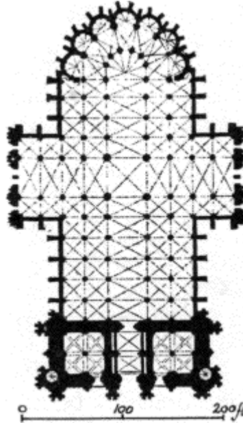
FIG. 141.—COLOGNE CATHEDRAL. PLAN.
