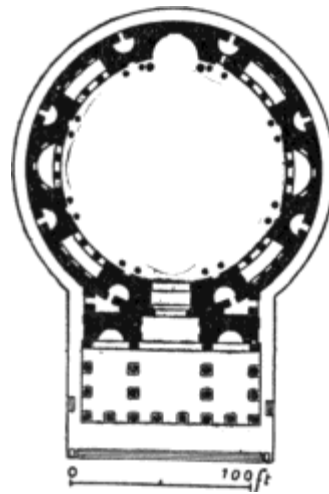
FIG. 54.—PLAN OF THE PANTHEON.
