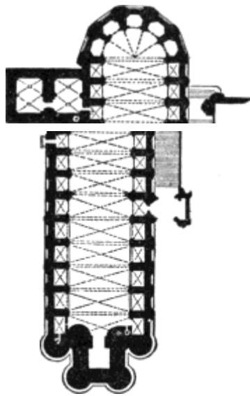
FIG. 123.—PLAN OF CATHEDRAL OF ALBY.
