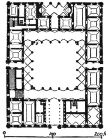
FIG. 167.—PLAN OF FARNESE PALACE.
