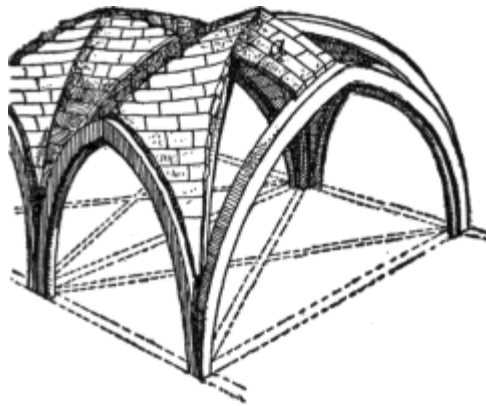
FIG. 119.—GROINED VAULT WITH ZIG-ZAG RIDGE-JOINTS.
