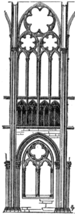
FIG. 120.—ONE BAY, ABBEY OF ST. DENIS.
