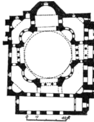
FIG. 74.—ST. SERGIUS, CONSTANTINOPLE.
